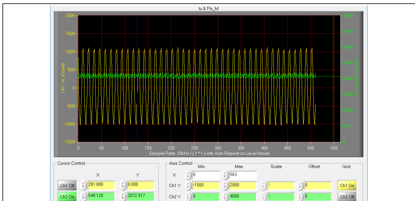
Figure 11 Trace waveform for lu & Flx-M at rate speed
