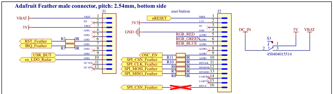
Figure 15: Schematic of Adafruit headers
