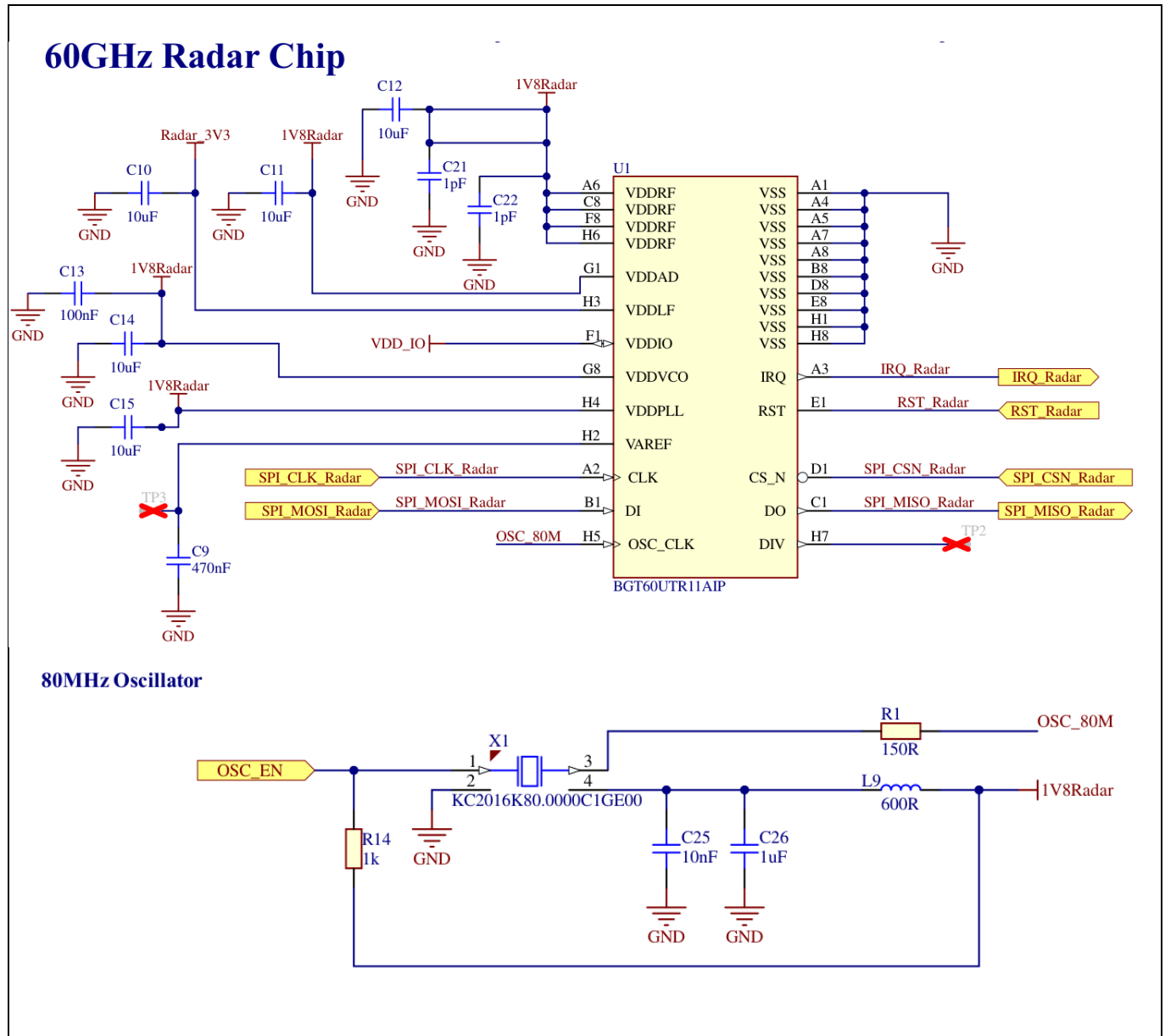
Figure 14: Schematic of XENSIV™ BGT60UTR11AIP radar with 80 MHz oscillator
