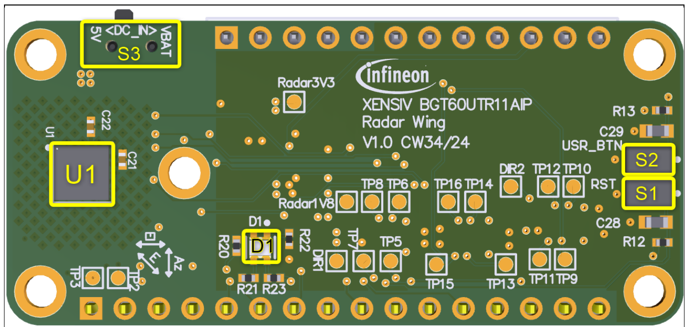
Figure 12: Front view of the BGT60UTR11 radar wing
