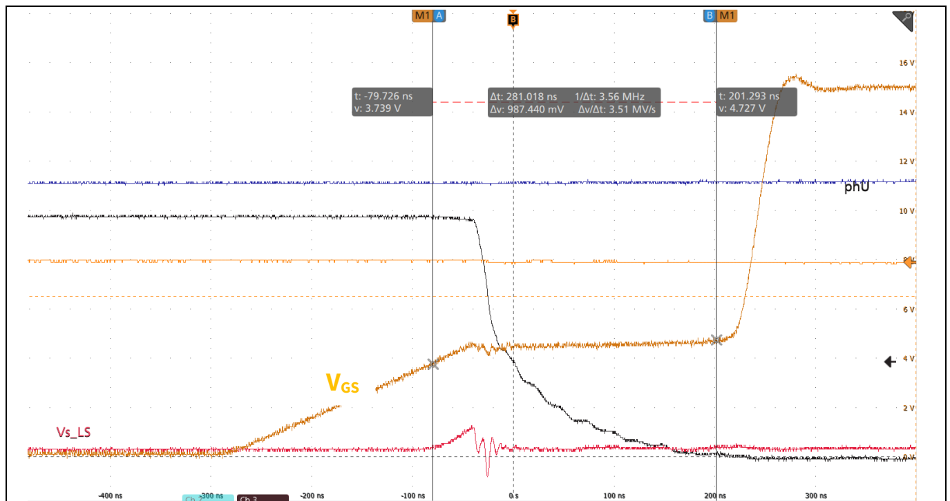
Figure 50 Gate charge (MOSFET turn-on), V_{GS} at I_u = 10 A, I_G = 40 mA, T_{ON} = 281 ns
