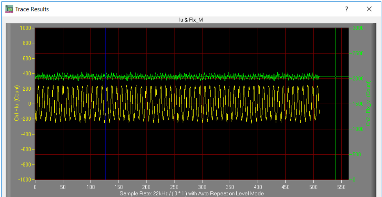
Figure 9 Trace waveform for lu & Flx-M at 50% Speed
