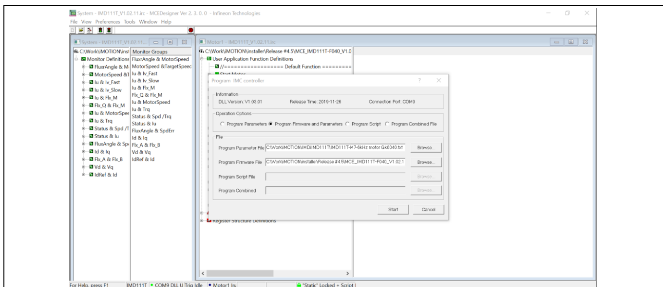
Figure 7 Programming window
