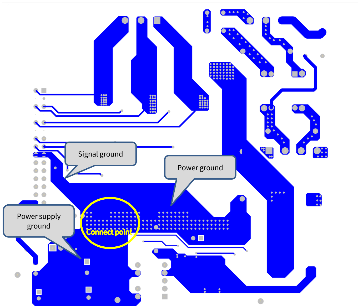
Figure 18 Bottom layer
