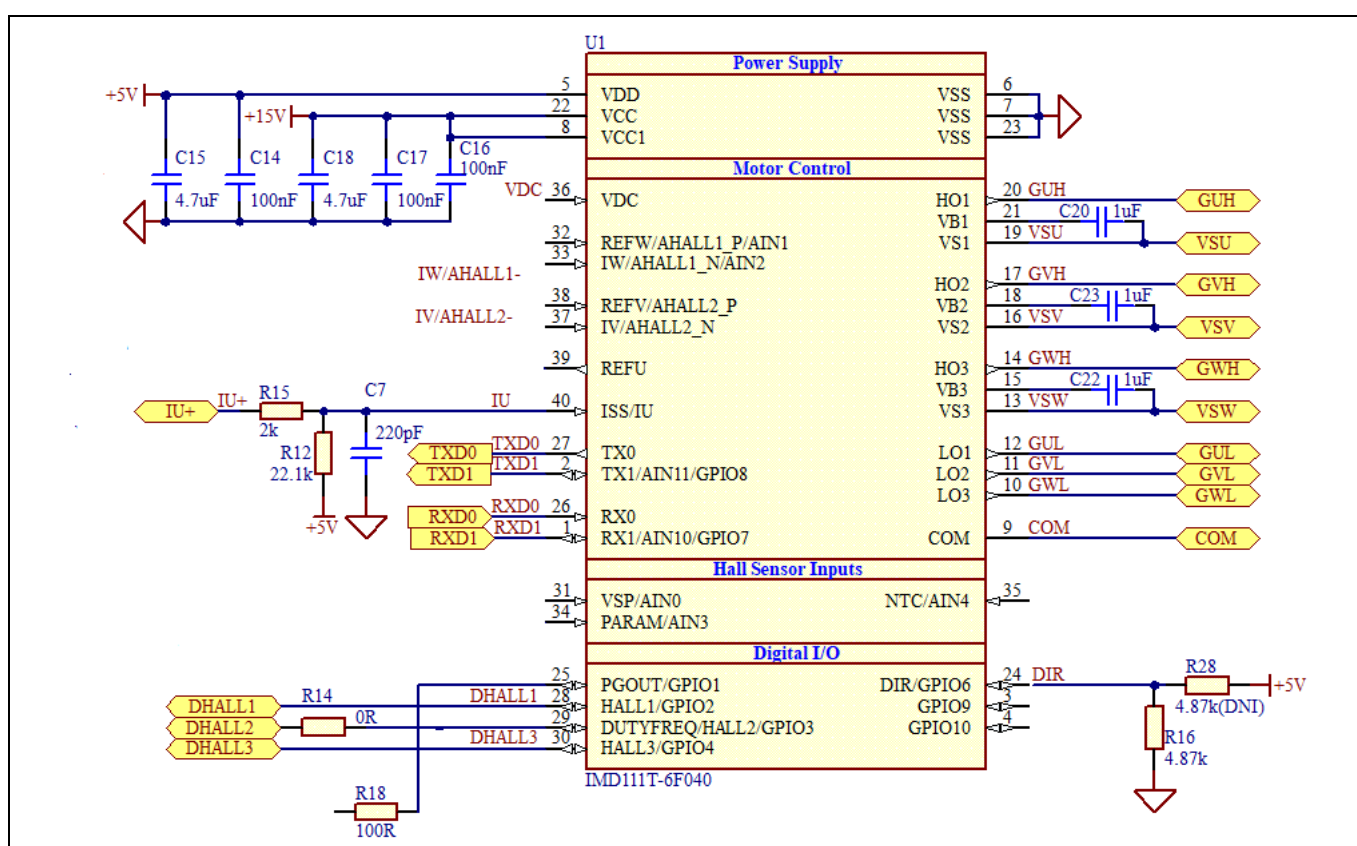
Figure 11 IMD111T schematics
