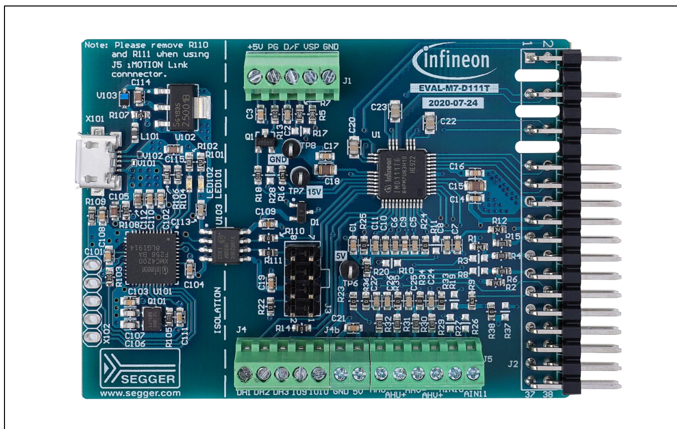
Figure 1 Evaluation board of EVAL-M7-IMD111T
