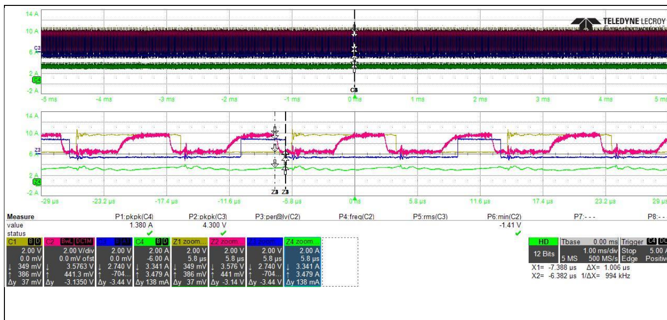
Figure 15 Synchronous rectification gate signal
