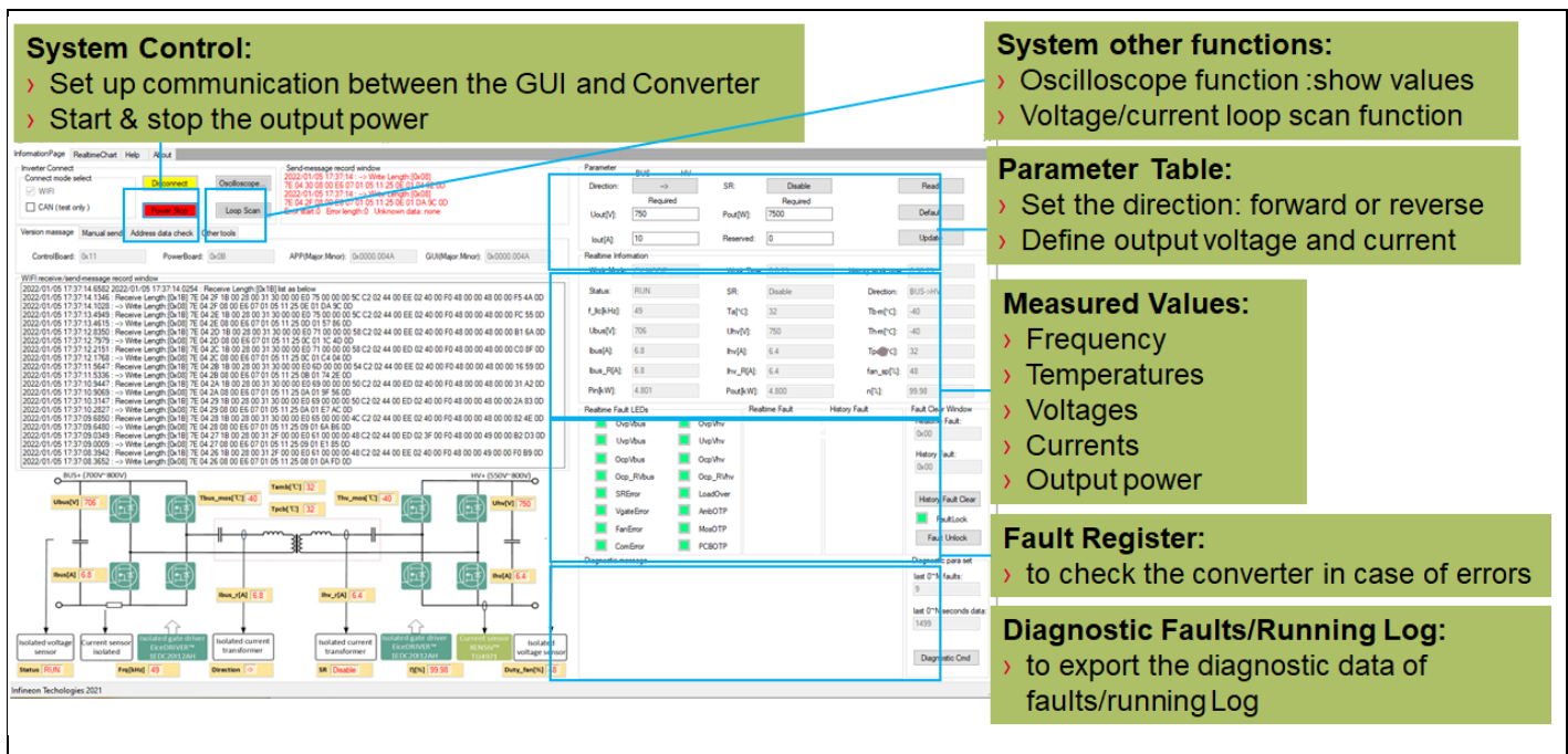
Figure 19 Graphical user interface (GUI)
