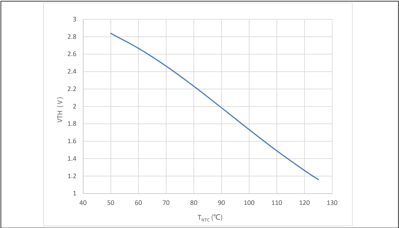
Figure 28 VTH output
