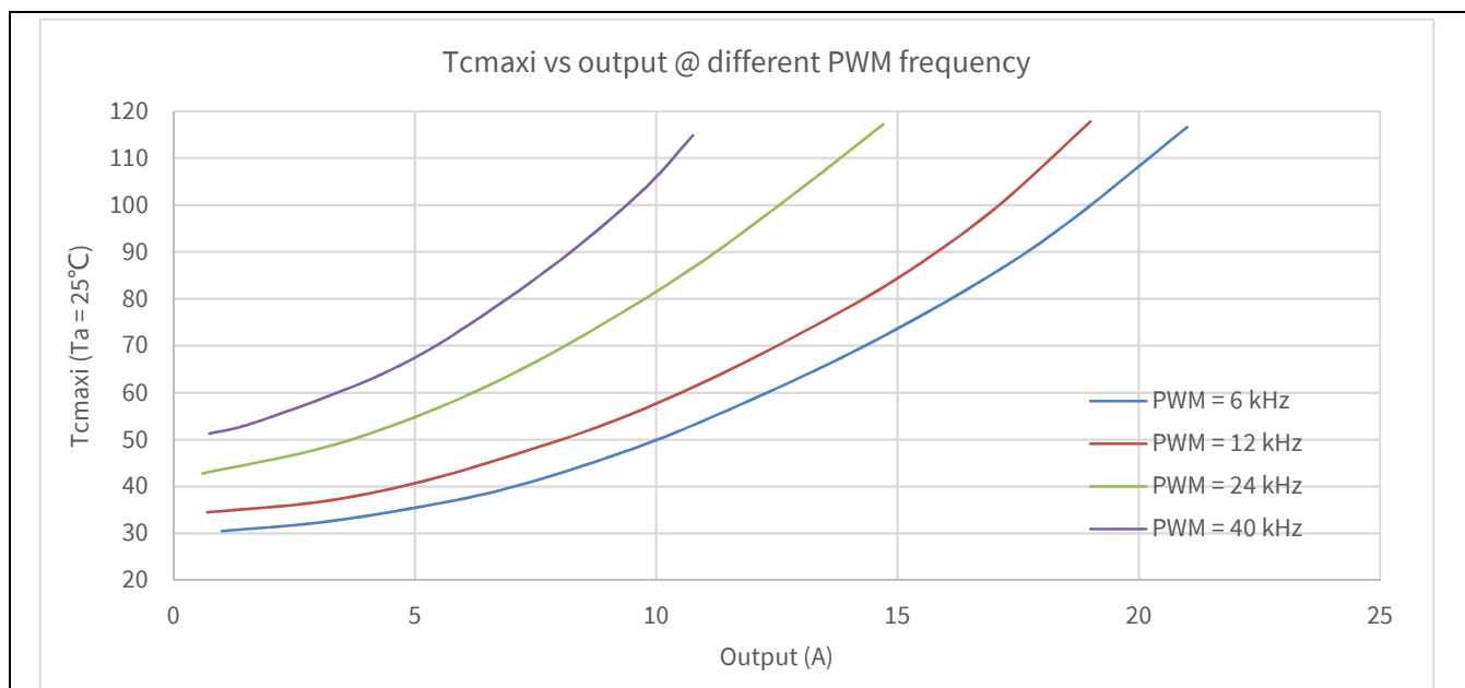
Figure 37 IM828-XCC case temperature vs output power current at different PWM frequencies @380 V AC input, T_a=25^\circ\text{C}
