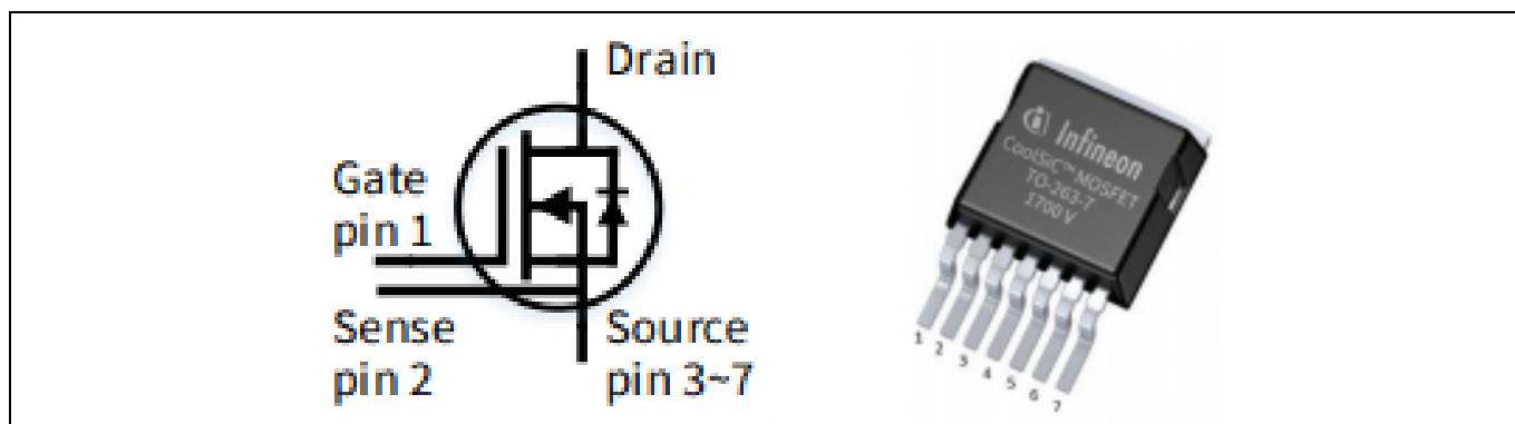
Figure 13 IMBF170R1K0M1 package: PG-TO263-7 and pin definition
