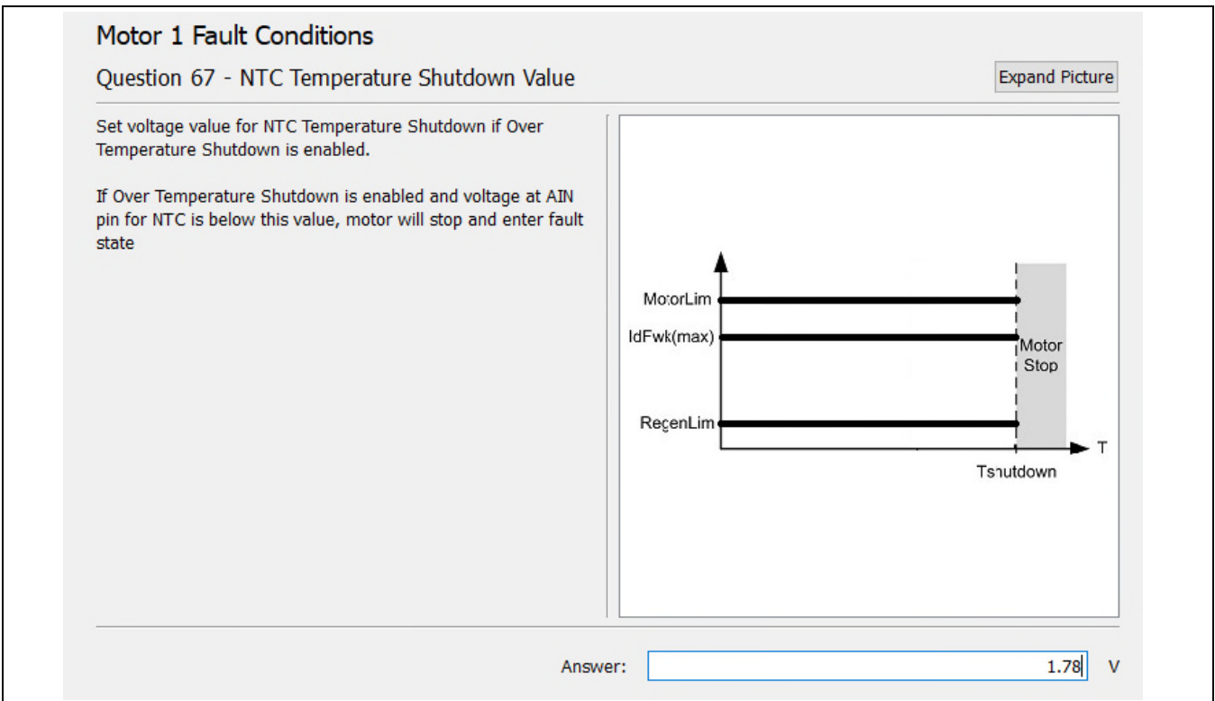
Figure 29 IPM temperature shutdown set to 100°C in MCEWizard
