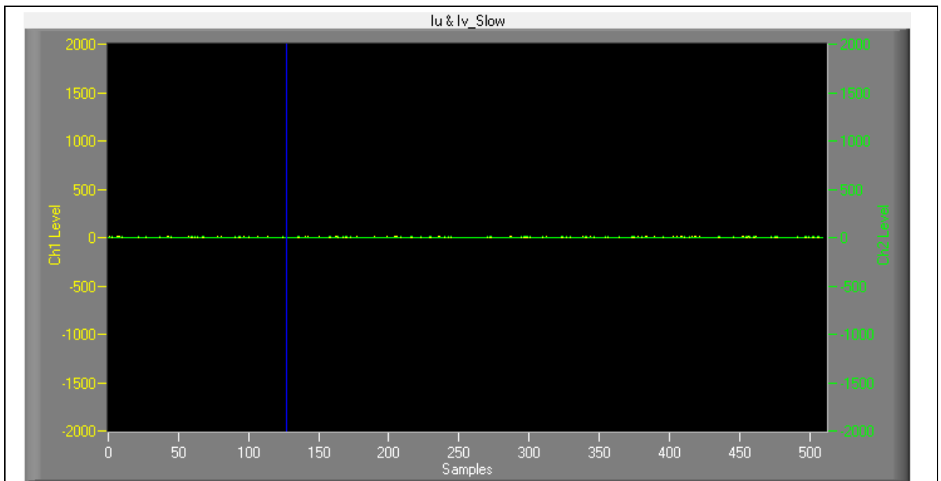
Figure 10 I_u and I_v static noise waveform from MCEDesigner
