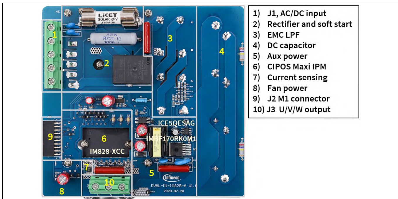
Figure 2 Functional groups of the EVAL-M1-IM828-A reference design
