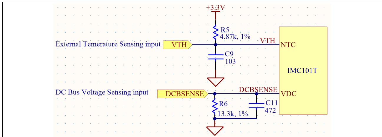
Figure 16 Analog inputs on the EVAL-M1-101TF evaluation board
