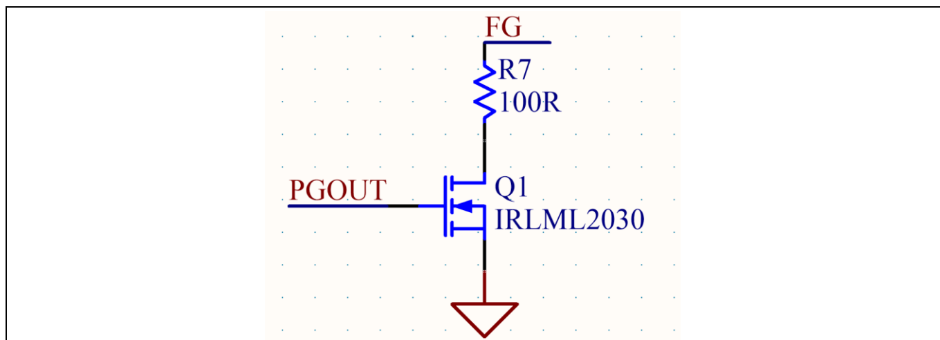
Figure 23 VSP Input Connector and level shift schematic for FG
