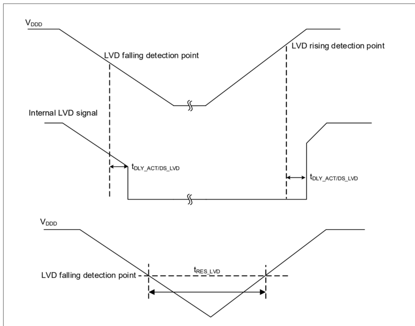
Figure 31 LVD specifications
