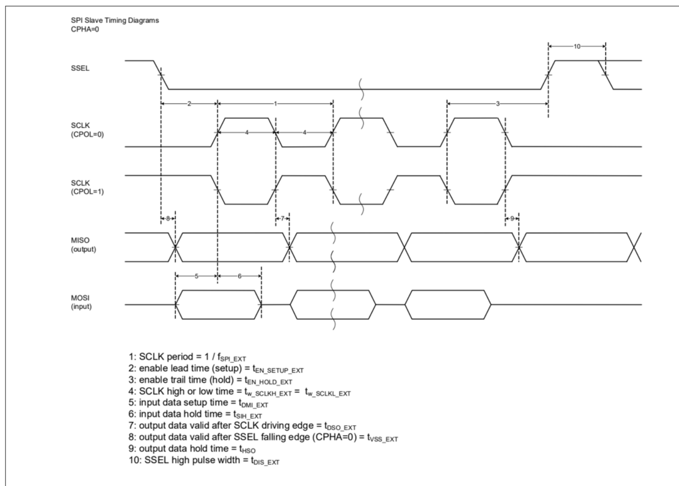
Figure 23 SPI slave timing diagrams with LOW clock phase
