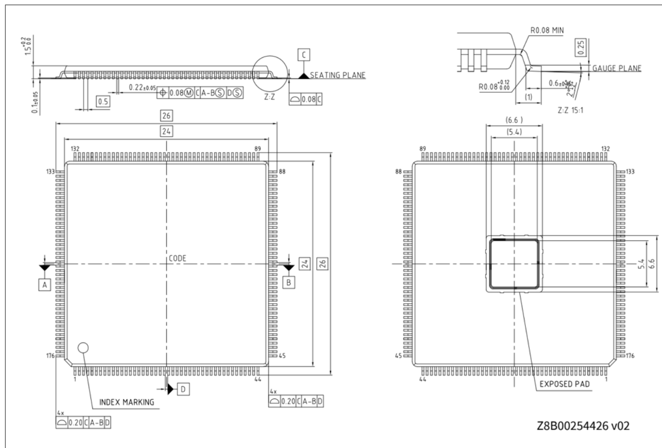
Figure 59 Package outline - 176-TEQFP
