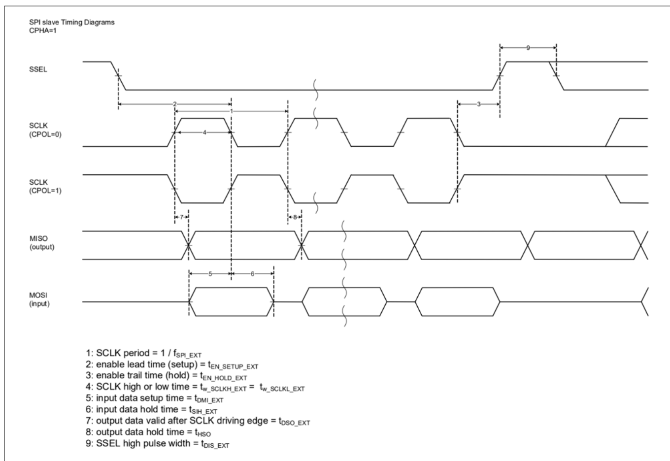
Figure 24 SPI slave timing diagrams with HIGH clock phase
