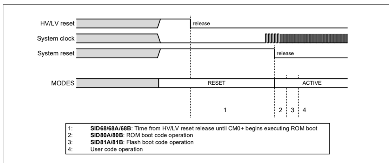
Figure 14 Reset sequence
