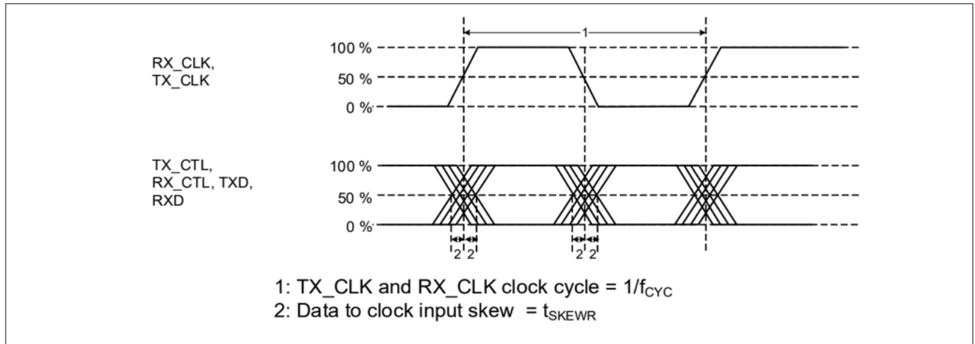
Figure 41 RGMII Rx timing diagram
