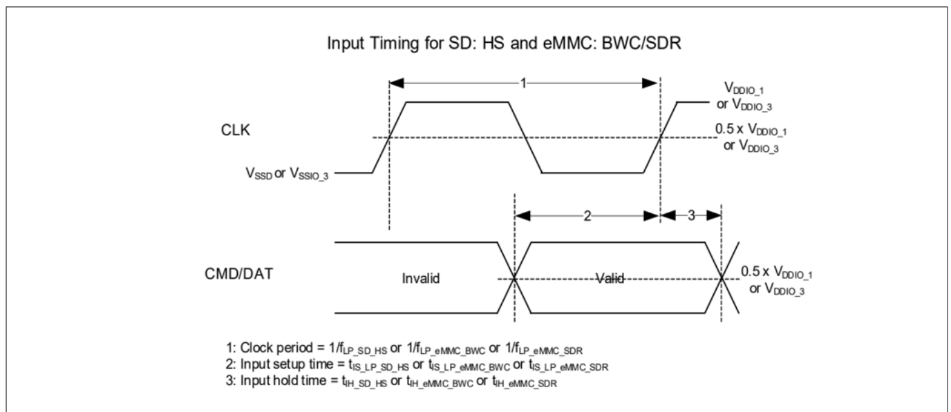
Figure 44 SD high-speed and eMMC BWC/SDR input timing
