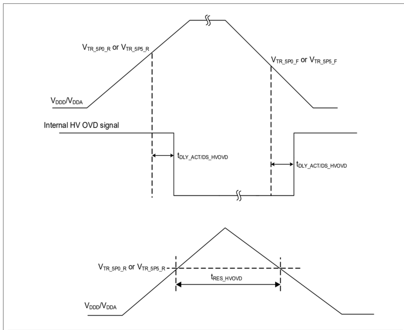
Figure 29 High-voltage OVD specifications
