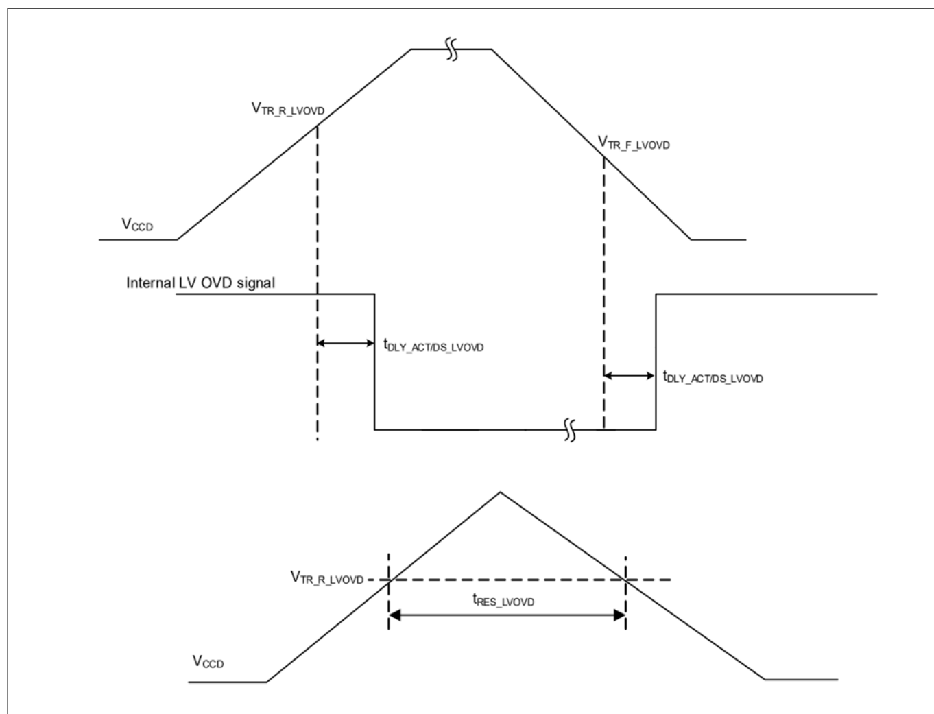
Figure 30 Low-voltage OVD specifications
