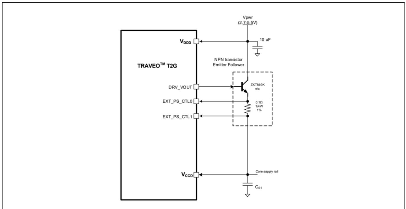
Figure 2 Sample core external regulator with NPN transistor
