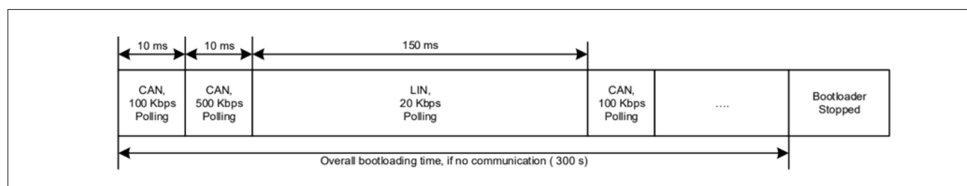
Figure 62 Bootloading sequence
