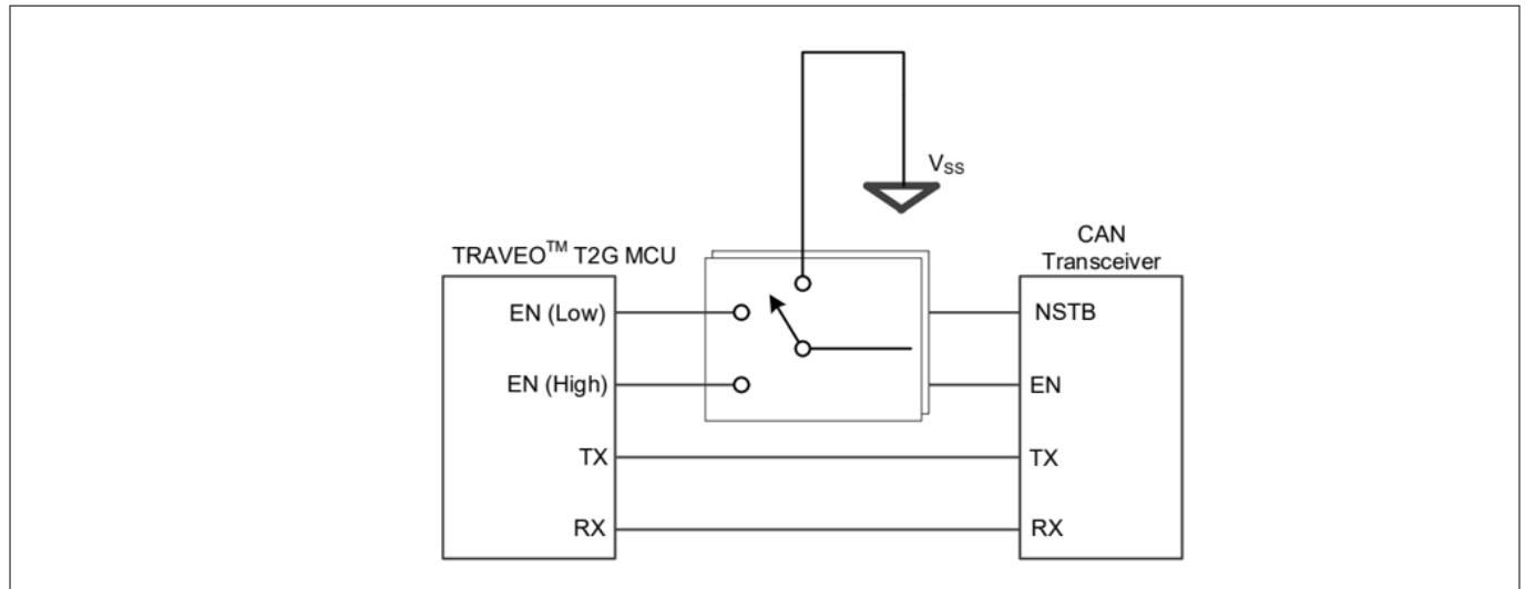
Figure 63 MCU to CAN transceiver connections
