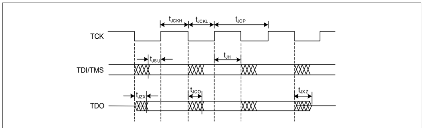
Figure 32 JTAG specifications
