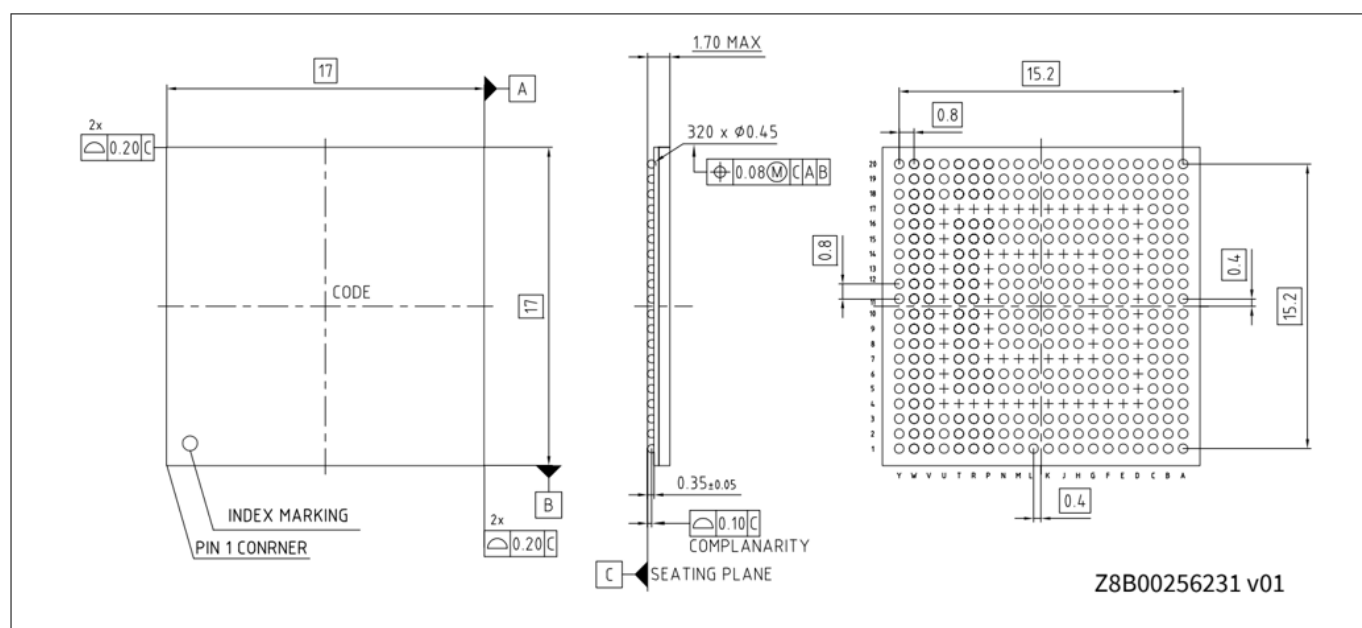
Figure 61 Package outline – 320-BGA
