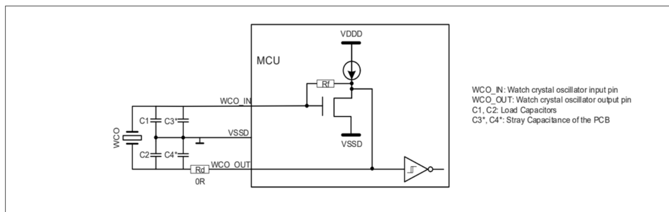
Figure 34 WCO connection scheme 19)
