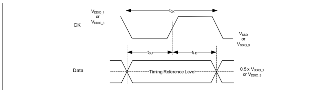
Figure 51 SDR write timing reference level
