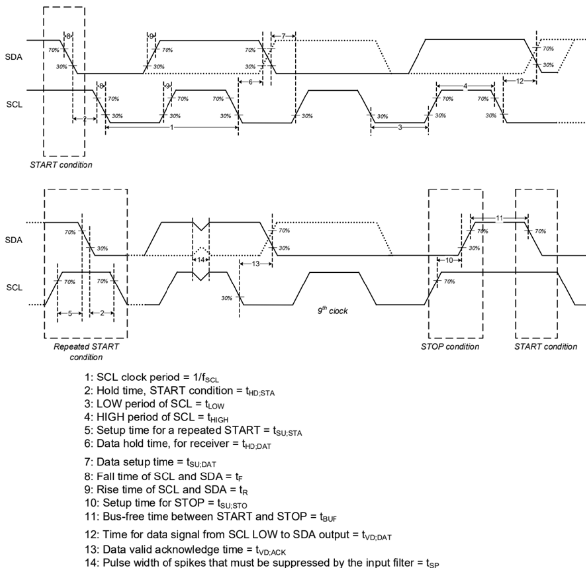
Figure 20 I2C timing diagrams
