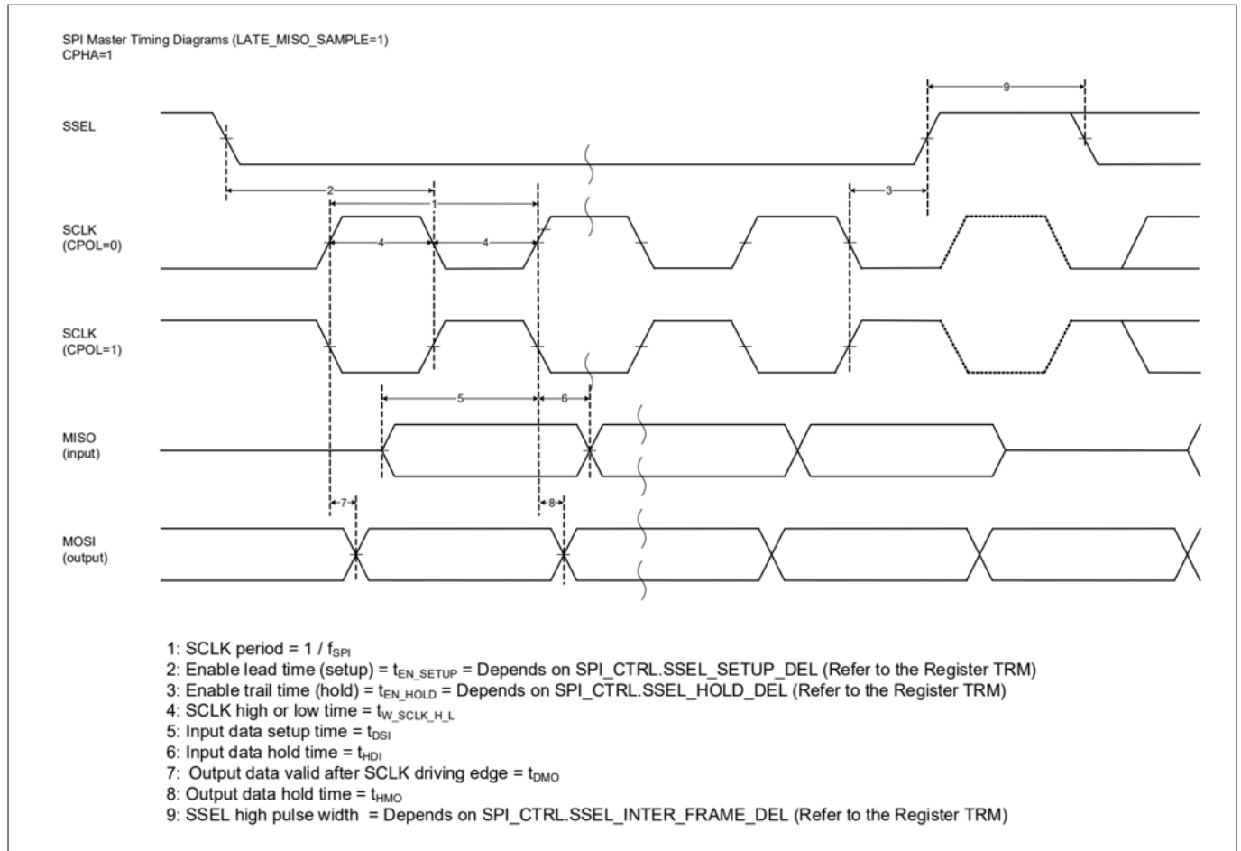
Figure 22 SPI master timing diagrams with HIGH clock phase
