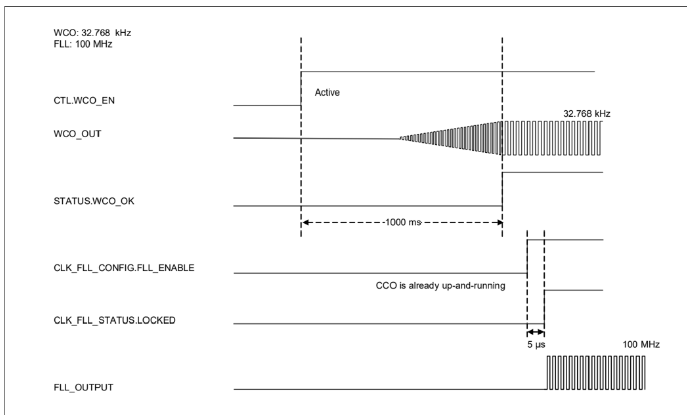
Figure 36 WCO to FLL diagram
