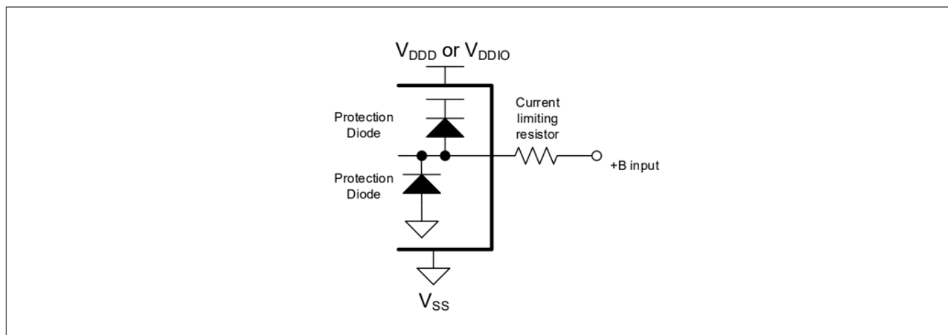
Figure 12 Example of a recommended circuit 17)
