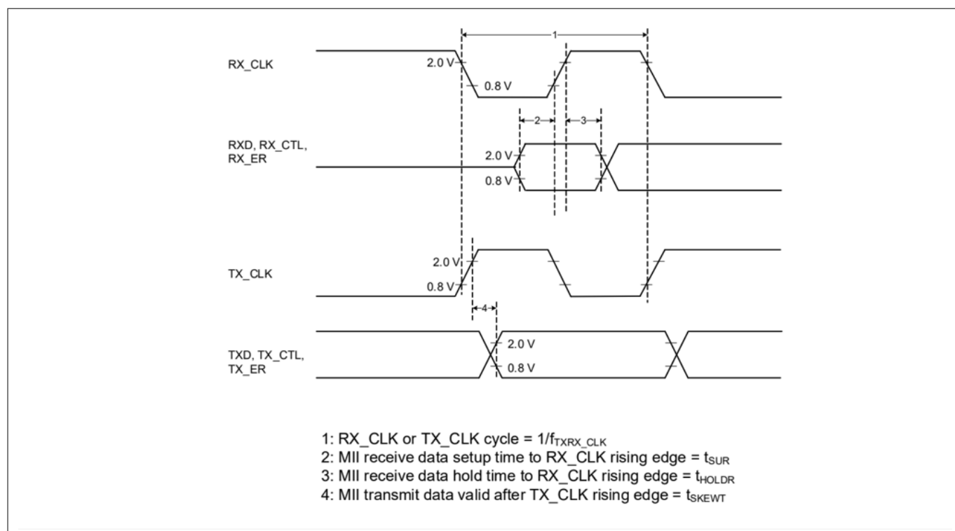
Figure 37 MII timing diagram
