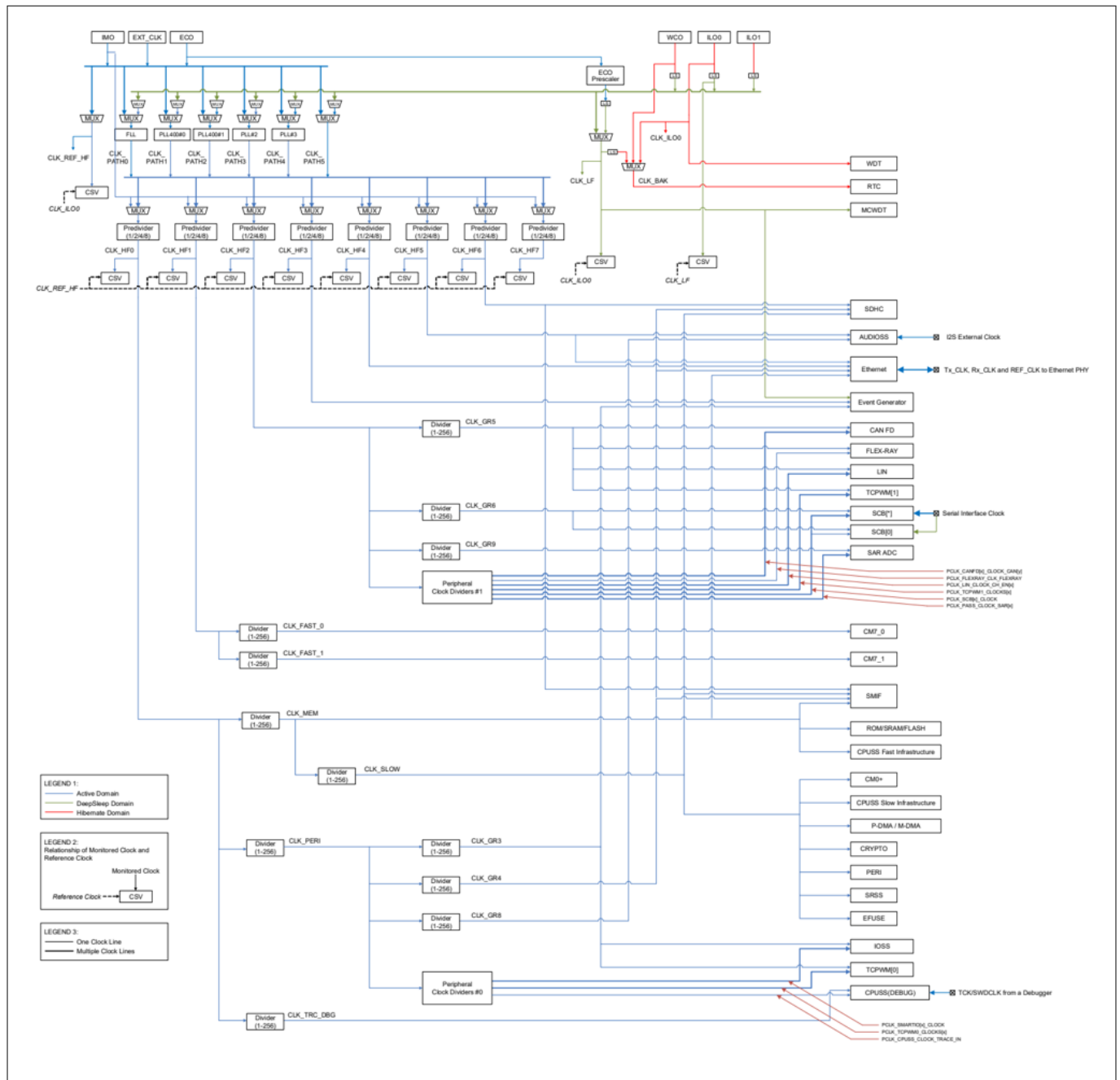
Figure 5 CYT4BF clock diagram
