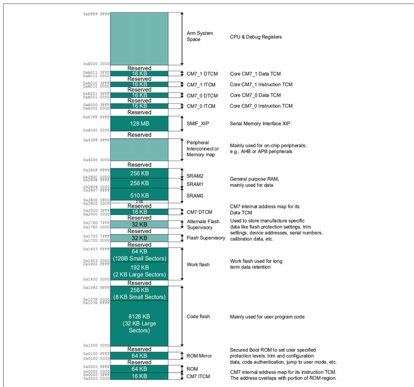
Figure 4 CYT4BF address map 12), 13)
