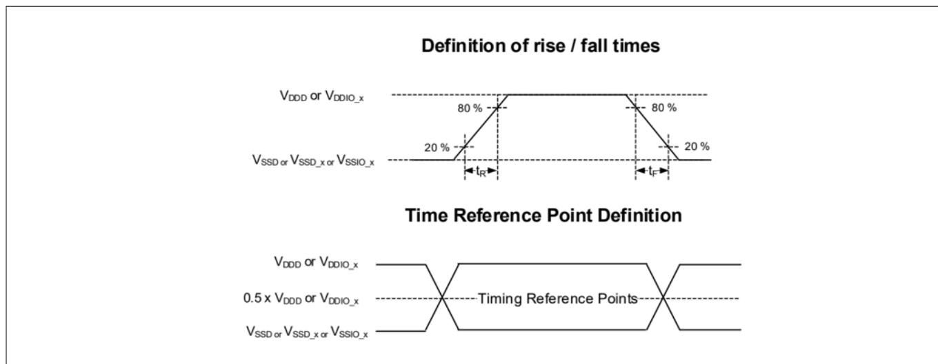
Figure 18 AC timings specifications
