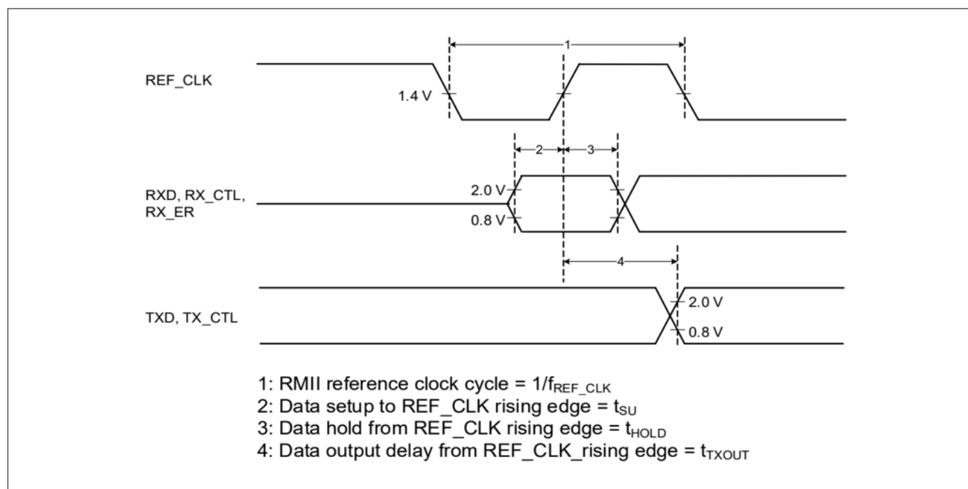
Figure 39 RMI timing diagram
