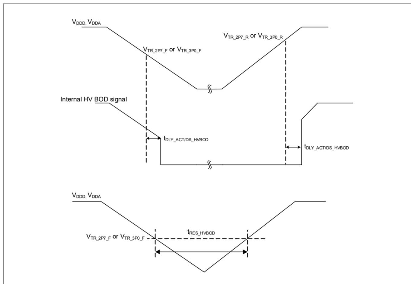
Figure 27 High-voltage BOD specifications
