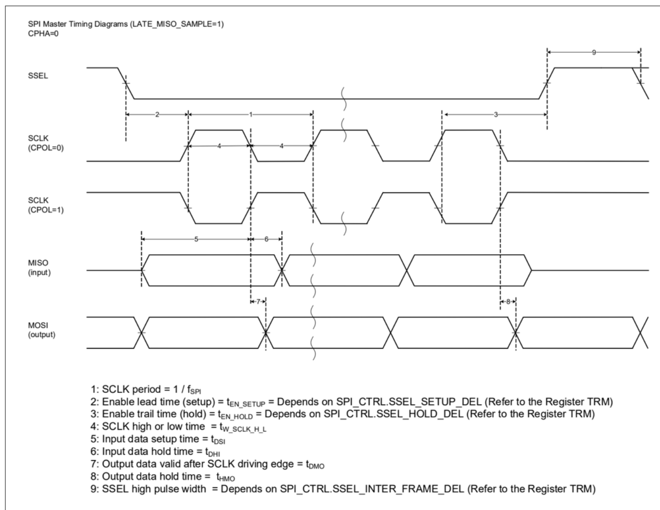
Figure 21 SPI master timing diagrams with LOW clock phase
