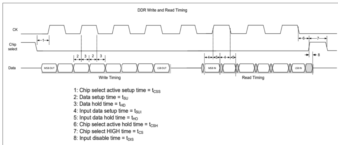
Figure 56 DDR write and read timing diagram
