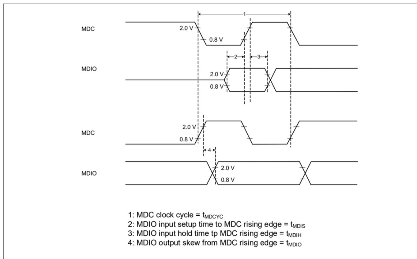
Figure 38 MDIO timing diagram
