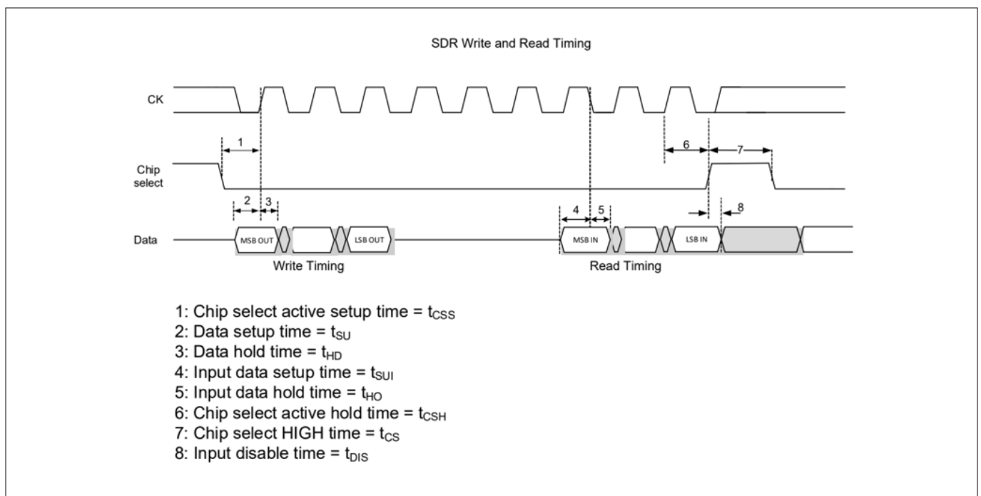
Figure 55 SDR write and read timing diagram
