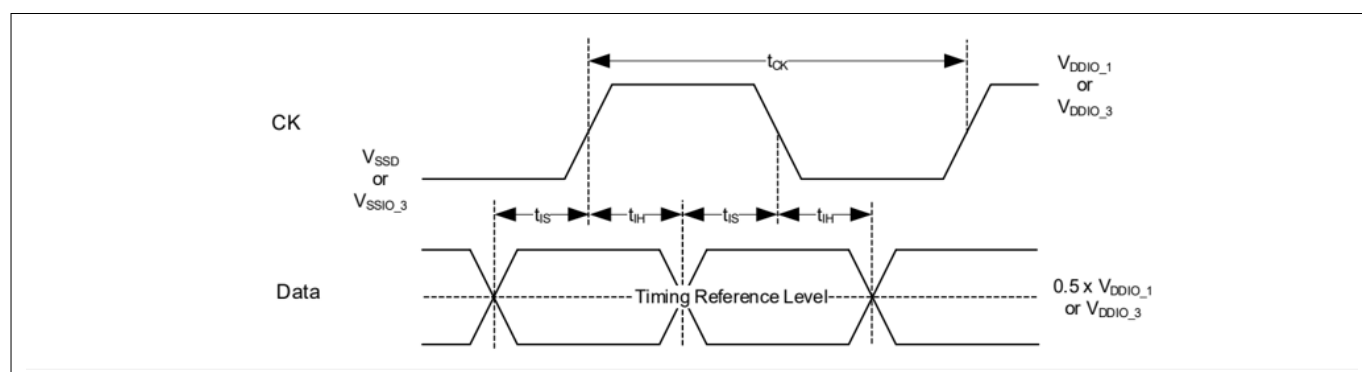
Figure 57 HYPERBUS™ timing reference level
