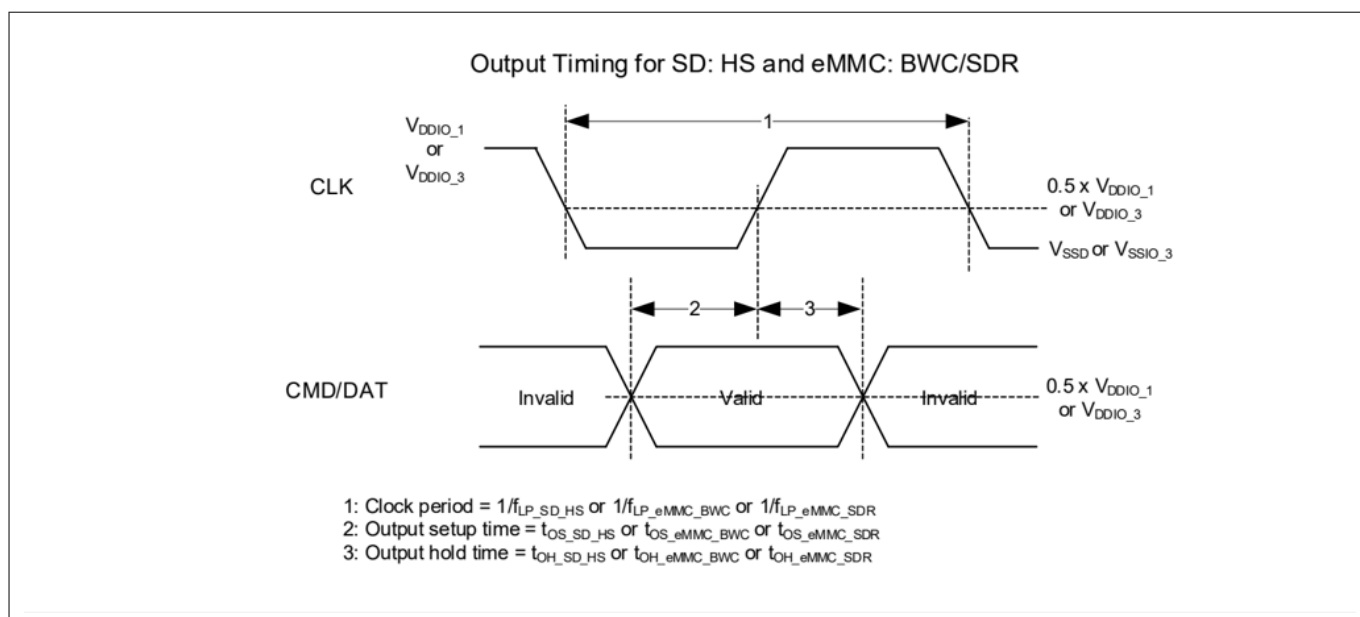
Figure 45 SD high-speed and eMMC BWC/SDR output timing
