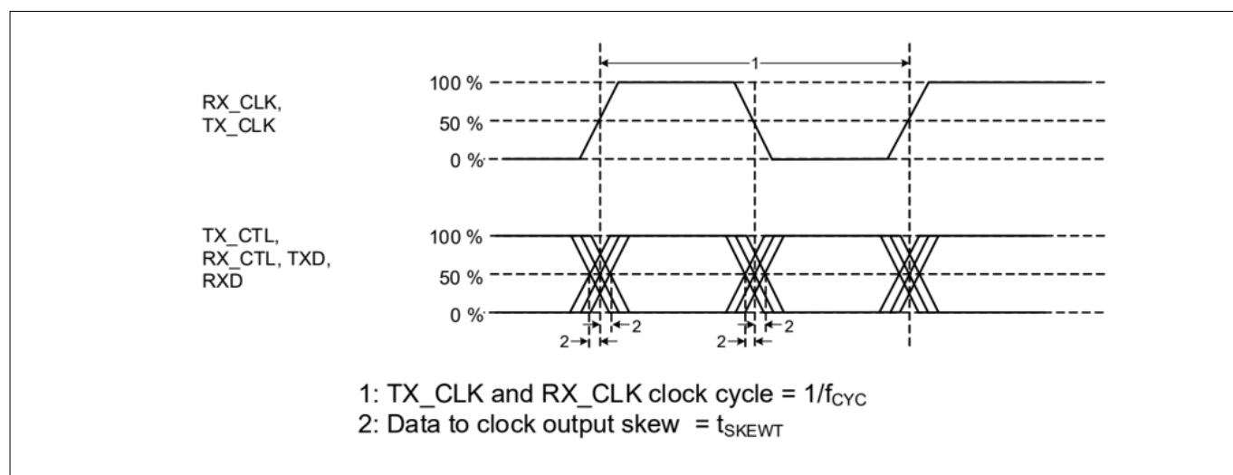
Figure 40 RGMII Tx timing diagram
