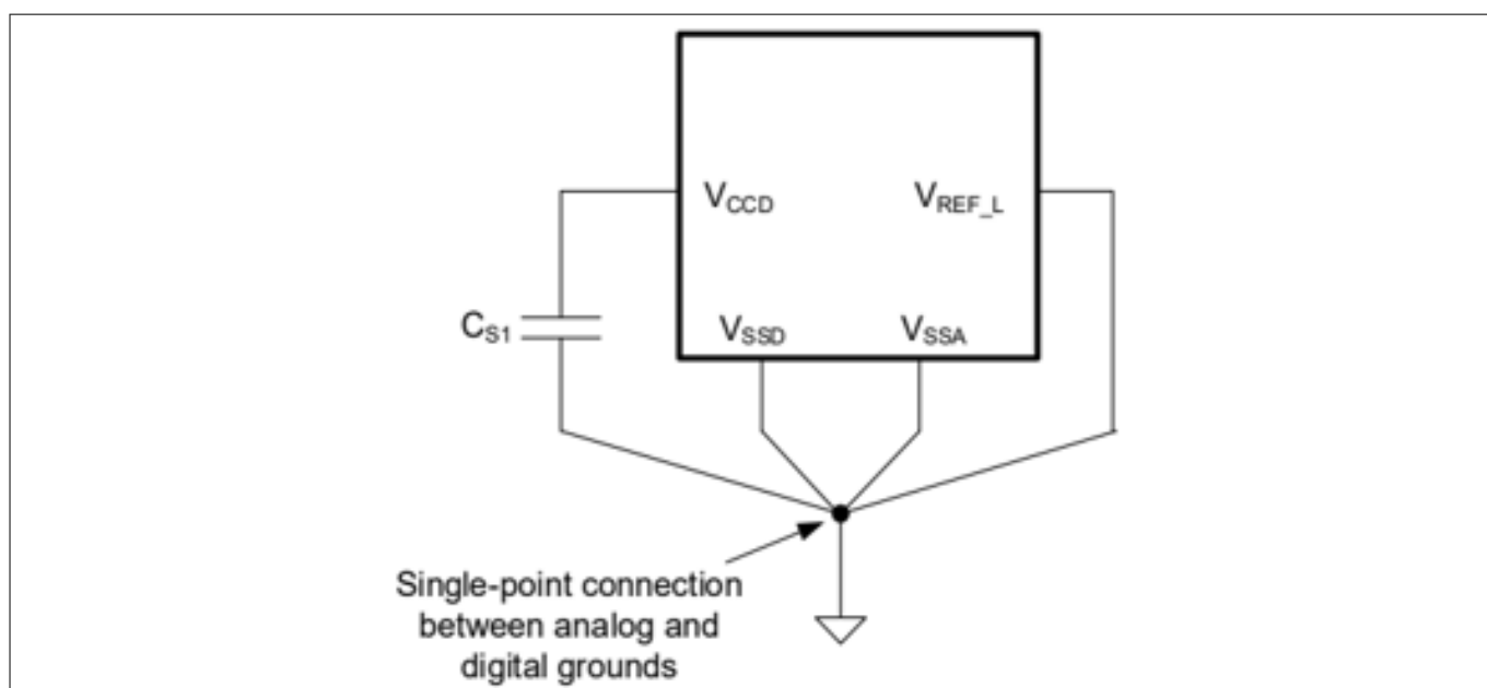
Figure 13 Smoothing capacitor
