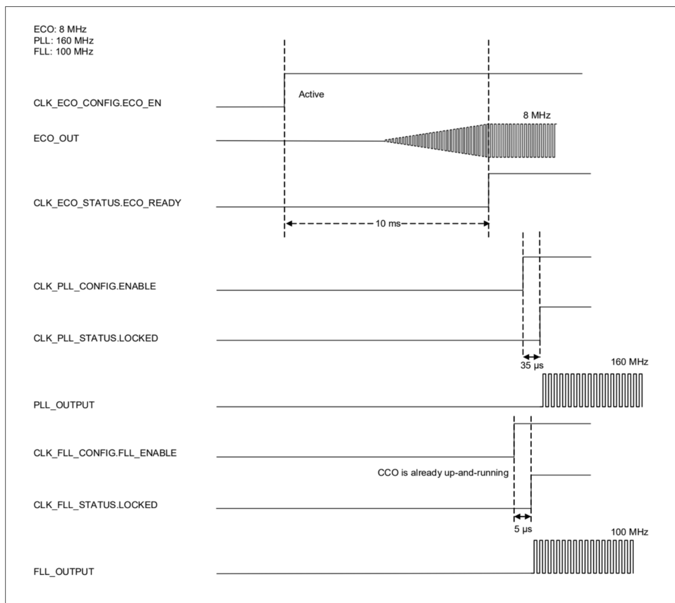
Figure 35 ECO to PLL or FLL diagram
