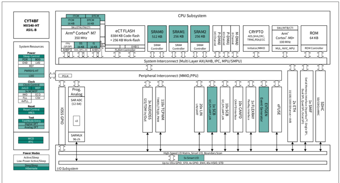
Figure 1 Architecture block diagram
