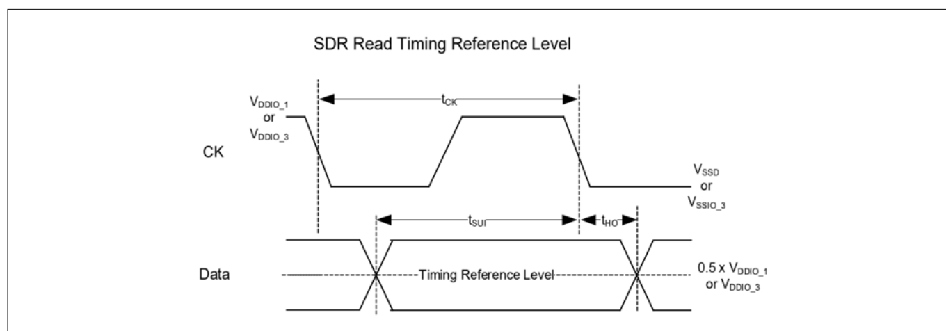
Figure 52 SDR read timing reference level
