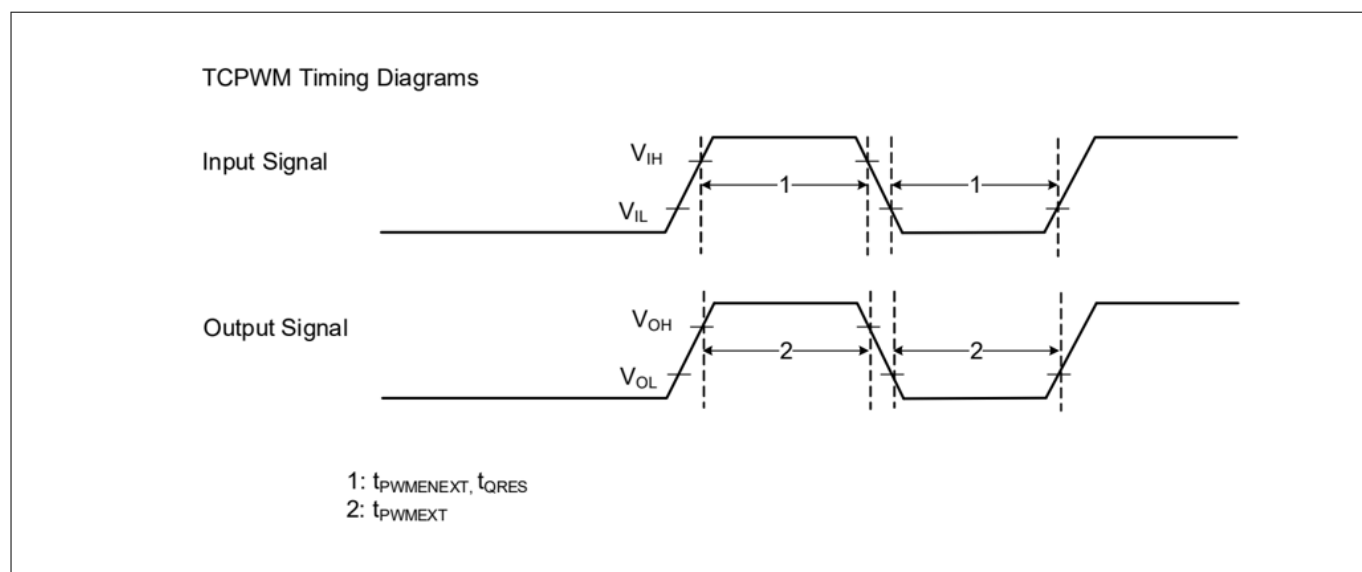
Figure 19 TCPWM timing diagrams
