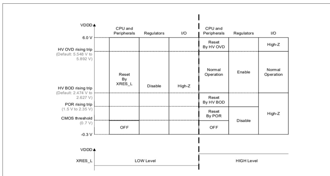
Figure 25 Device operations supply range
