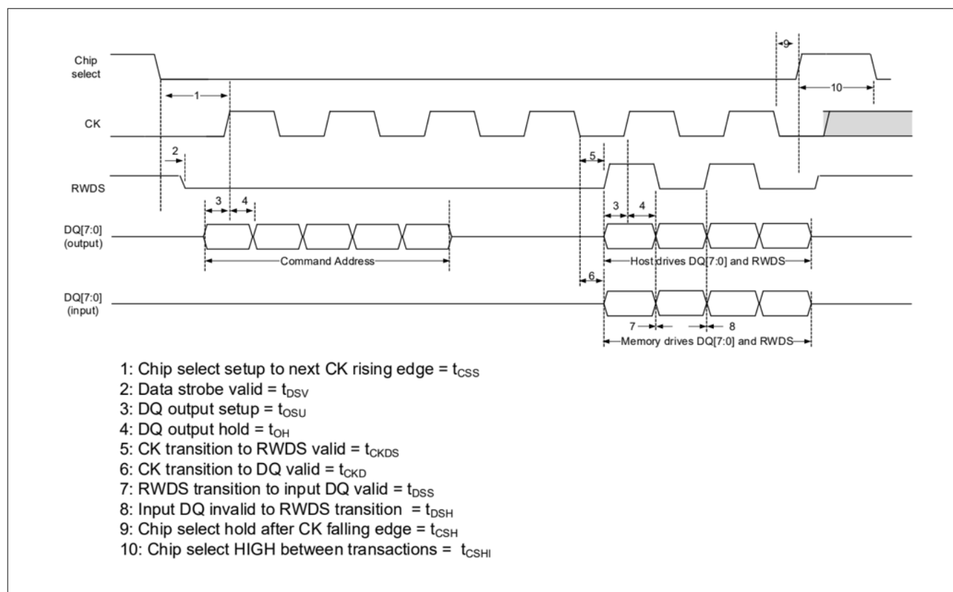
Figure 58 HYPERBUS™ timing diagram
