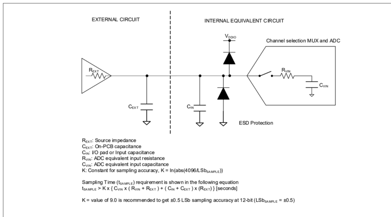
Figure 17 ADC equivalent circuit for analog input
