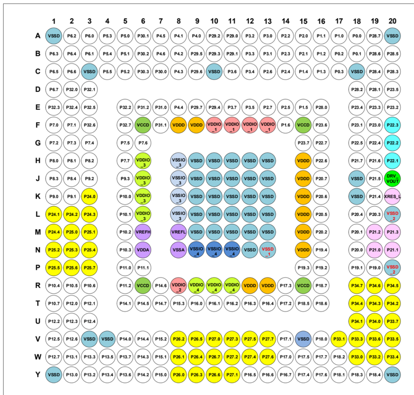
Figure 9 320-BGA ball map
