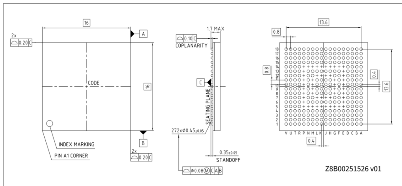
Figure 60 Package outline – 272-BGA
