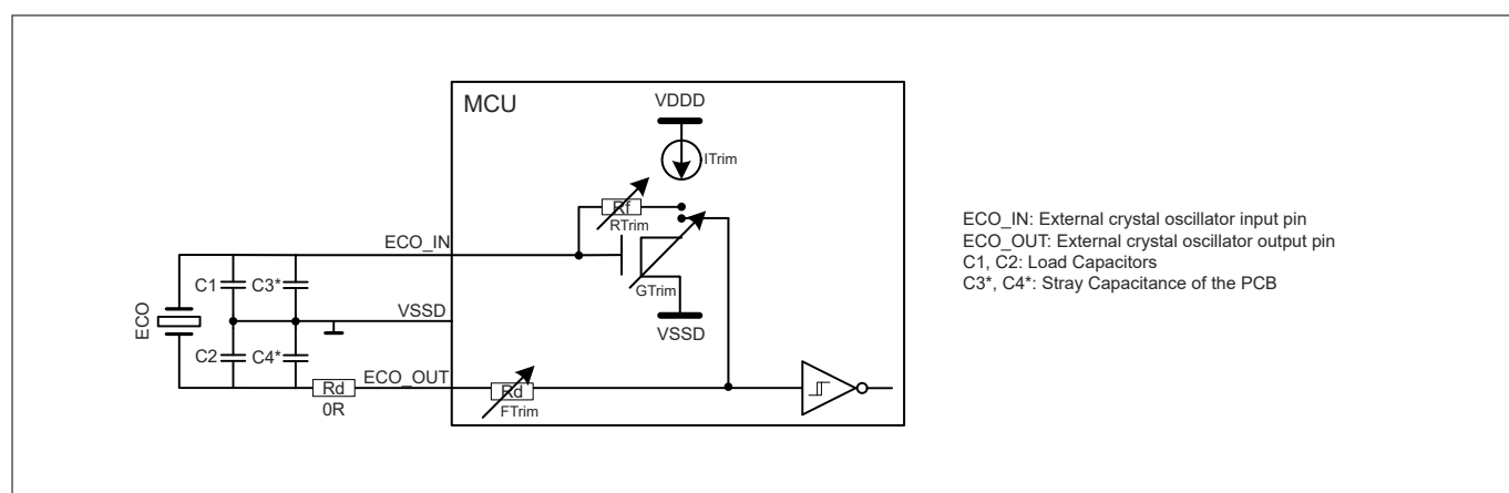
Figure 33 ECO connection scheme 18)
