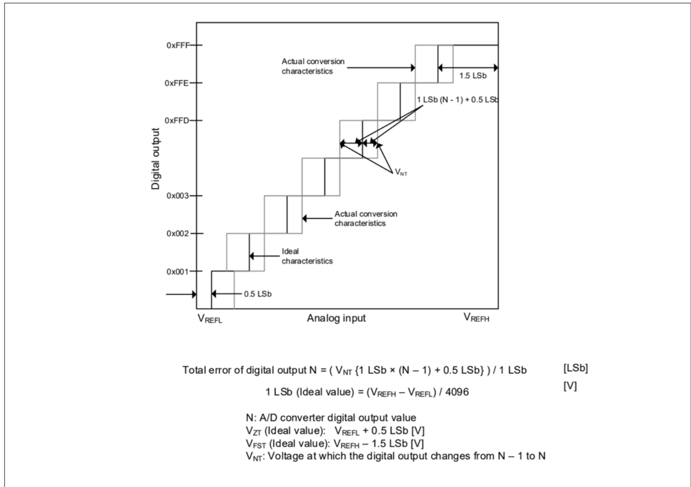
Figure 15 ADC characteristics and error descriptions
