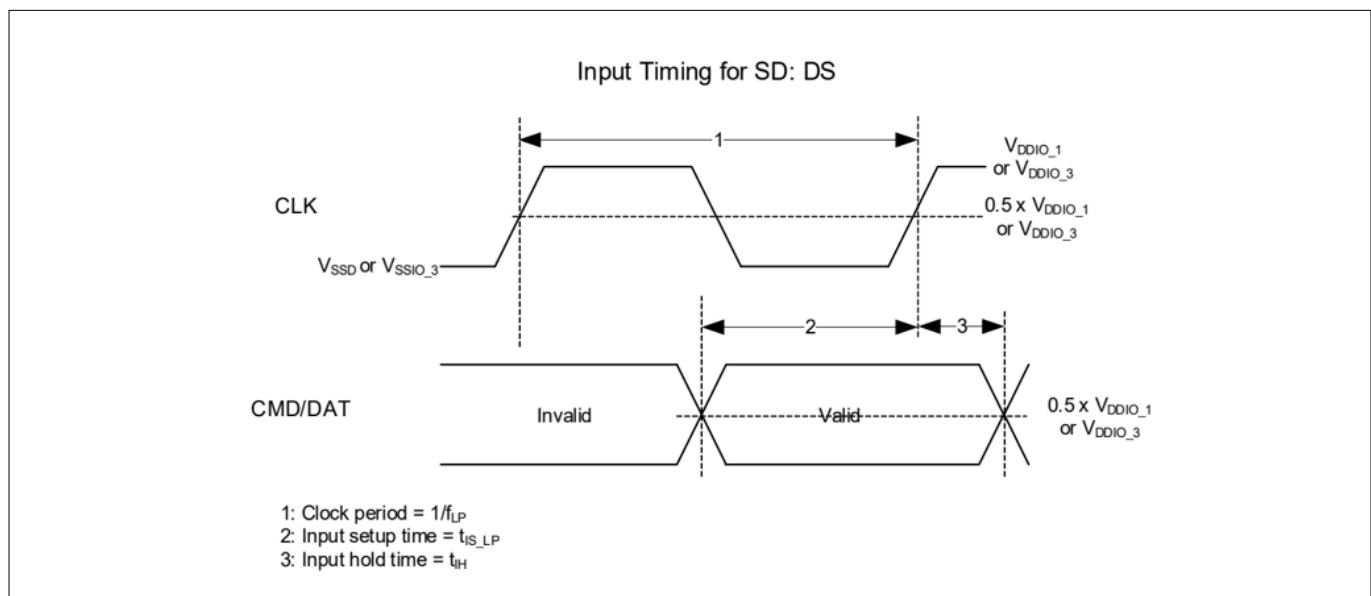
Figure 42 SD default speed input timing
