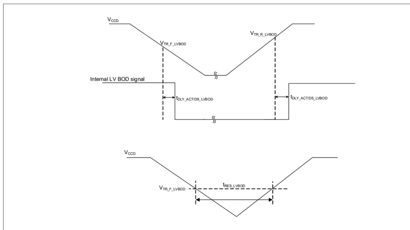
Figure 28 Low-voltage BOD specifications
