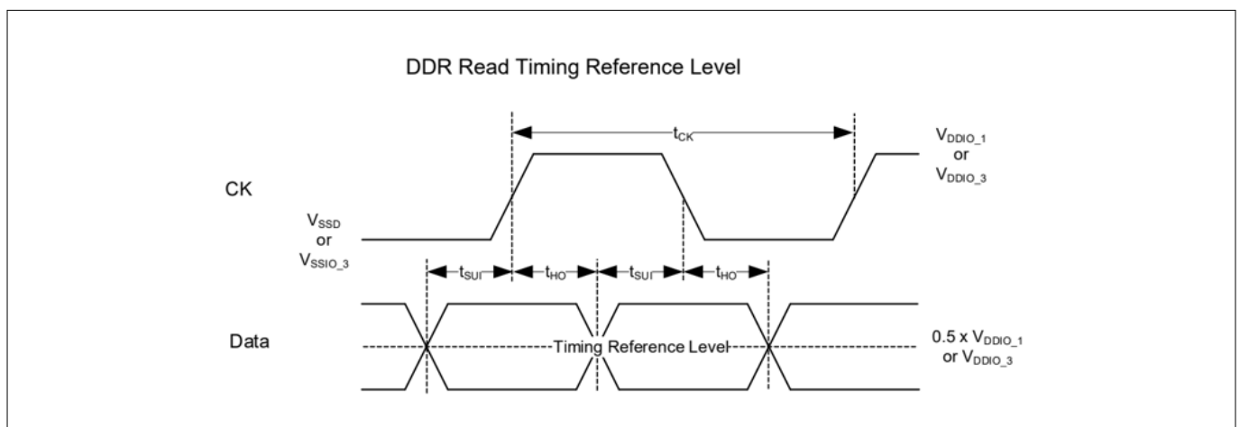
Figure 54 DDR read timing reference level
