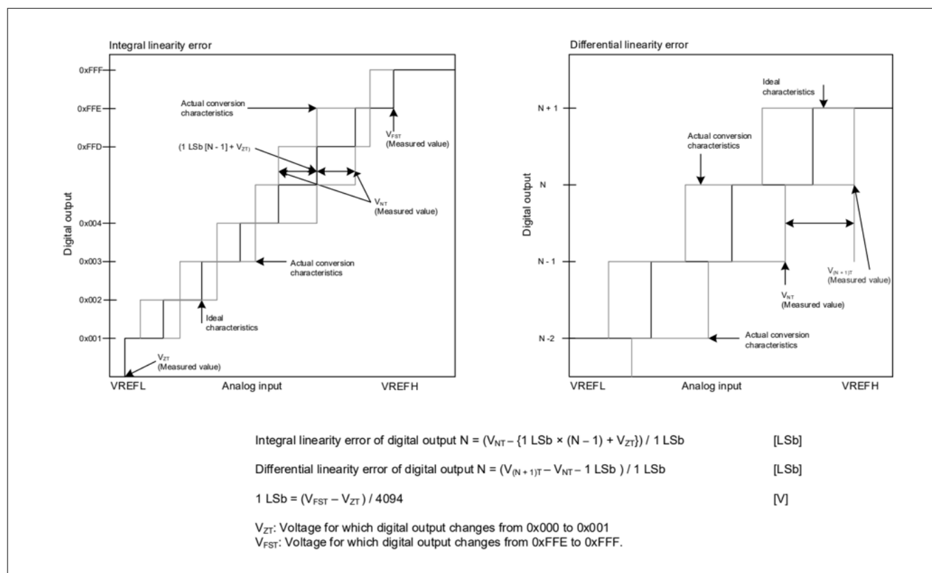
Figure 16 Integral and differential linearity errors
