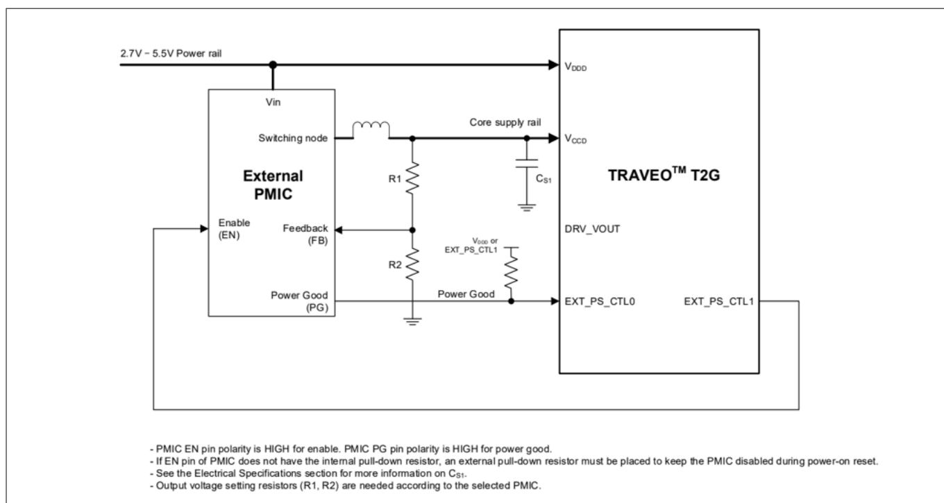
Figure 3 Sample core external regulator with PMIC/LDO
