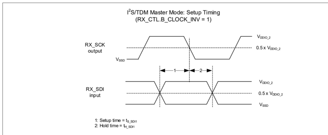
Figure 48 Master setup with clock inversion
