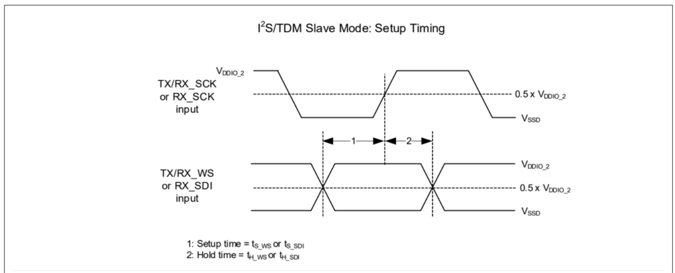
Figure 50 Slave setup
