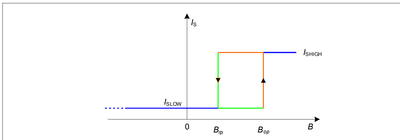
Figure 4 Output Signal
