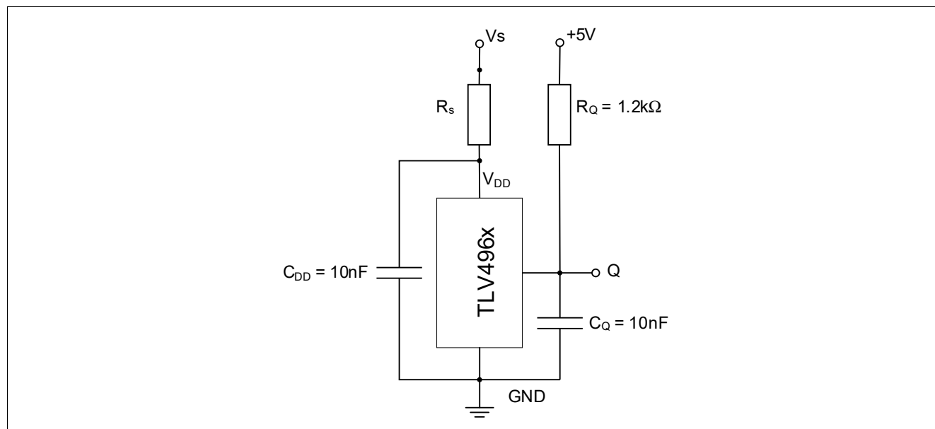
Figure 10 EMC test circuit
