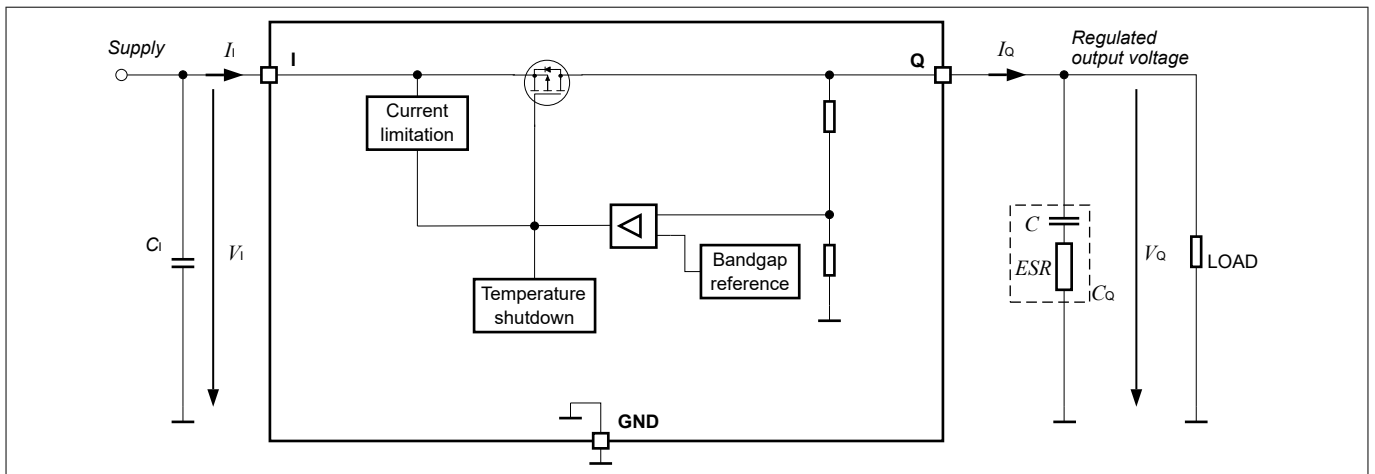
Figure 3 Voltage regulation
