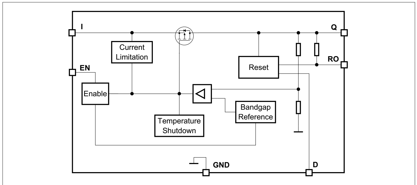
Figure 1 Block diagram
