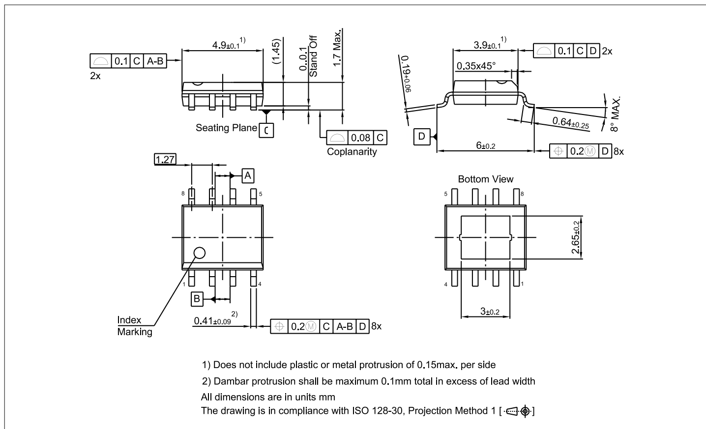
Figure 6 PG-DSO-8 EP
