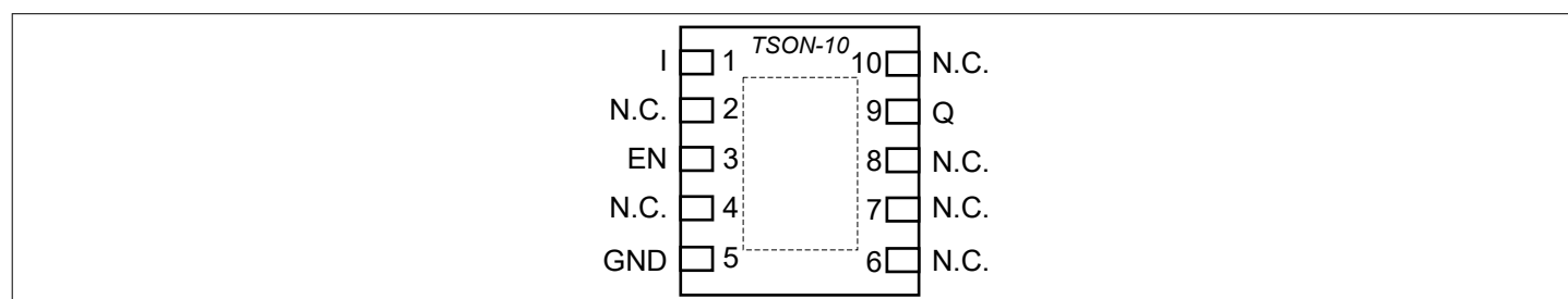
Figure 3 Pin configuration
