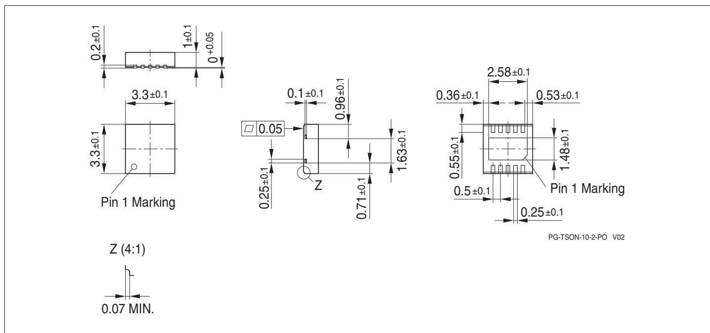
Figure 7 PG-TSON-10-2-PO 1)
