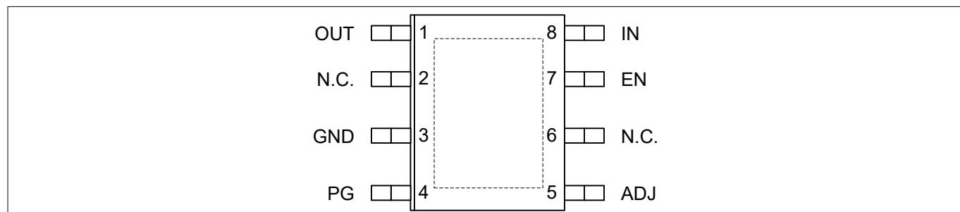
Figure 2 Pin configuration
