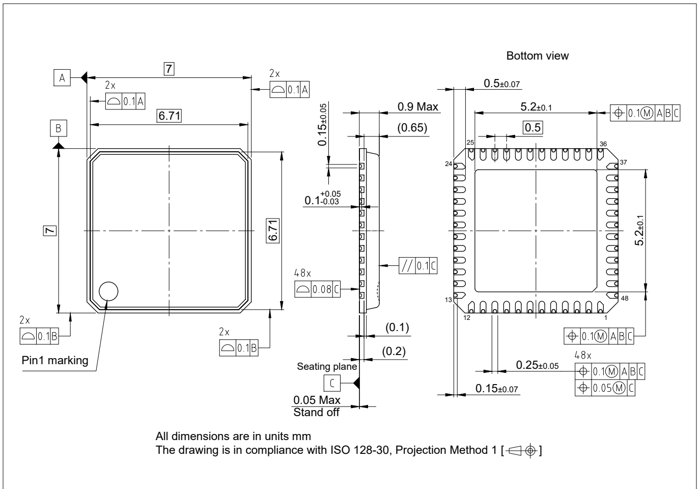
Figure 2 PG-VQFN-48-79
