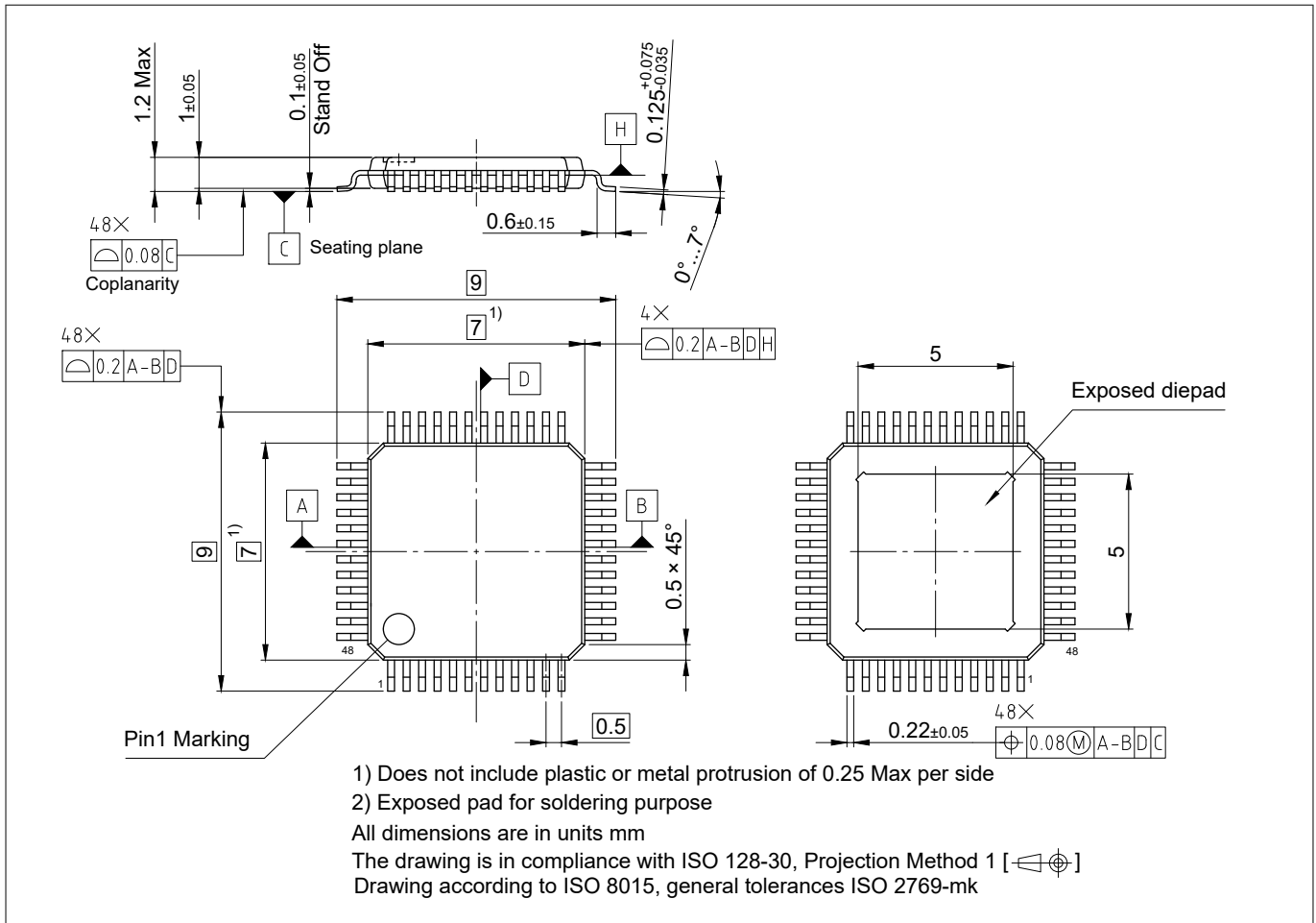
Figure 2 PG-TQFP-48-10
