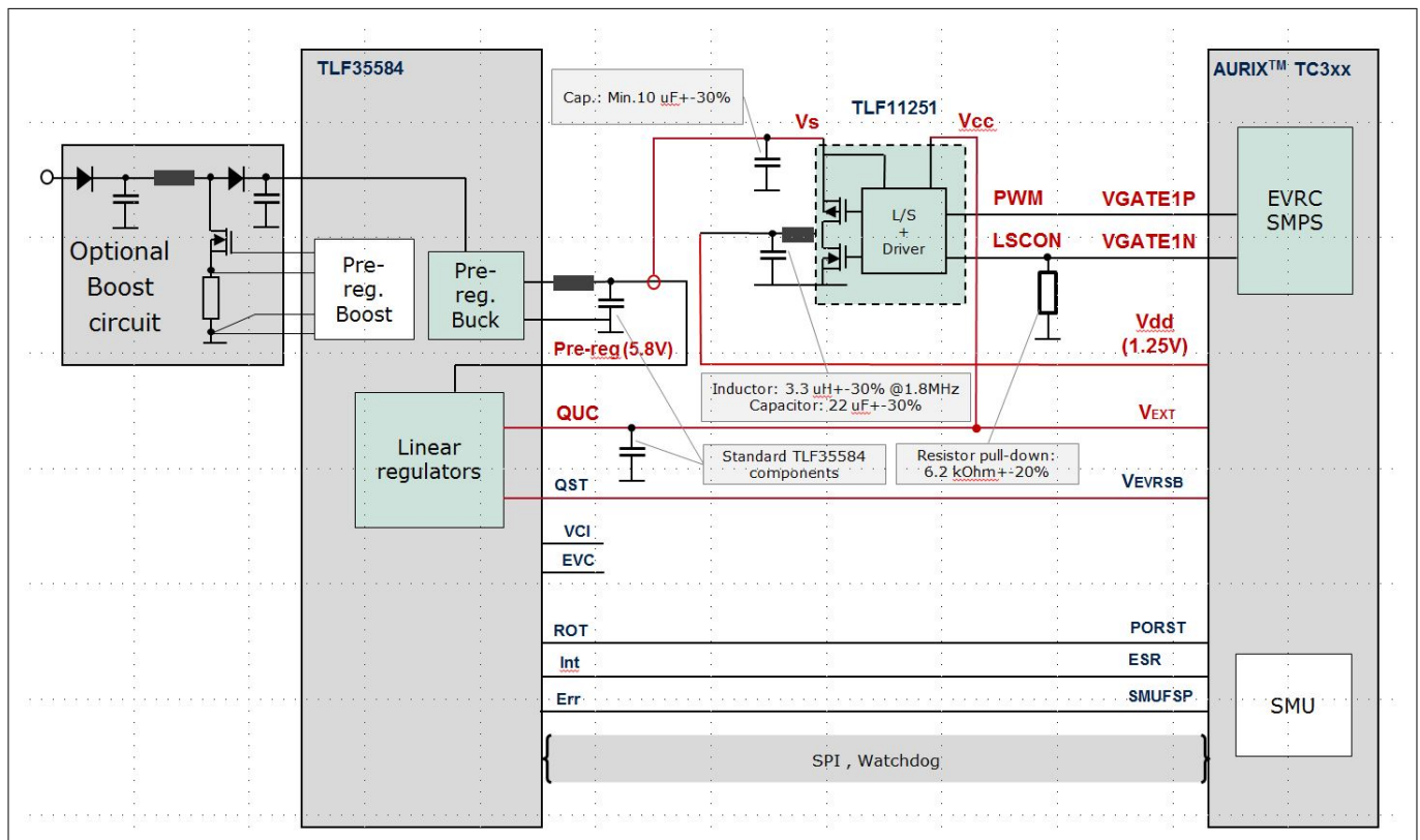
Figure 5 Application diagram
