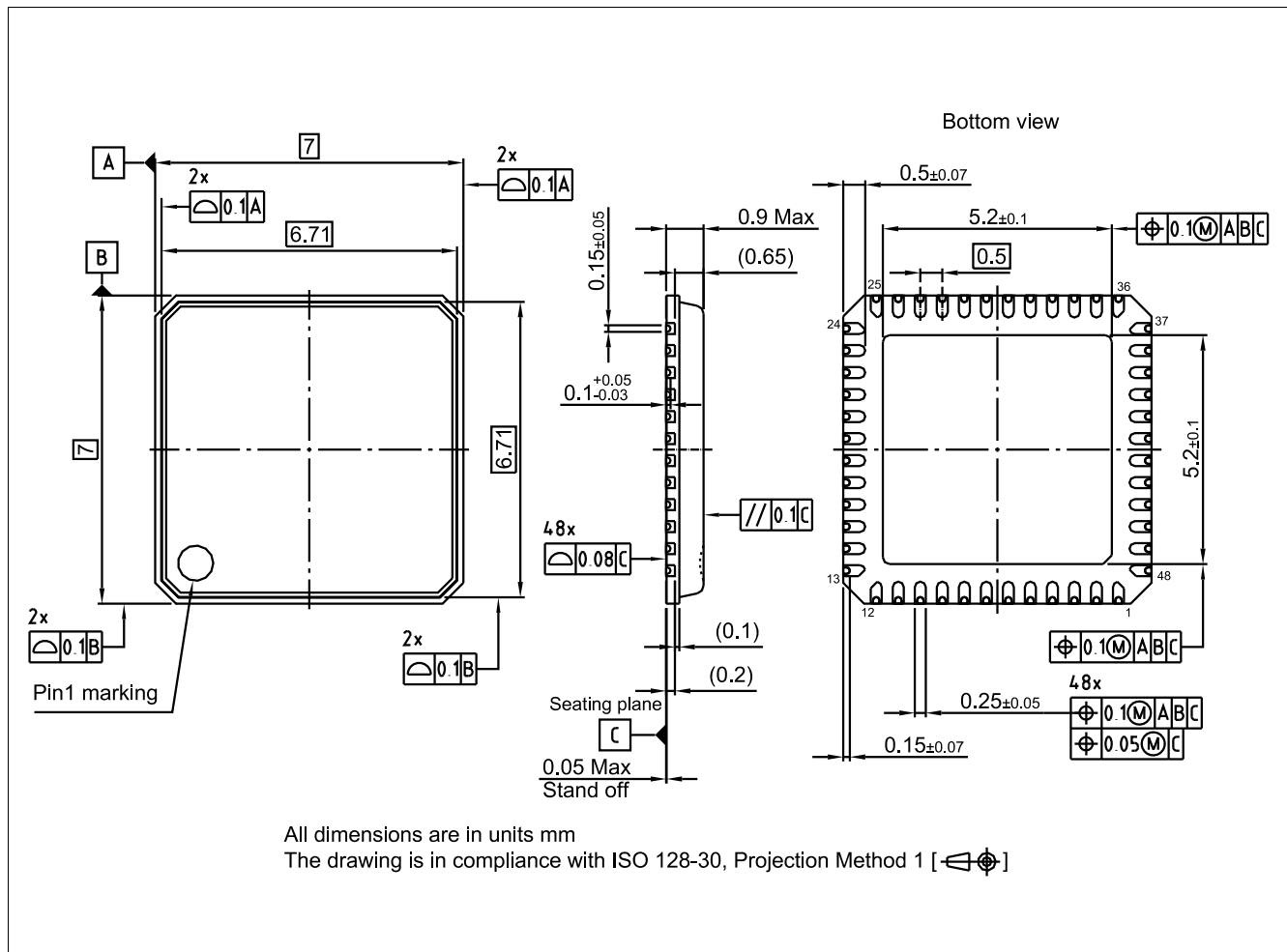
Figure 39 Package outline VQFN-48-79 with LTI (UH and UI step) 1)
