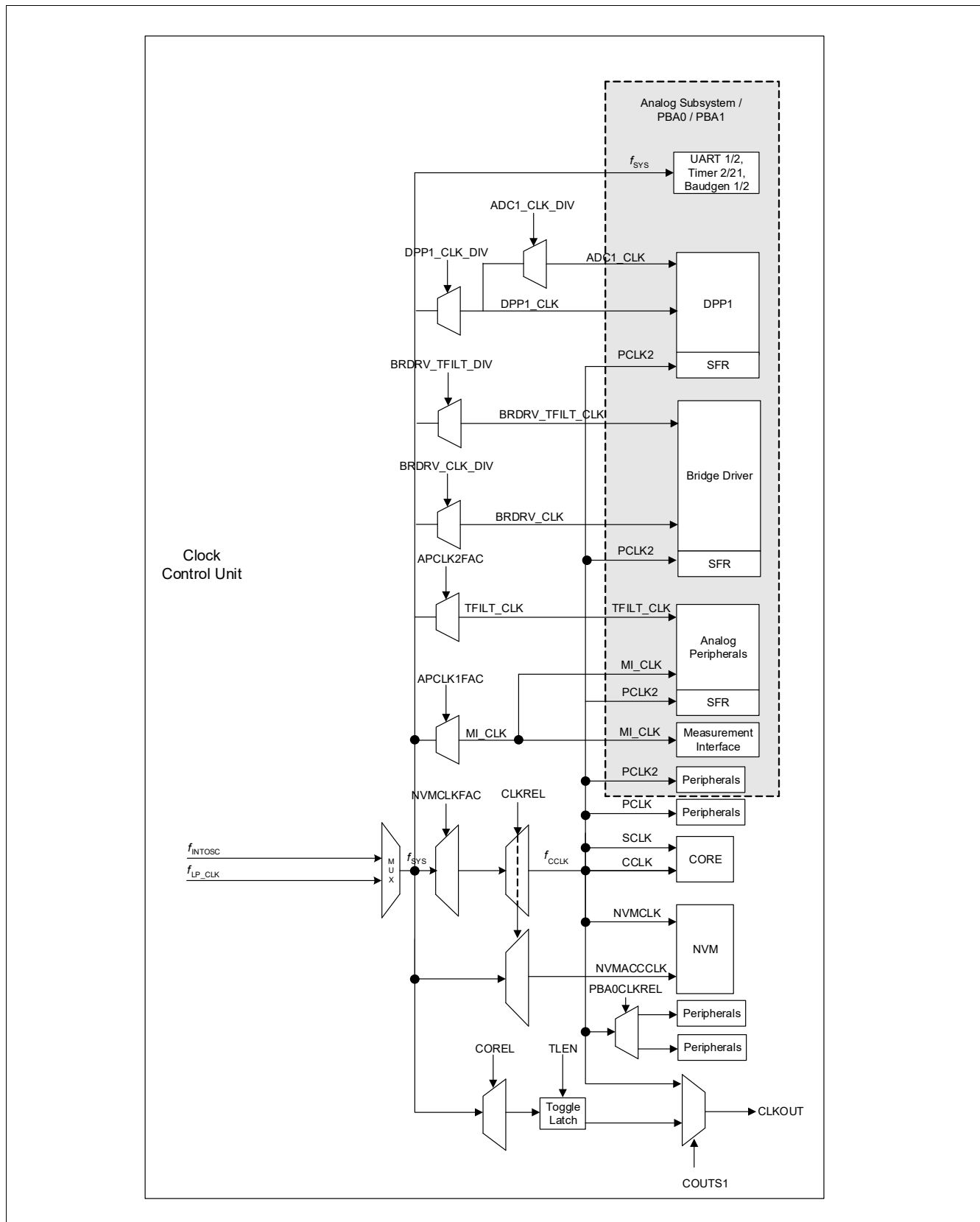
Figure 12 Clock Generation from f_{\text{sys}} ; CLKOUT Generation
