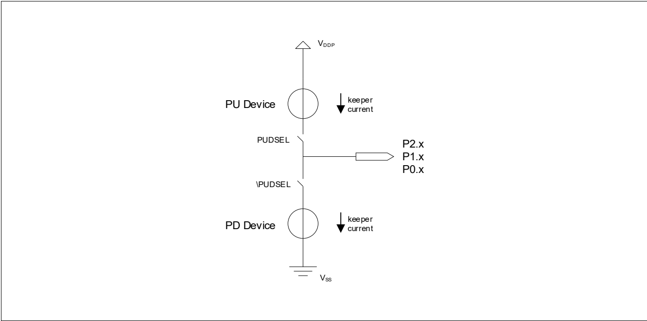
Figure 44 Pull-Up/Down Device
