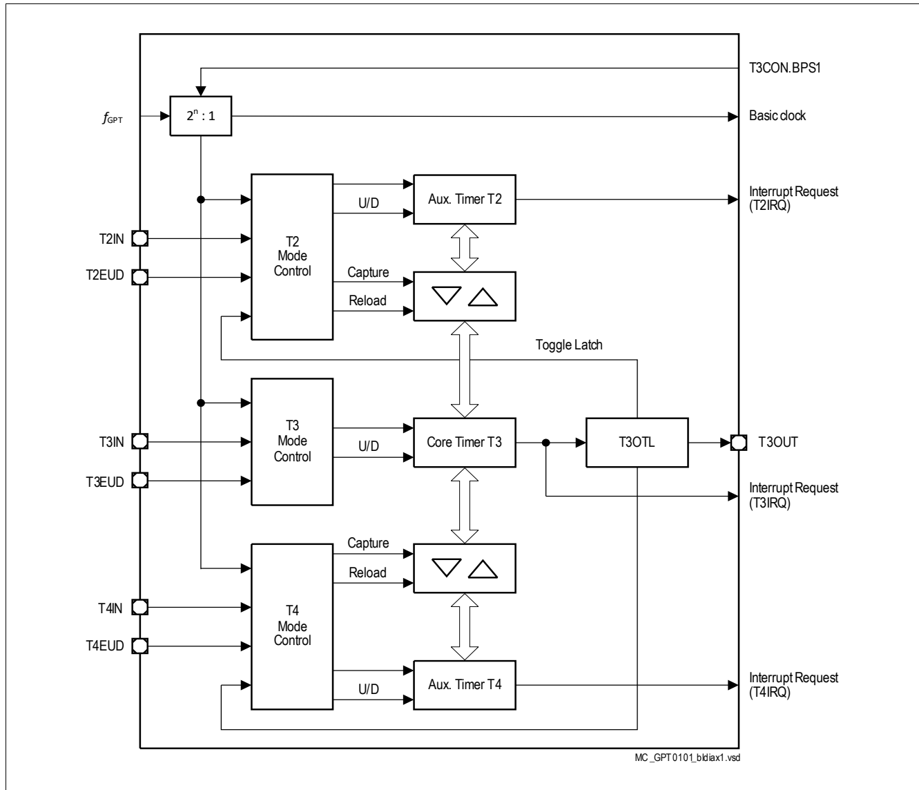
Figure 21 GPT1 Block Diagram ( n = 2 \dots 5 )
