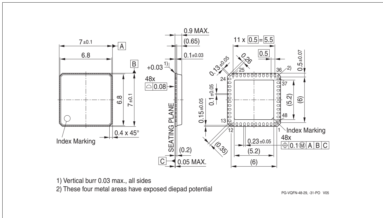
Figure 48 VQFN-48-29 (with LTI)
