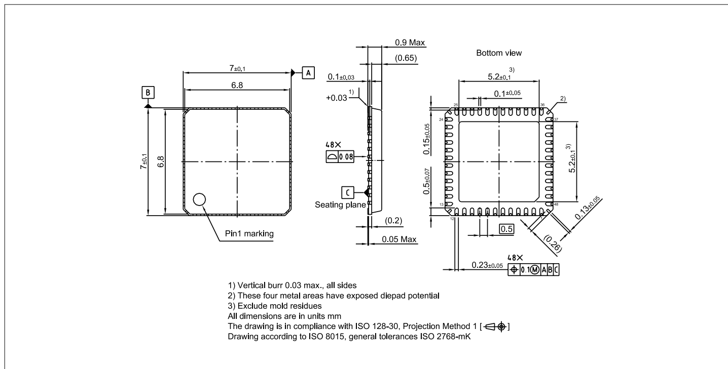
Figure 69 PG-VQFN-48
