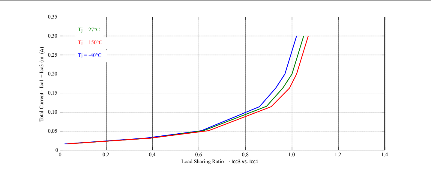
Figure 22 Load Sharing Ratio ICC1 : ICC3 vs. the total load current
