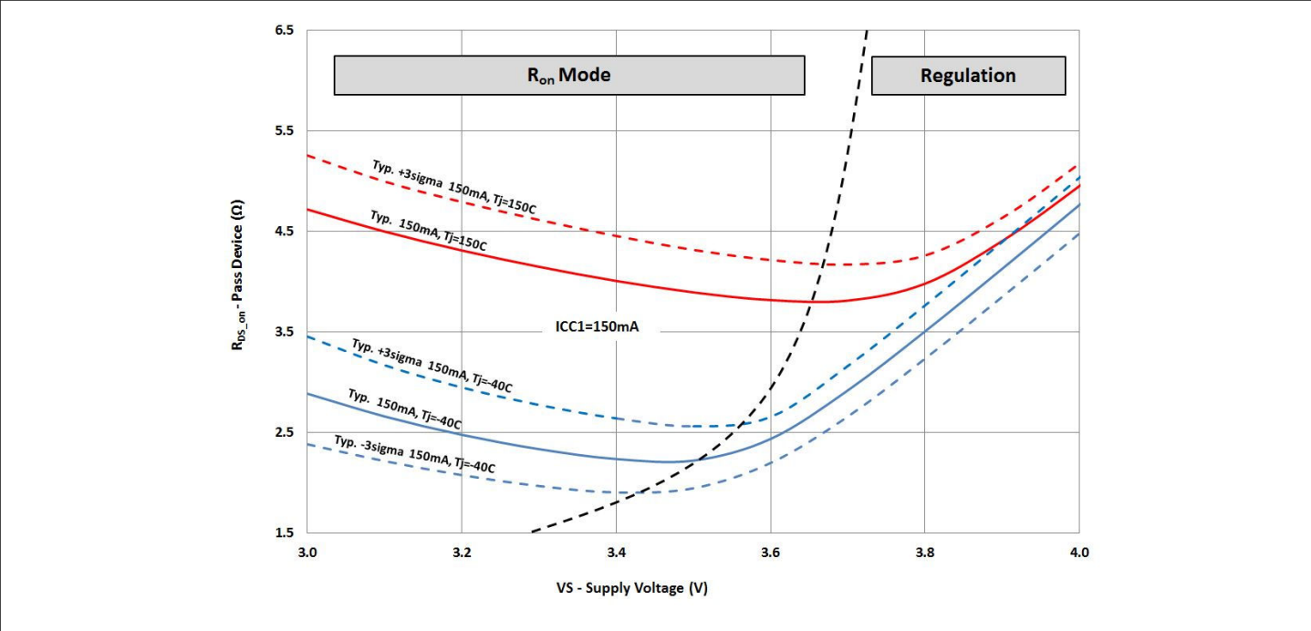
Figure 13 Characterization results of on-resistance range of VCC1 pass device during low drop operation for I_{CC1} = 150\text{mA}
