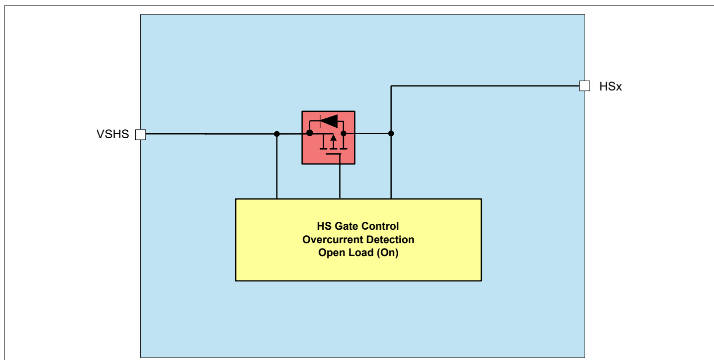
Figure 24 High-Side Module Block Diagram
