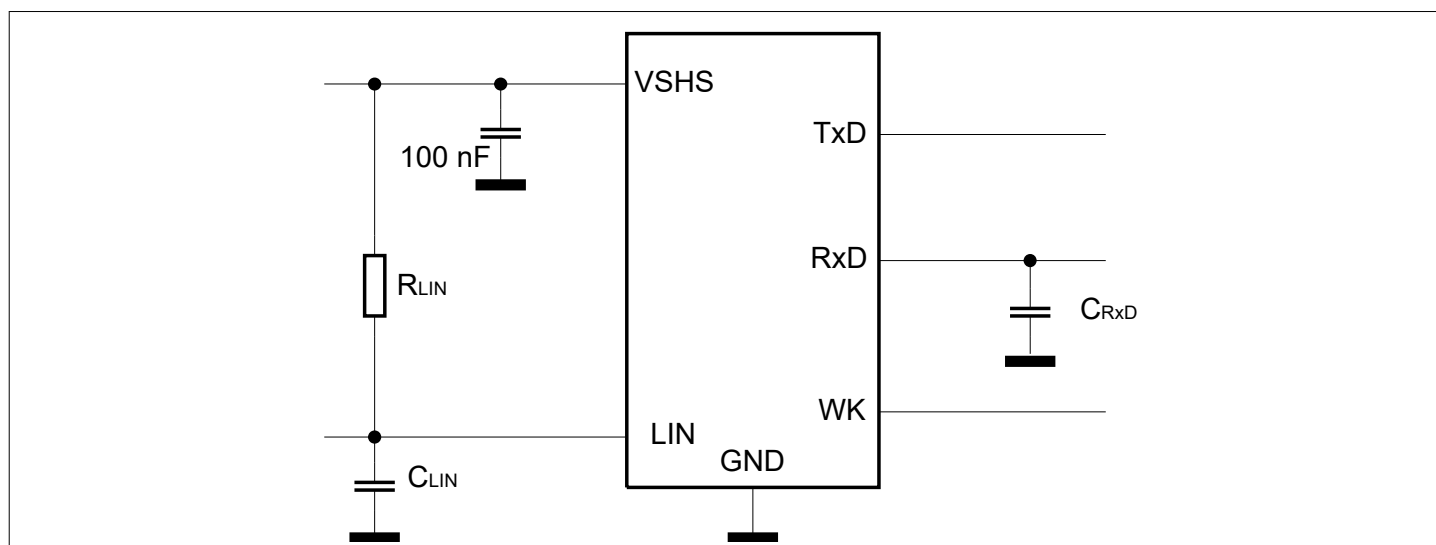
Figure 36 Simplified Test Circuit for Dynamic Characteristics
