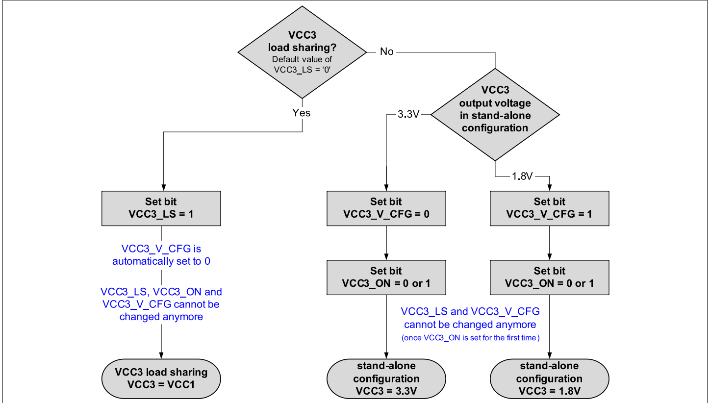
Figure 18 Selecting the Configuration of the VCC3 Regulator
