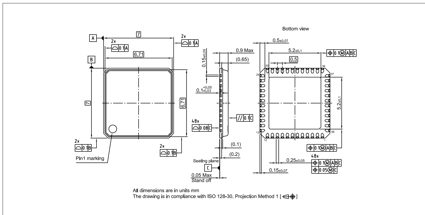
Figure 65 PG-VQFN-48
