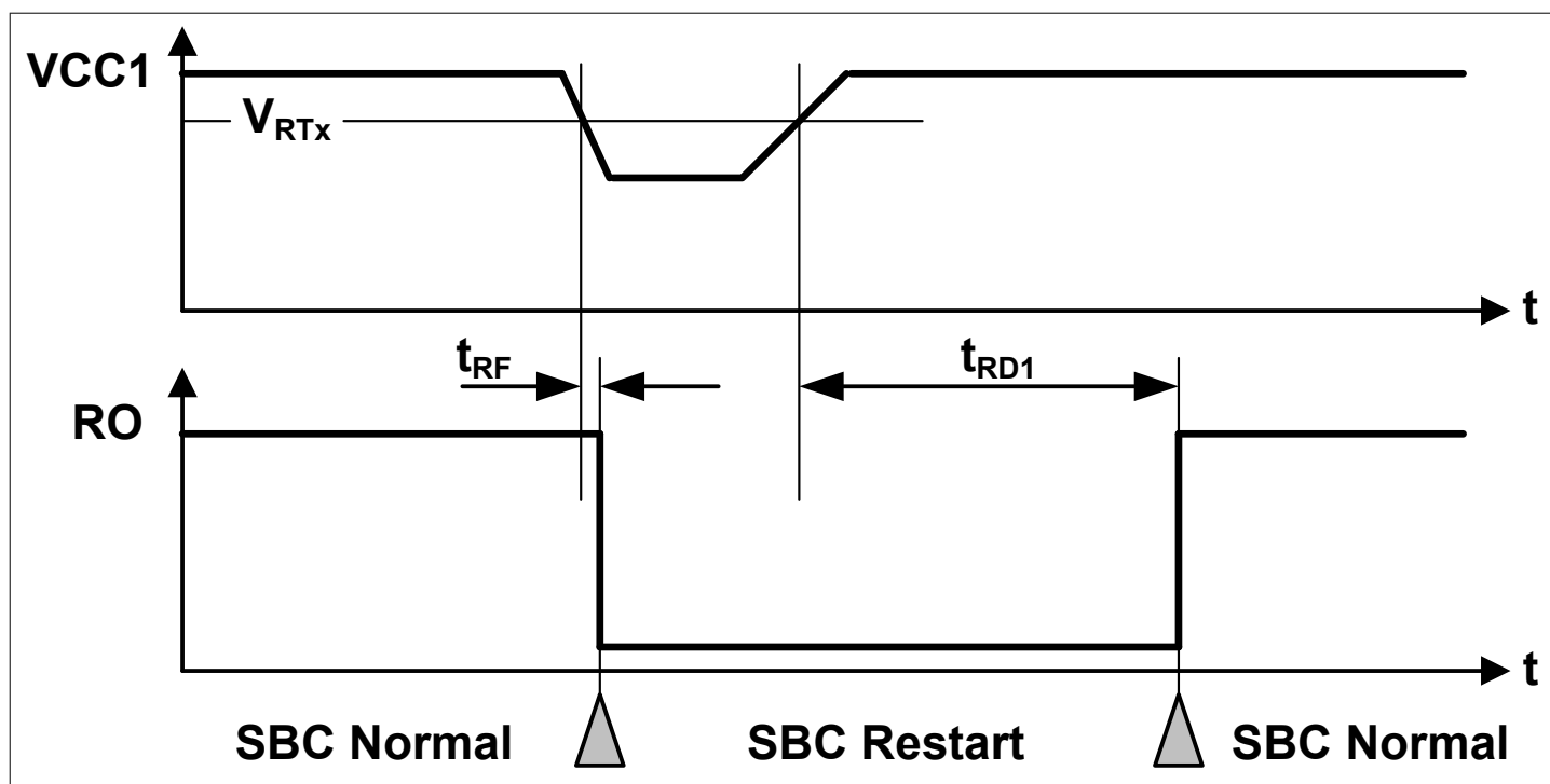
Figure 52 VCC1 Undervoltage Timing Diagram
