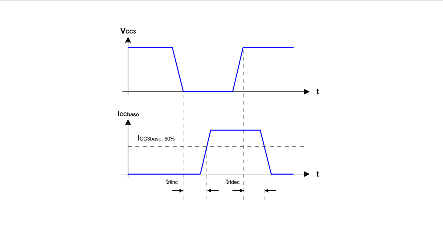
Figure 21 Regulator Reaction Time
