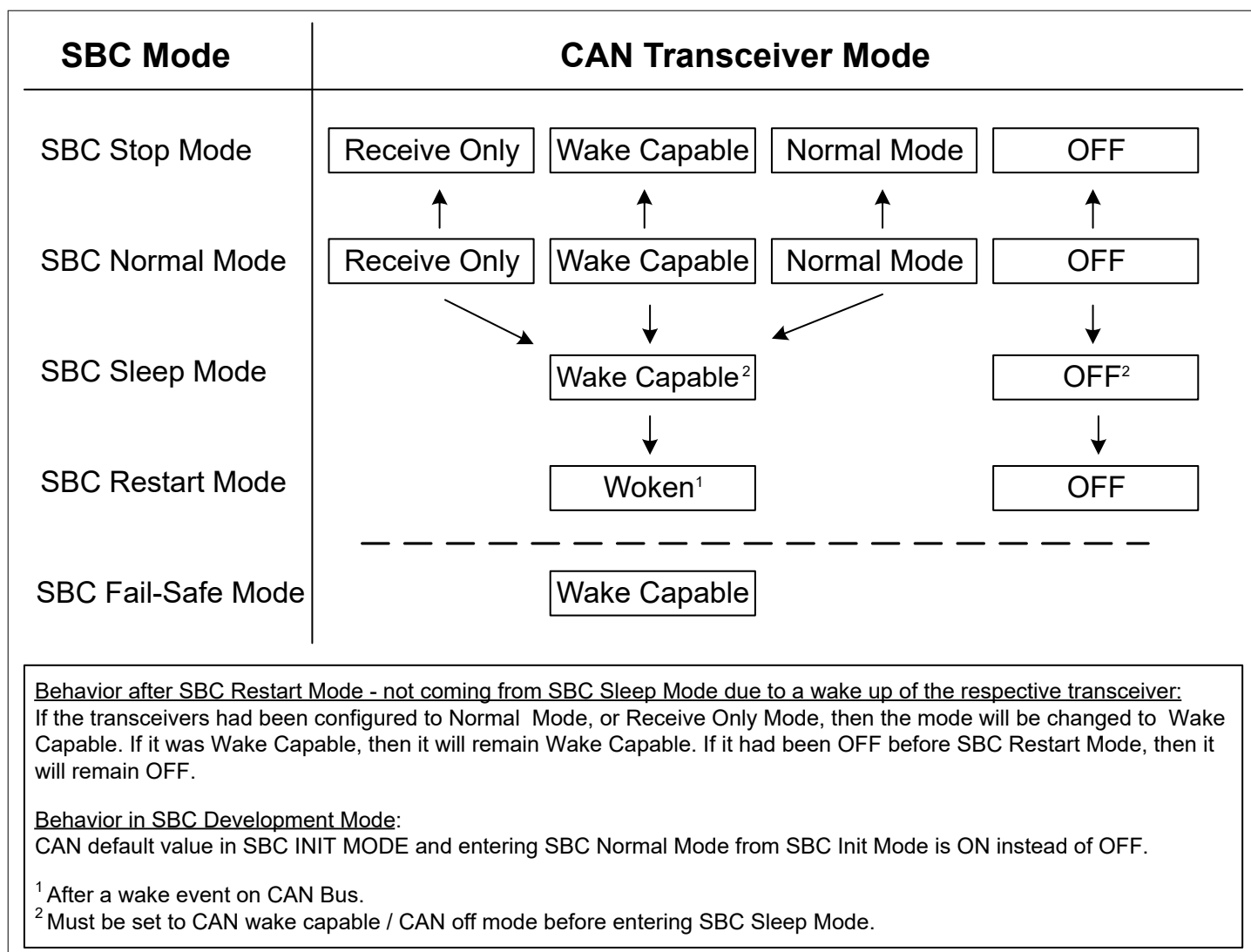
Figure 26 CAN Mode Control Diagram
