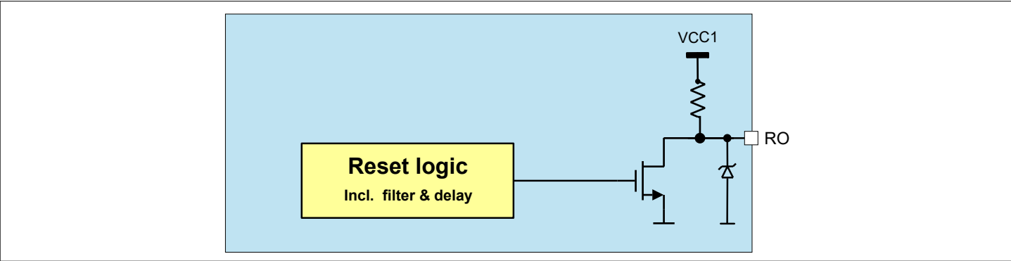
Figure 46 Reset Block Diagram
