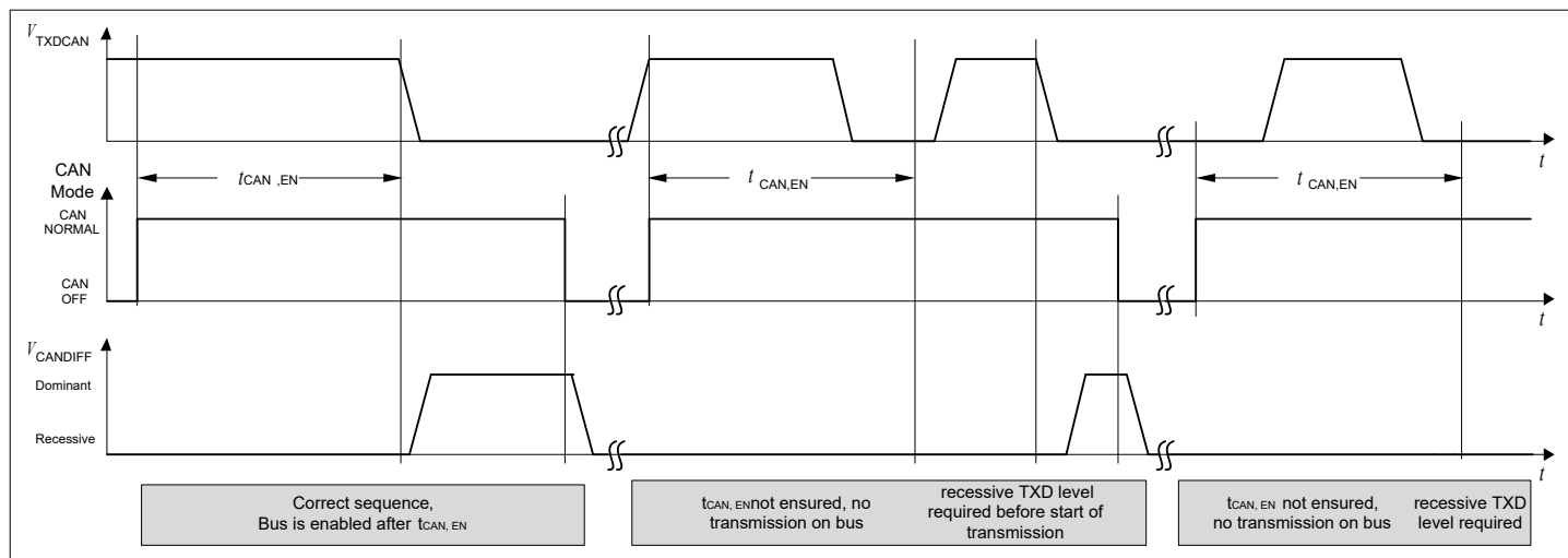
Figure 28 CAN Transceiver Enabling Sequence
