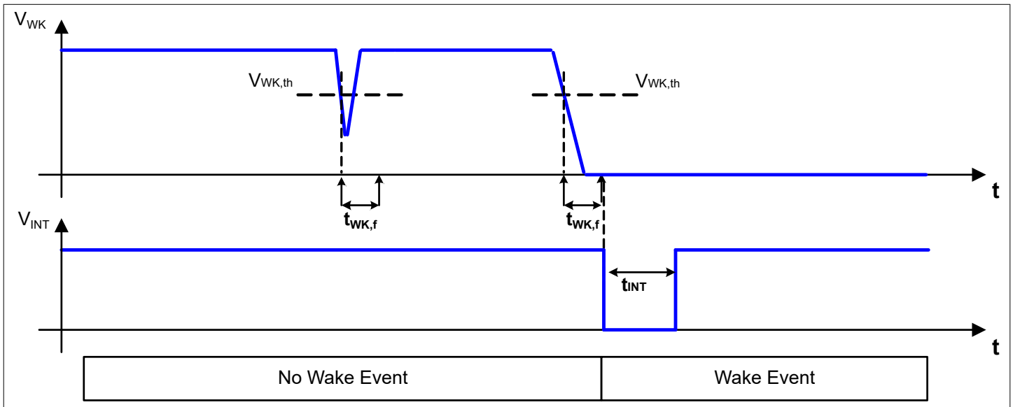
Figure 39 Wake-up Filter Timing for Static Sense
