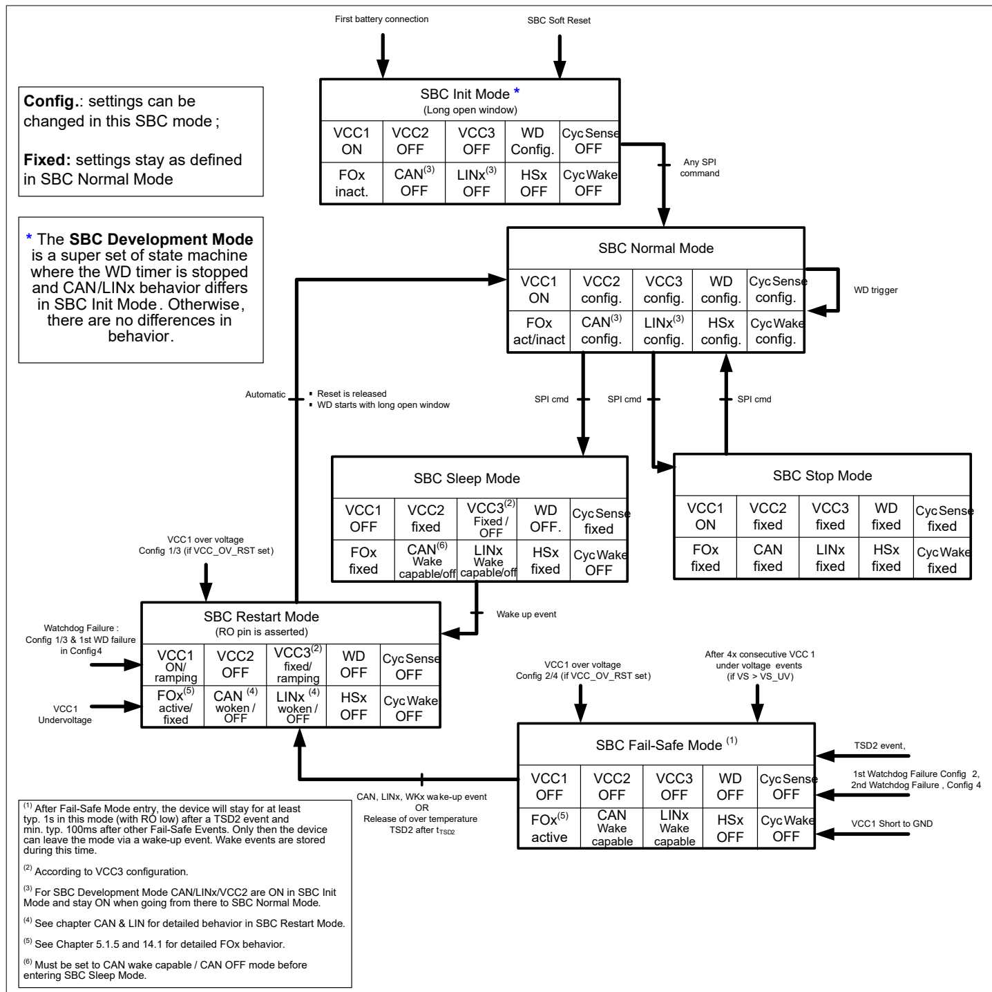
Figure 3 State Diagram showing the SBC Operating Modes
