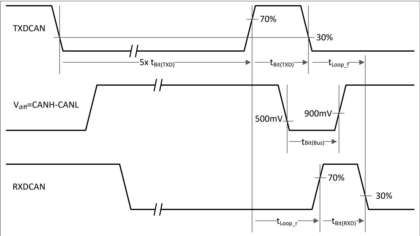
Figure 31 From ISO 11898-2: t_{loop} , t_{bit(TXD)} , t_{bit(Bus)} , t_{bit(RXD)} definitions
