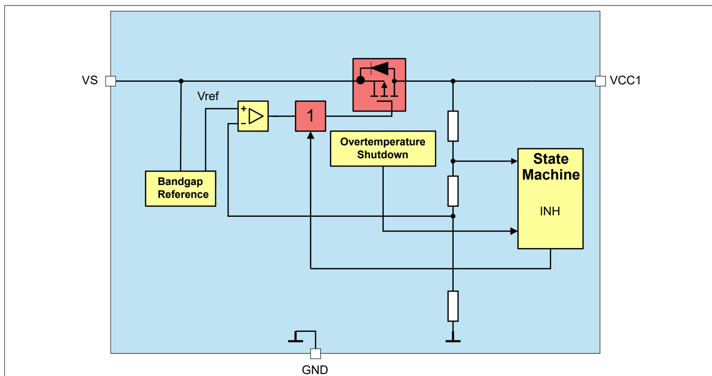
Figure 11 Module Block Diagram
