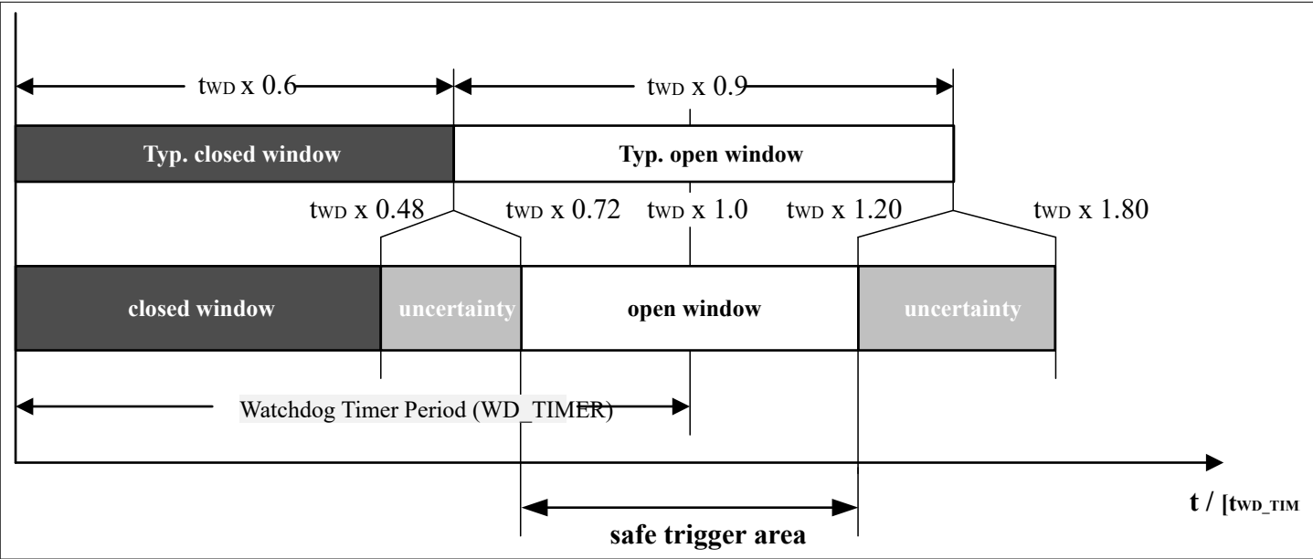
Figure 49 Window Watchdog Definition
