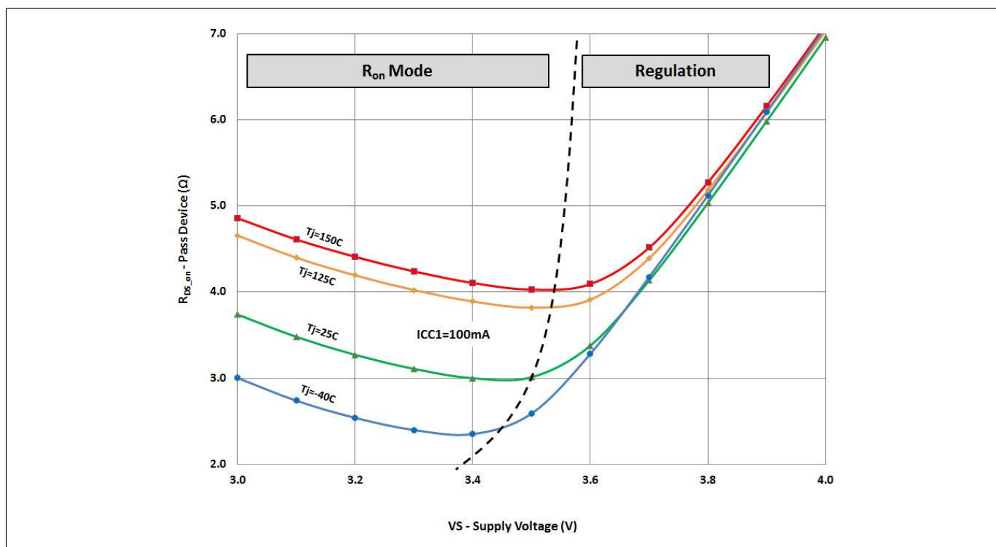
Figure 12 Typical on-resistance characterization results of VCC1 pass device during low drop operation for I_{CC1} = 100\text{ mA}
