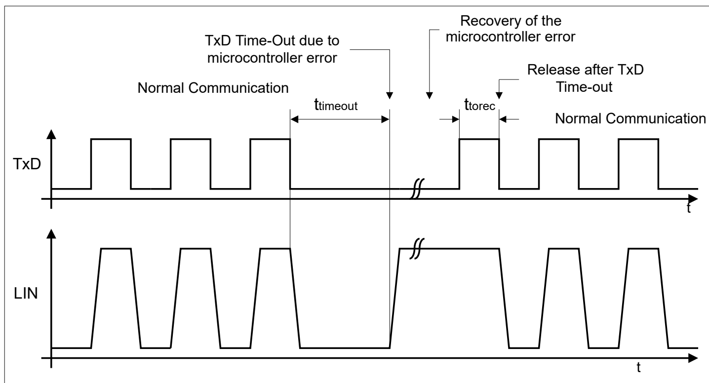
Figure 35 TXD Time-Out Function
