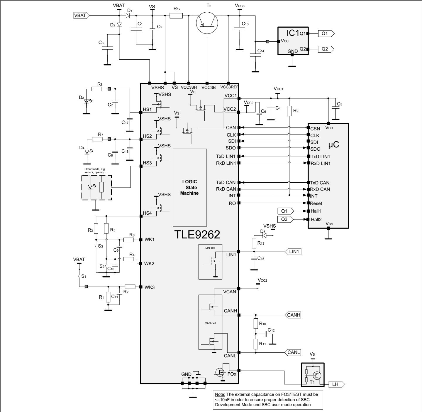
Figure 59 Simplified Application Diagram
