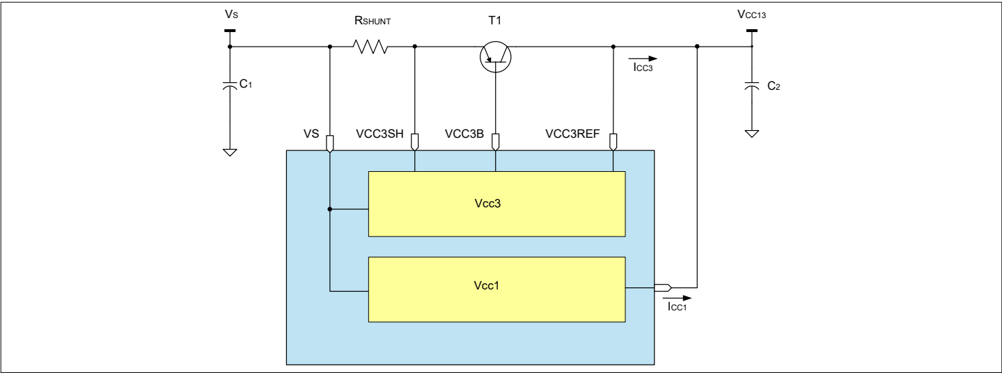
Figure 20 VCC3 in Load Sharing Configuration
