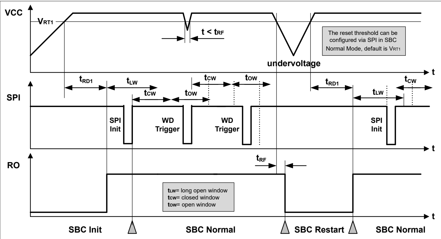
Figure 47 Reset Timing Diagram
