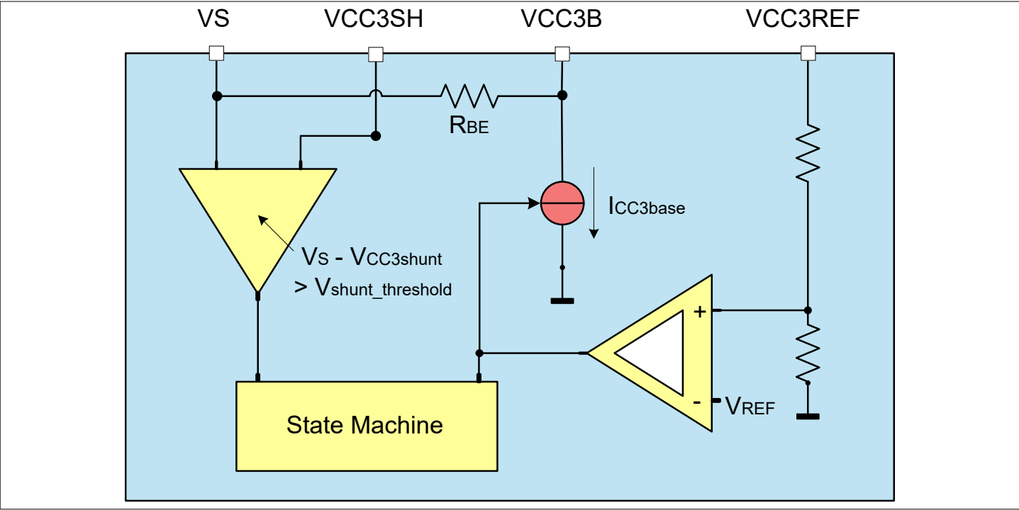
Figure 17 Functional Block Diagram
