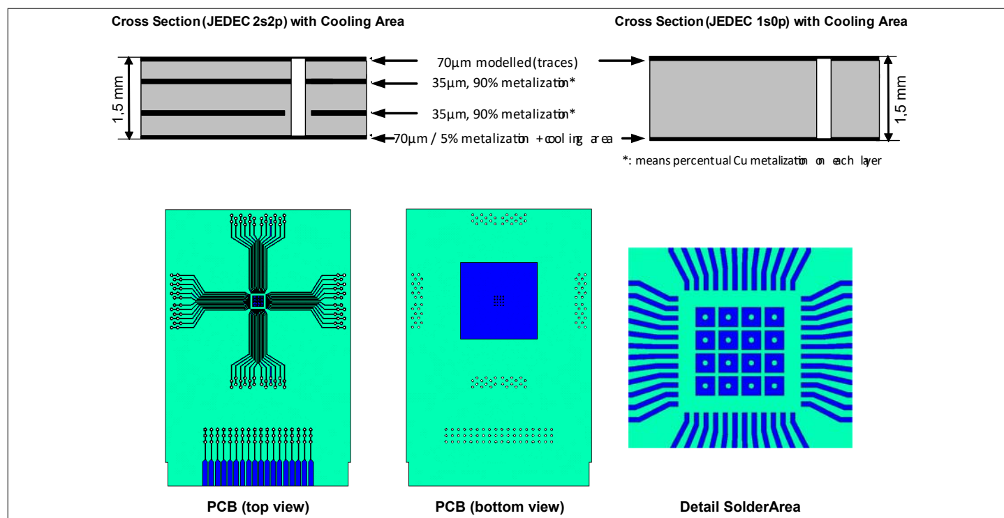
Figure 63 Board Setup
