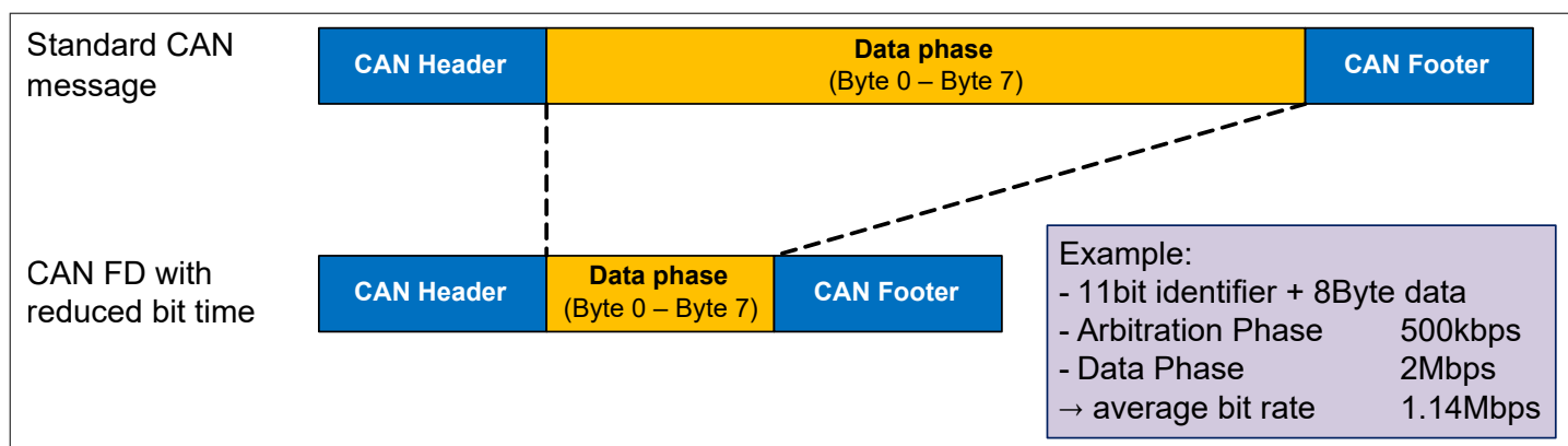
Figure 27 Bite Rate Increase with CAN FD vs. Standard CAN
