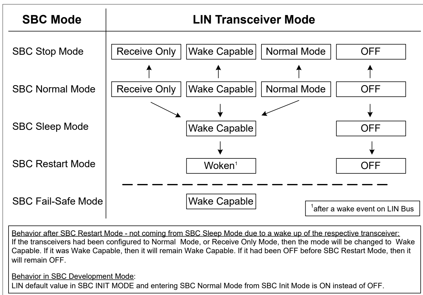
Figure 33 LIN Mode Control Diagram
