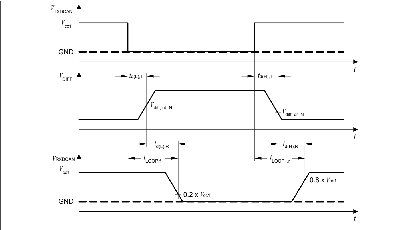
Figure 30 Timing Diagrams for Dynamic Characteristics
