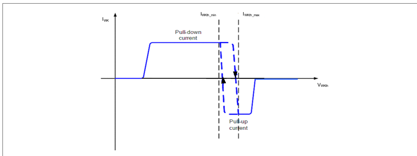
Figure 40 Illustration for Pull-Up / Down Current Sources with Automatic Switching Configuration
