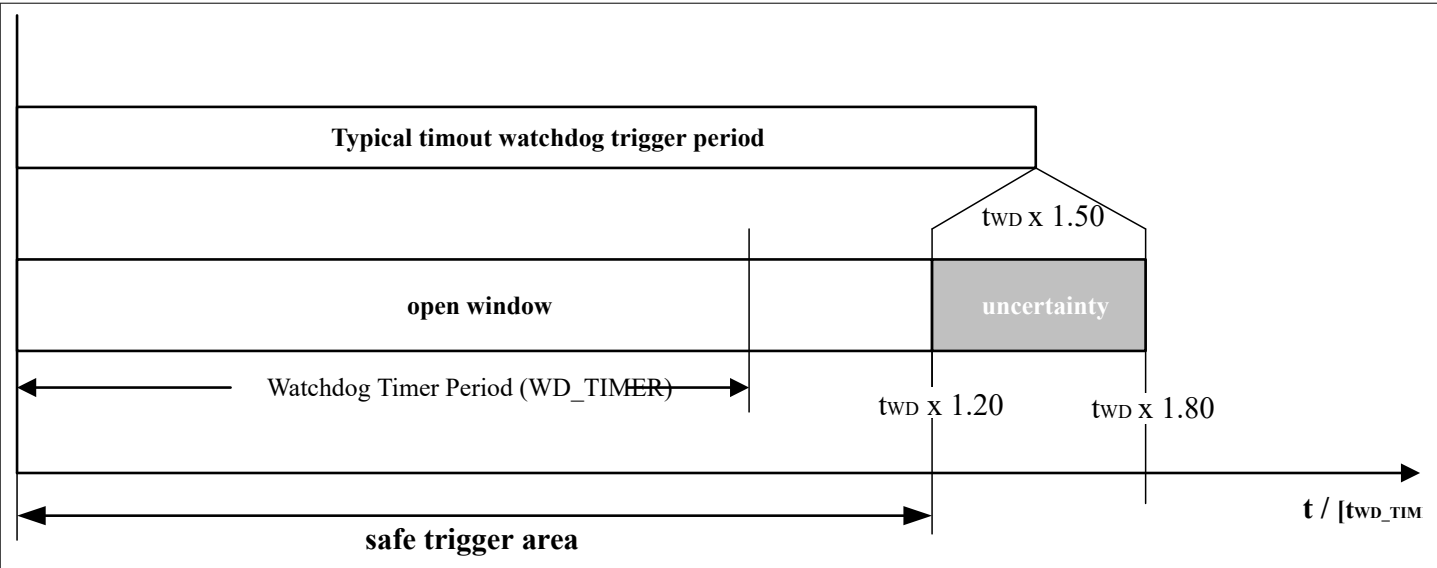
Figure 48 Time-out Watchdog Definition
