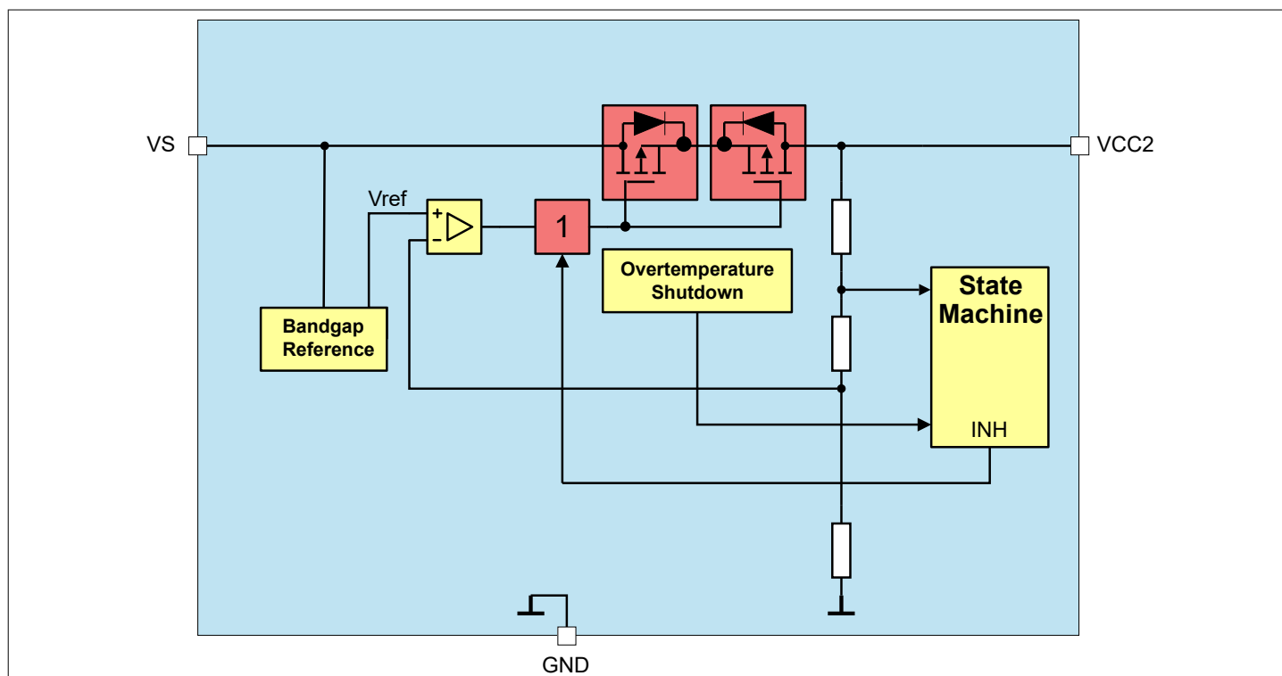
Figure 14 Module Block Diagram
