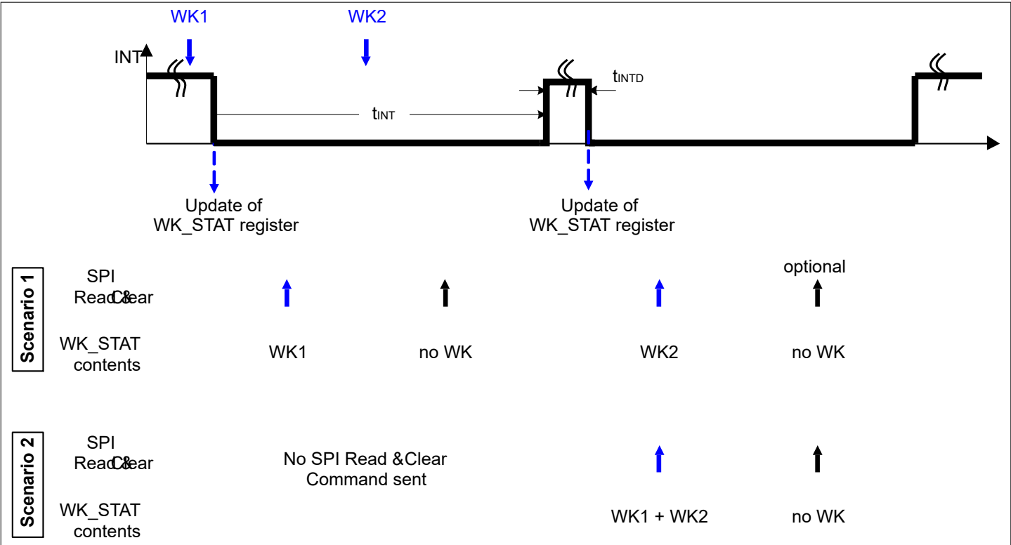
Figure 43 Interrupt Signalization Behavior
