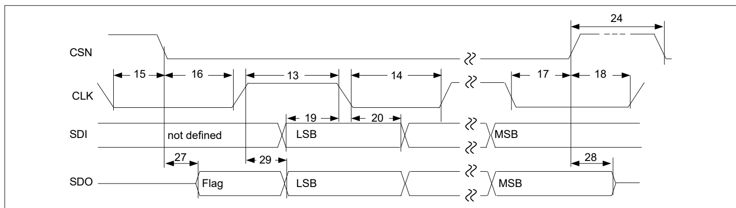
Figure 58 SPI Timing Diagram
