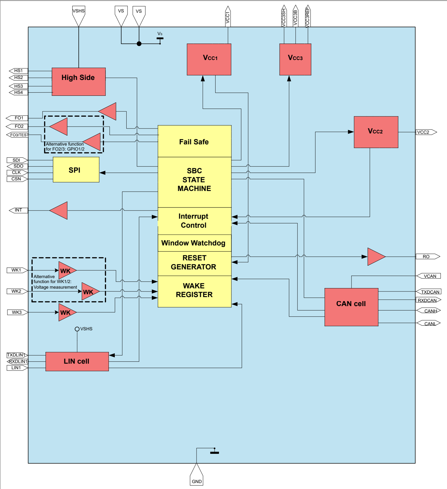
Figure 1 Block Diagram
