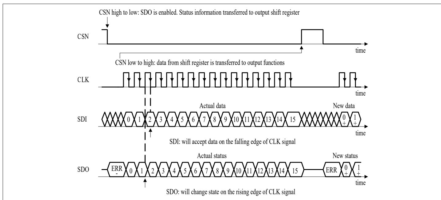
Figure 54 SPI Data Transfer Timing (note the reversed order of LSB and MSB shown in this figure compared to the register description)
