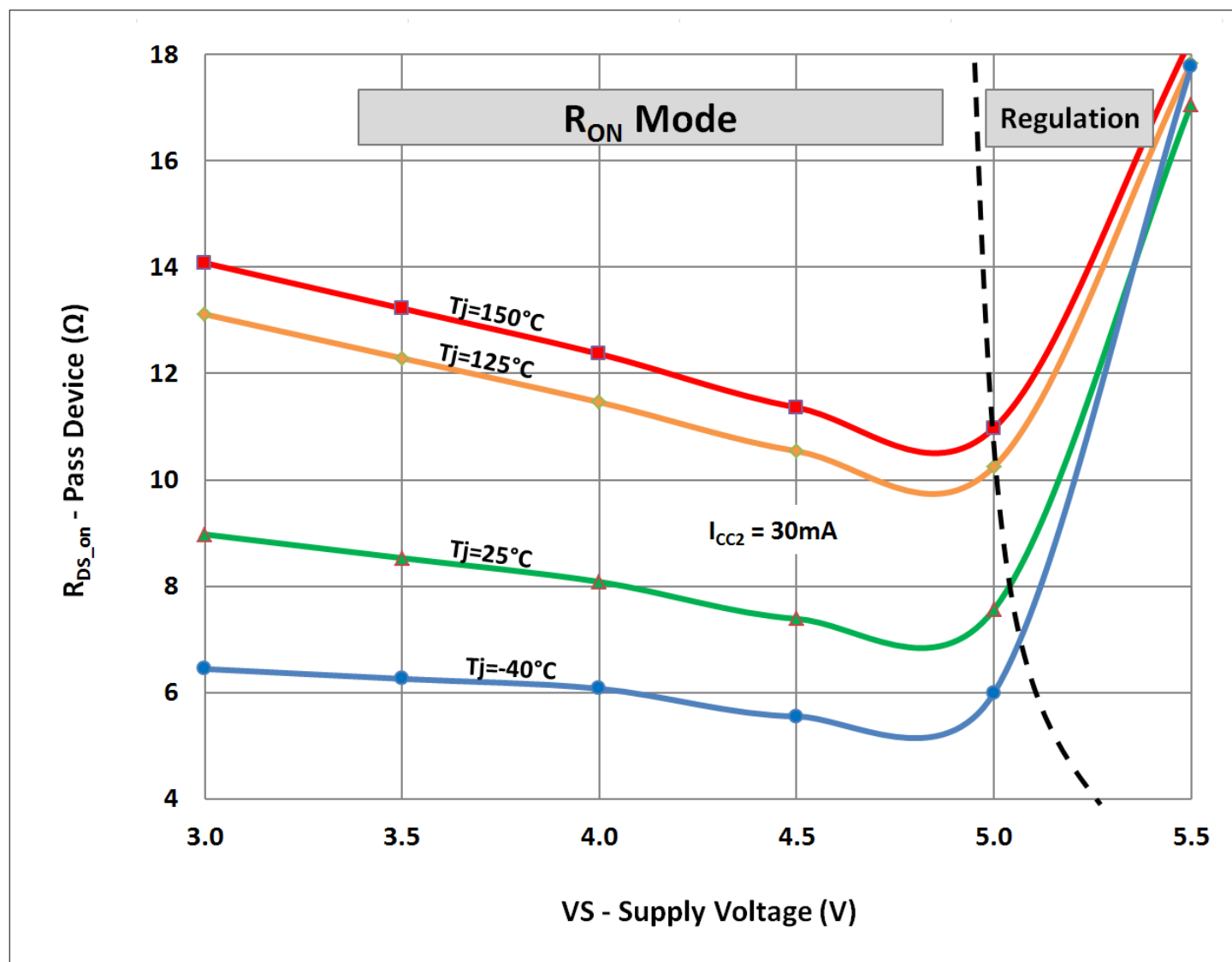
Figure 15 Typical on-resistance of VCC2 pass device during low drop operation for I_{CC2} = 30\text{mA}
