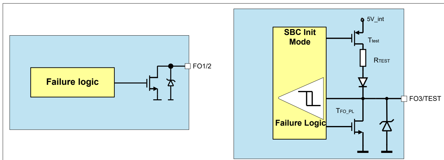
Figure 44 Simplified Fail Output Block Diagram for FO1/2 and for FO3/TEST
