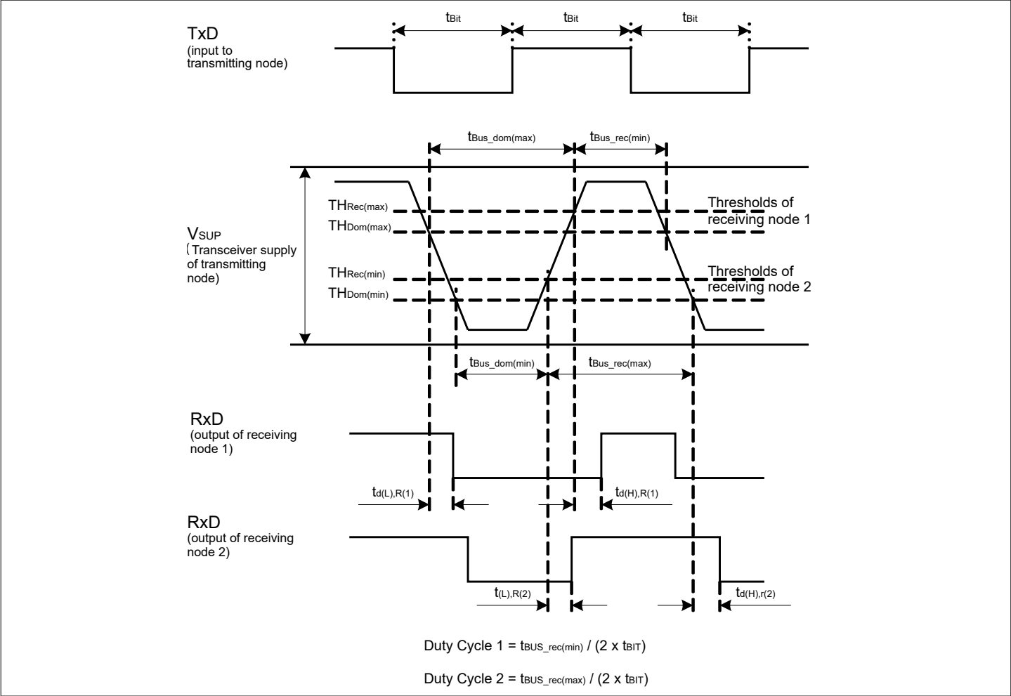
Figure 37 Timing Diagram for Dynamic Characteristics
