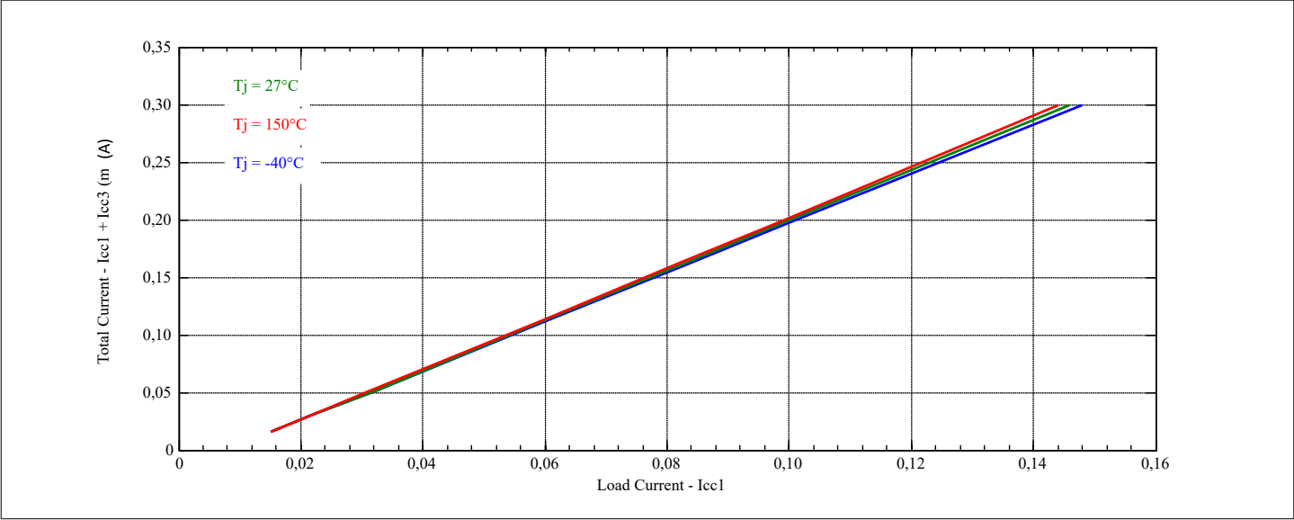
Figure 23 Load Sharing Behavior of ICC1 vs. the total load current
