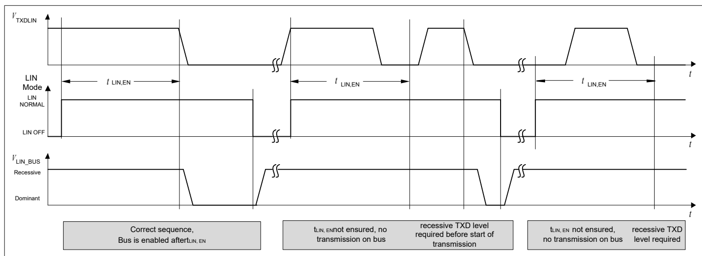
Figure 34 LIN Transceiver Enabling Sequence
