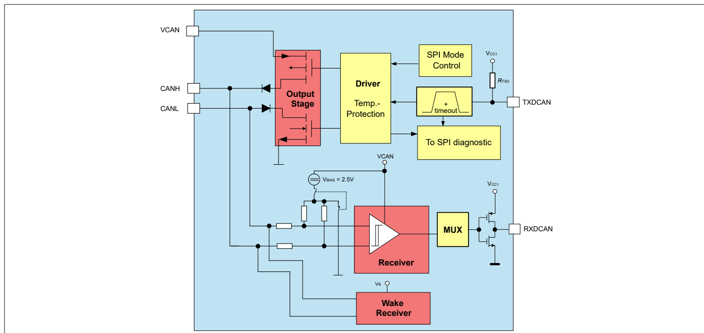
Figure 25 Functional Block Diagram
