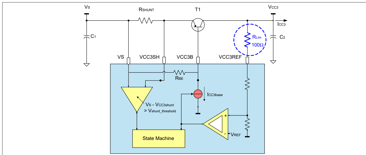
Figure 19 Protecting the VCC3 against inductive short circuits when configured as an independent voltage regulator for off-board supply
