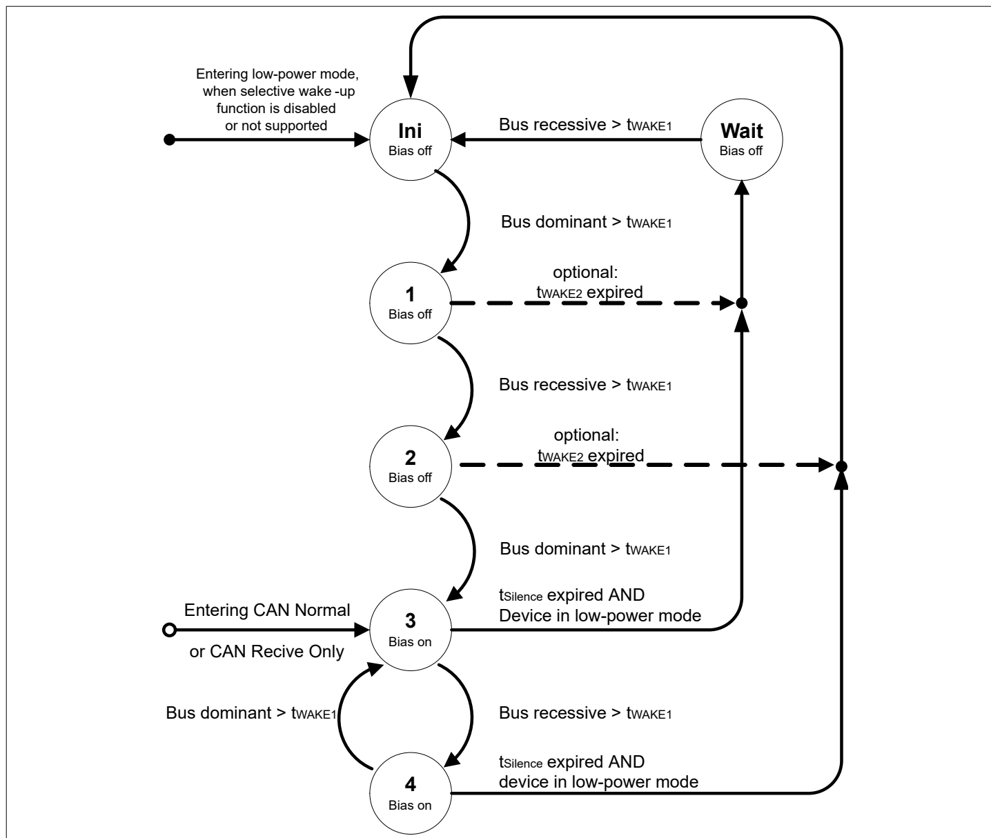
Figure 29 WUP detection following the definition in ISO 11898-2:2016
