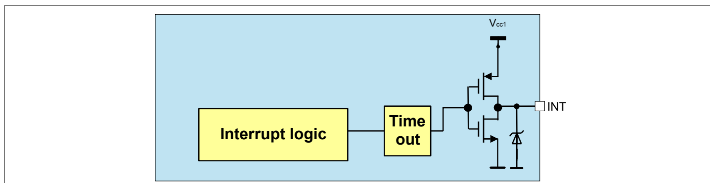
Figure 36 Interrupt Block Diagram
