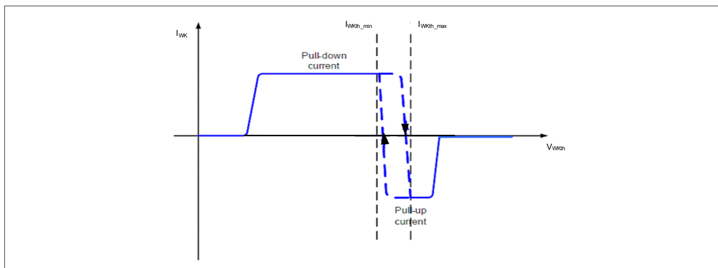
Figure 34 Illustration for Pull-Up / Down Current Sources with Automatic Switching Configuration
