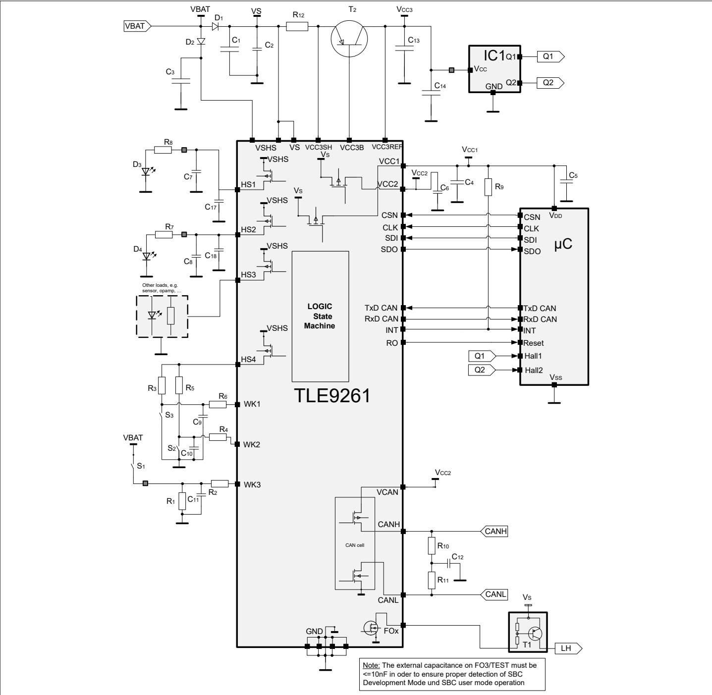
Figure 53 Simplified Application Diagram
