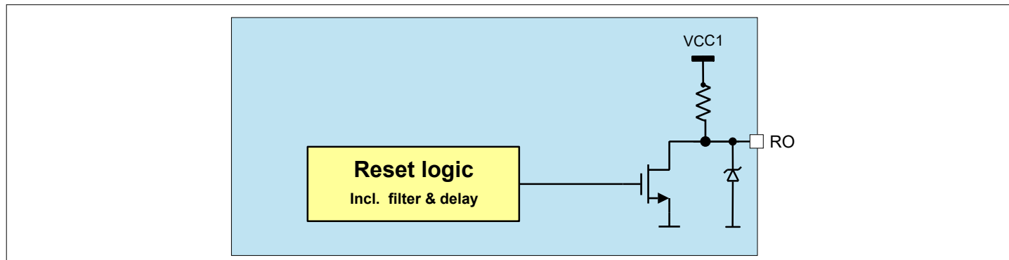
Figure 40 Reset Block Diagram
