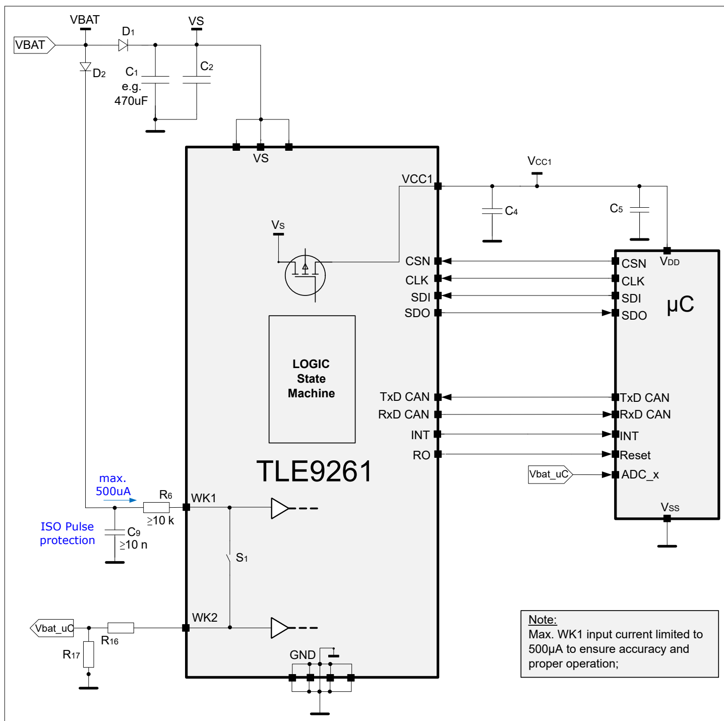
Figure 54 Simplified Application Diagram with the Alternate Measurement Function via WK1 and WK2
