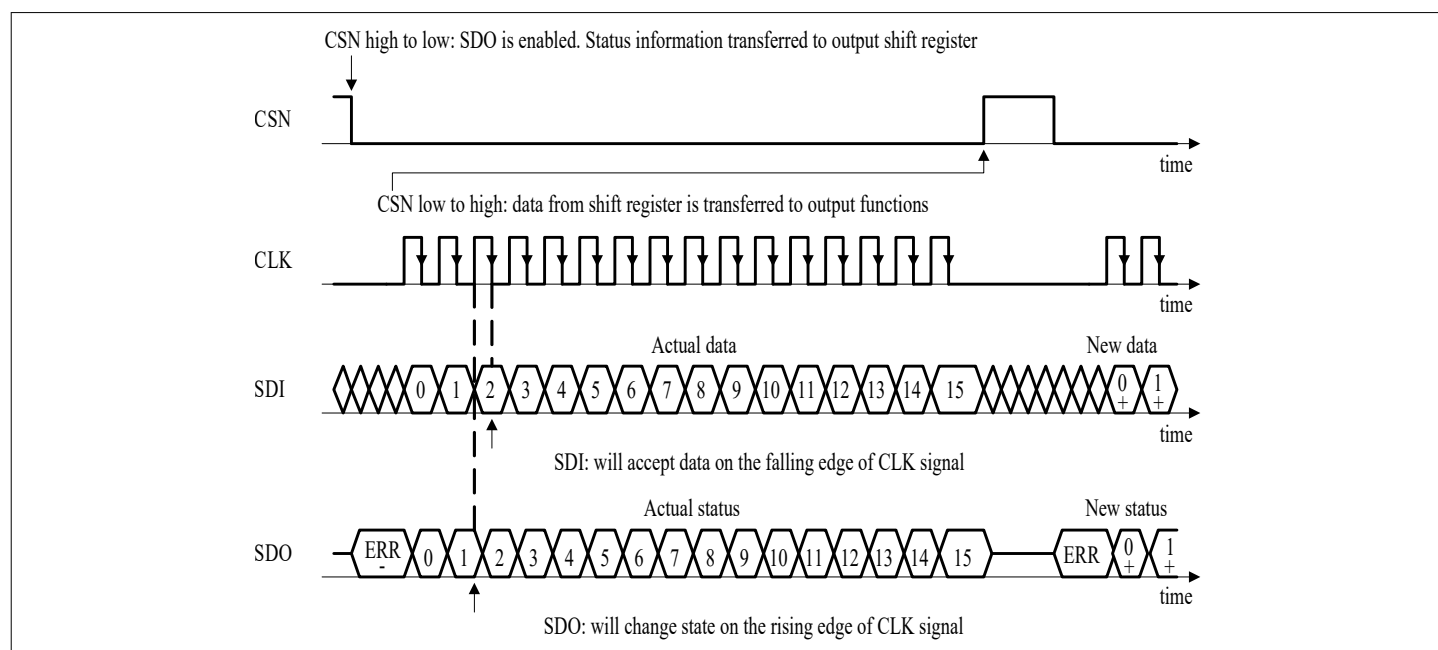
Figure 48 SPI Data Transfer Timing (note the reversed order of LSB and MSB shown in this figure compared to the register description)
