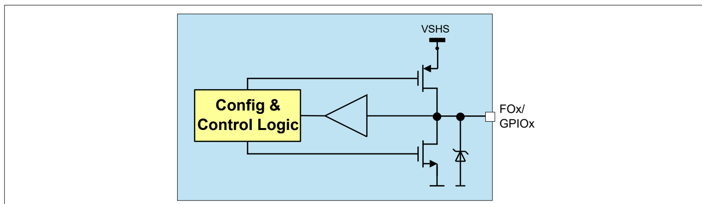
Figure 39 Simplified General Purpose I/O block diagram for FO2 and FO3/TEST
