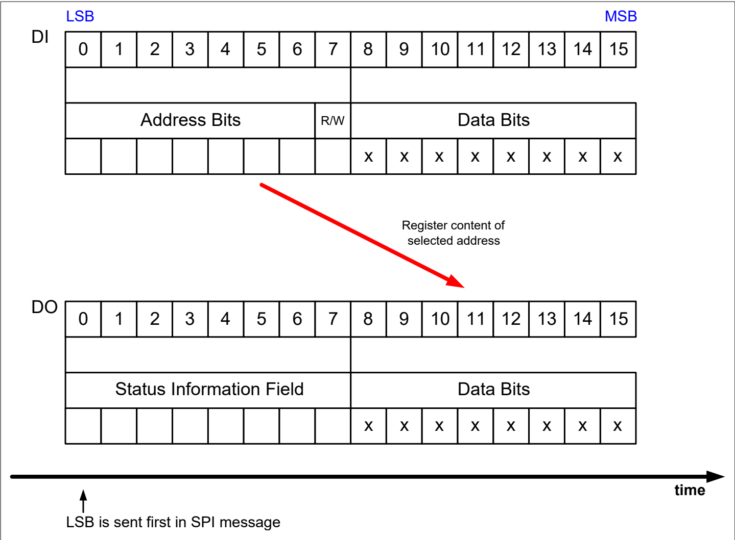
Figure 49 SPI Operation Mode
