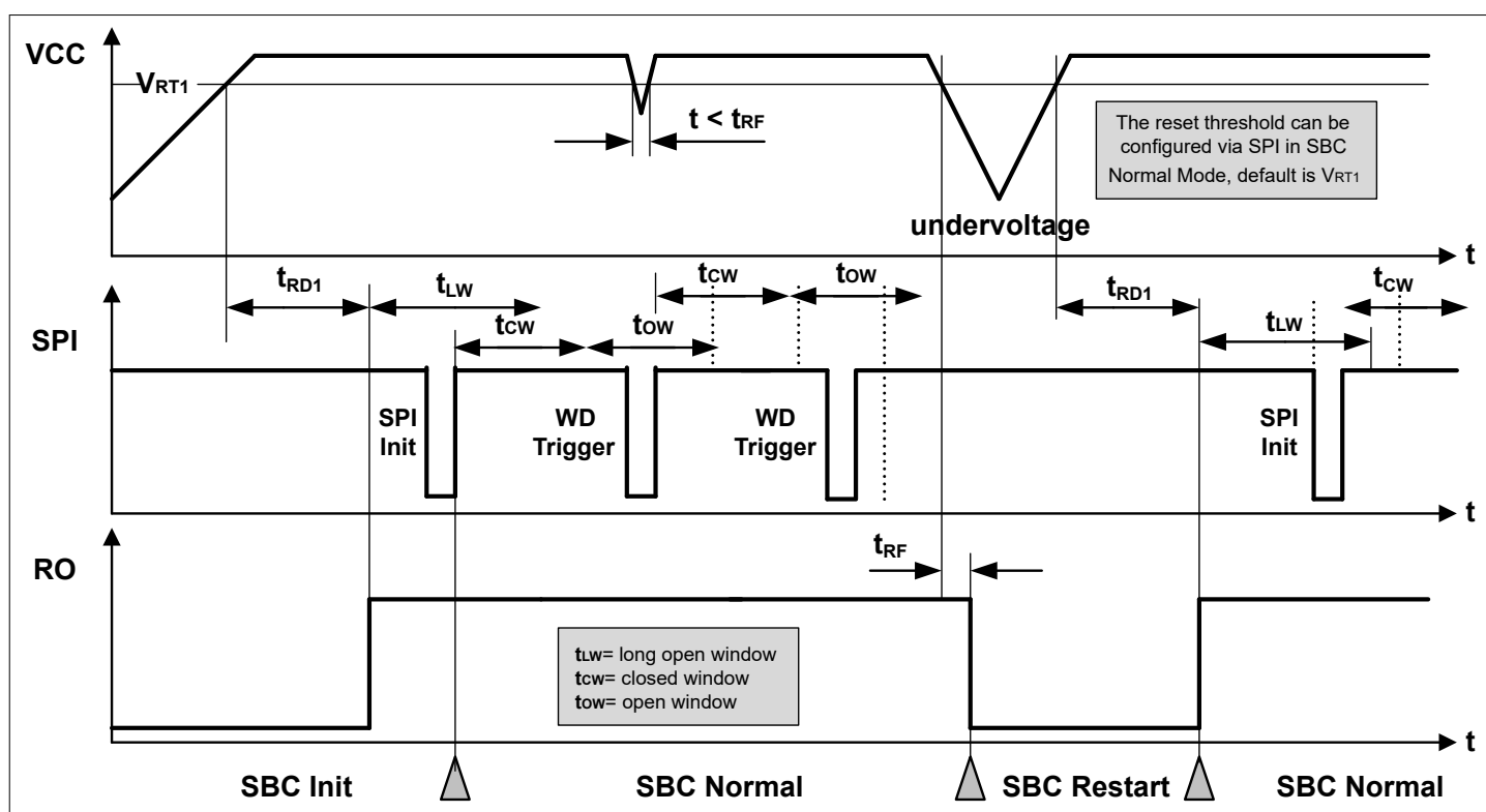
Figure 41 Reset Timing Diagram
