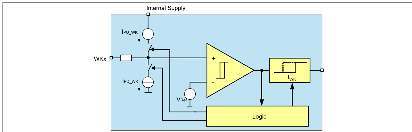
Figure 32 Wake Input Block Diagram
