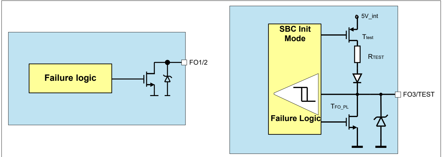
Figure 38 Simplified Fail Output Block Diagram for FO1/2 and for FO3/TEST
