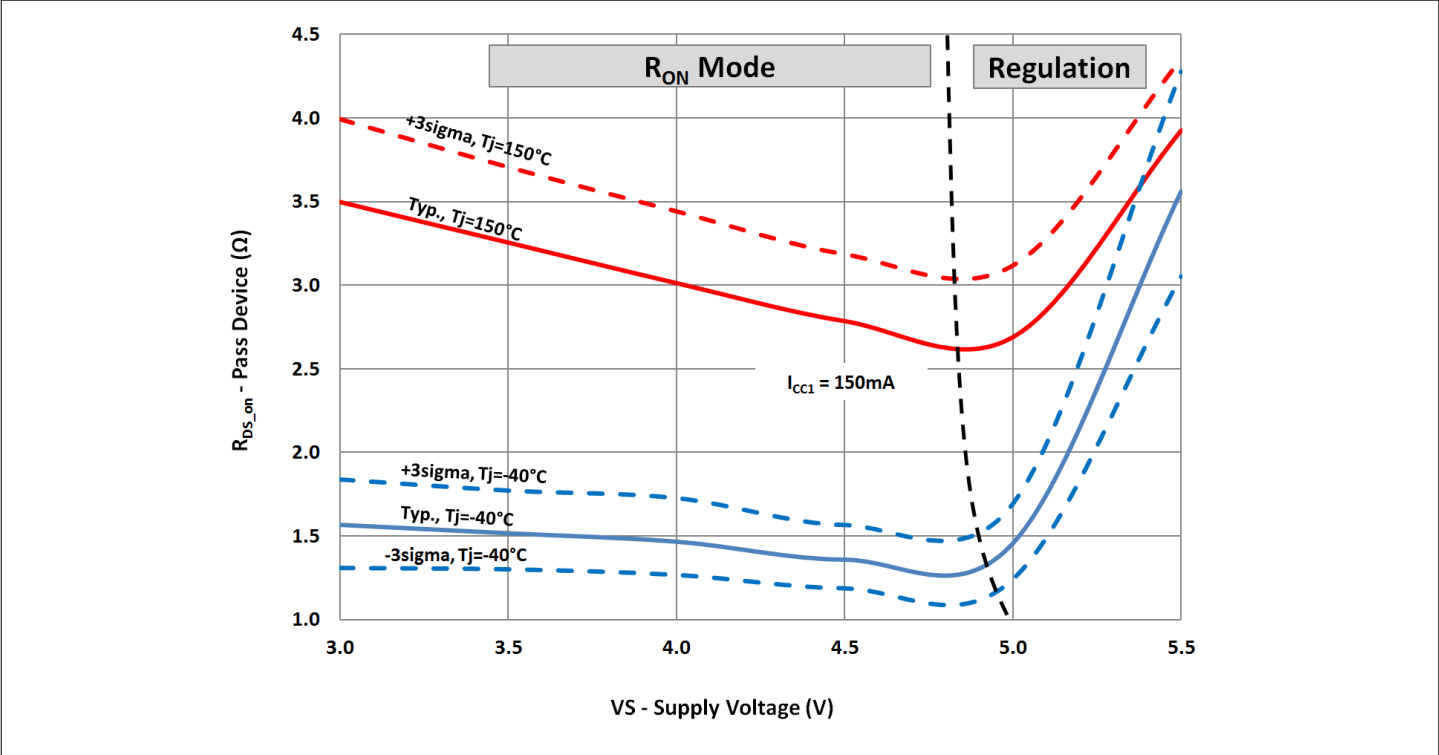
Figure 18 On-resistance range of VCC1 pass device during low drop operation for I_{CC1} = 150\text{mA}
