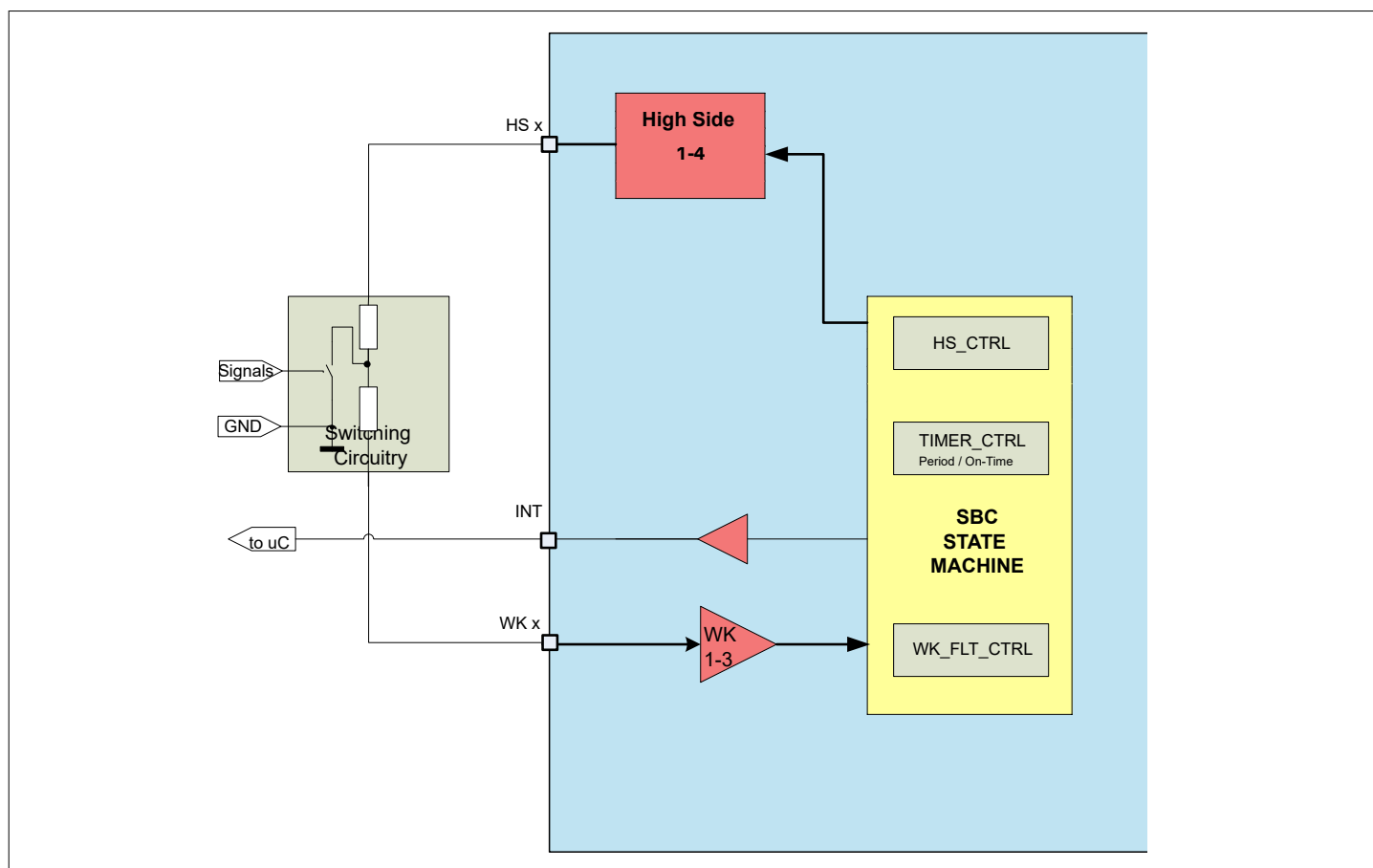
Figure 5 Cyclic Sense Working Principle
