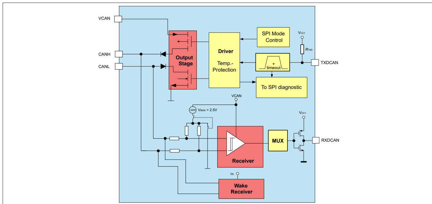
Figure 30 Functional Block Diagram
