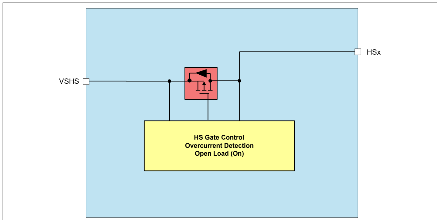
Figure 29 High-Side Module Block Diagram
