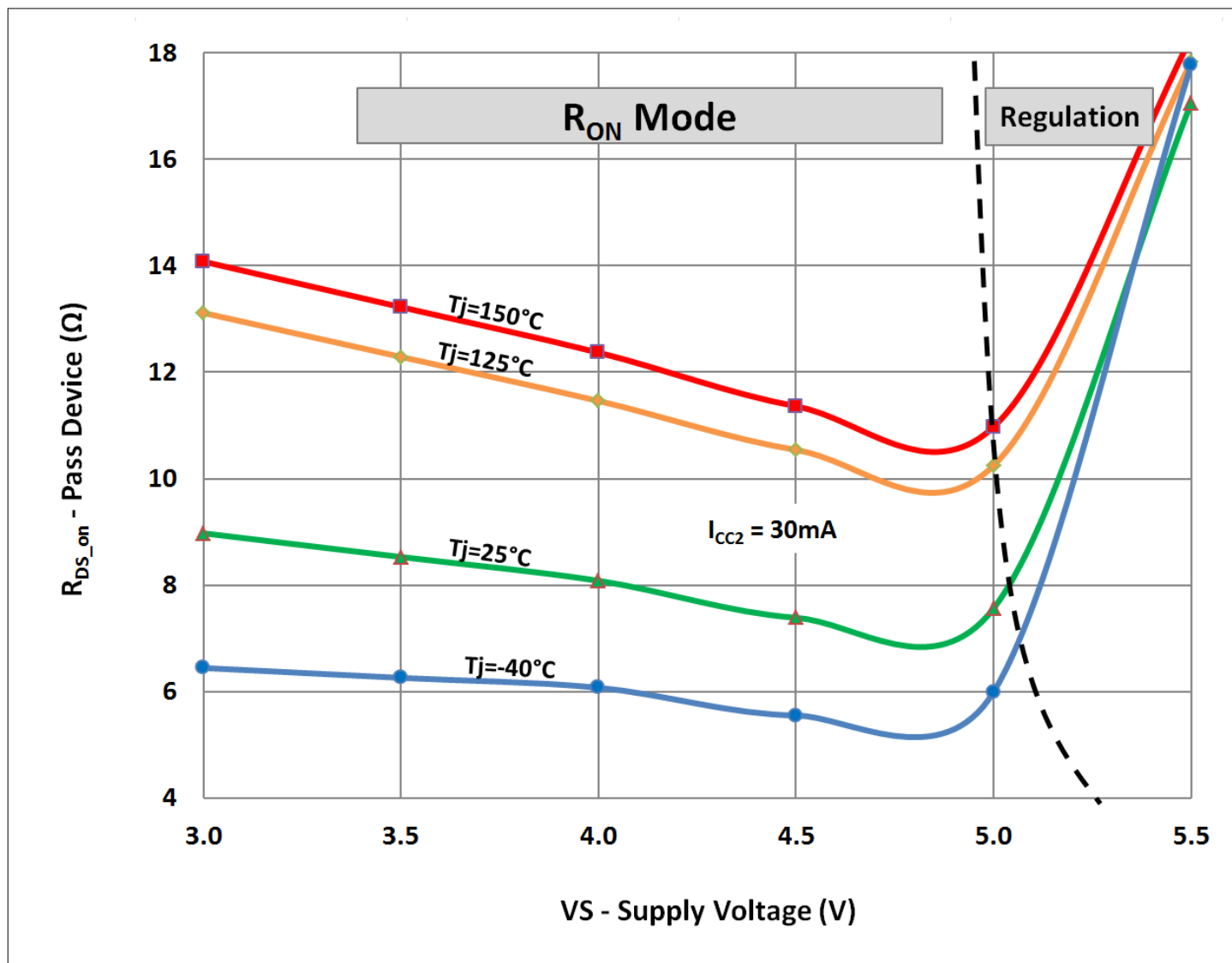
Figure 20 Typical on-resistance of VCC2 pass device during low drop operation for I_{CC2} = 30mA
