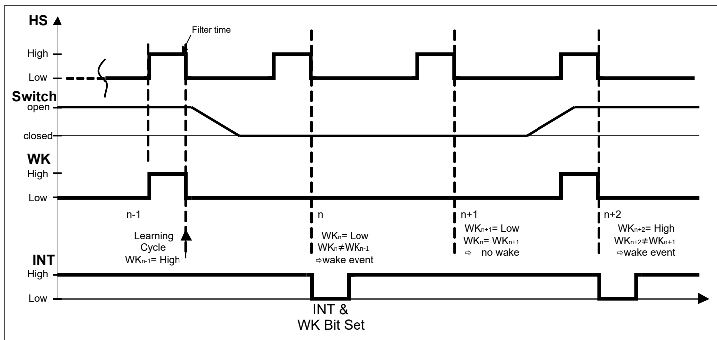
Figure 8 Cyclic Sense Example in SBC Stop Mode, HSx starts "OFF"/LOW, GND based WKx input
