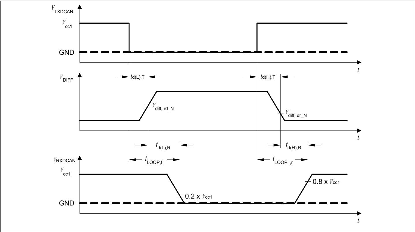
Figure 35 Timing Diagrams for Dynamic Characteristics
