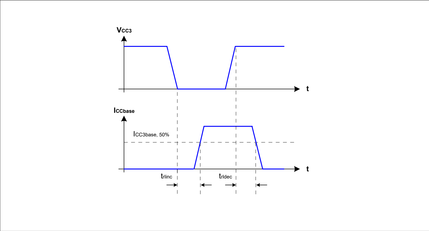
Figure 26 Regulator Reaction Time
