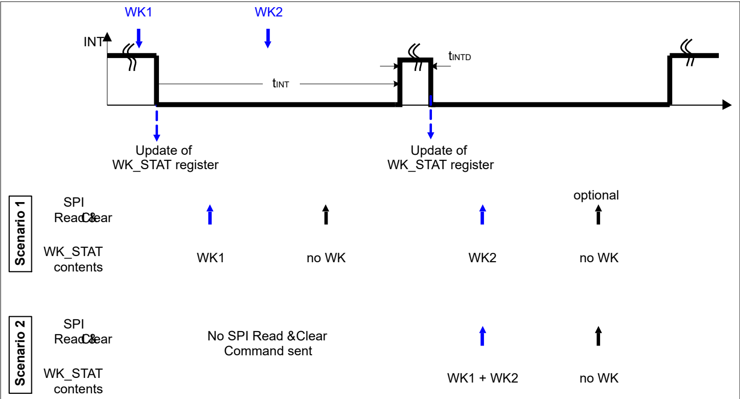
Figure 42 Interrupt Signalization Behavior
