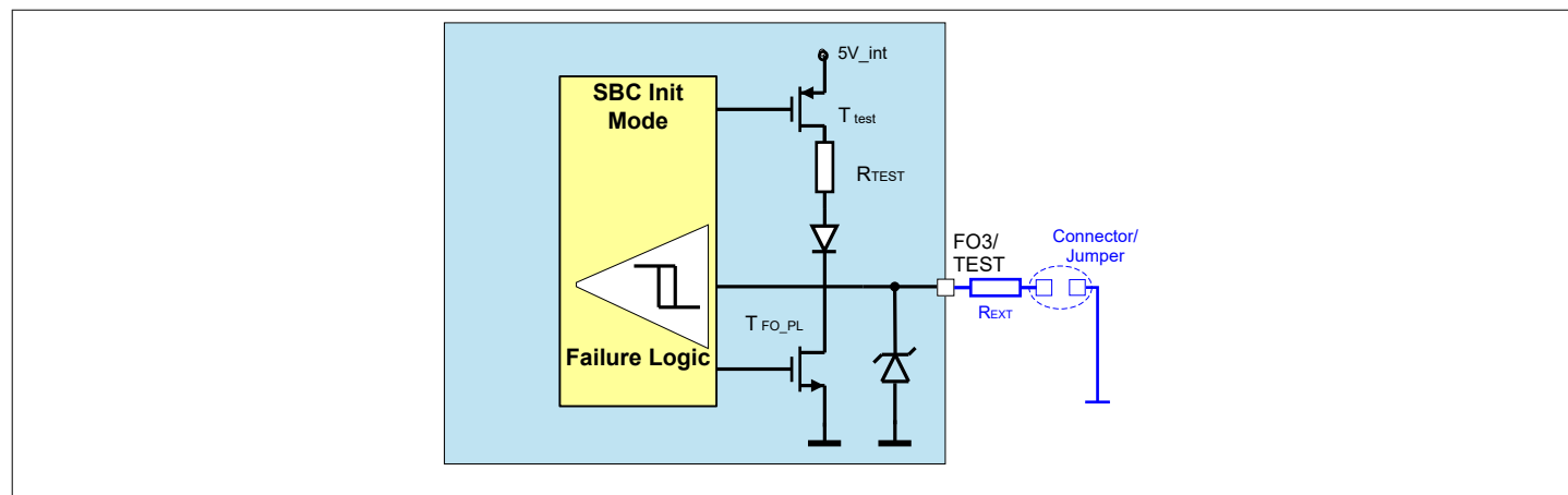
Figure 60 Hint for Increasing the Robustness of pin FO3/TEST during Debugging or Programming
