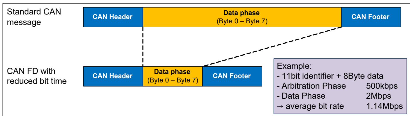
Figure 32 Bite Rate Increase with CAN FD vs. Standard CAN
