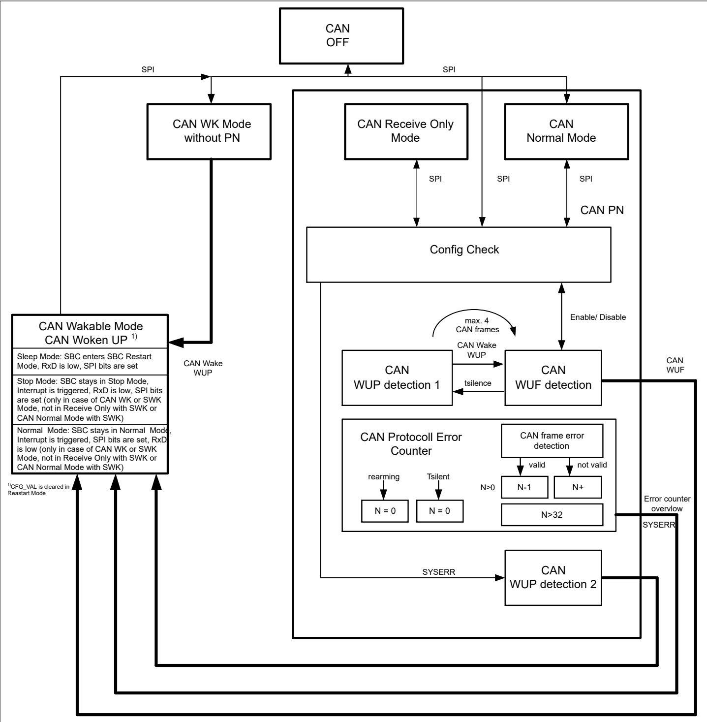
Figure 11 CAN Selective Wake State Diagram
