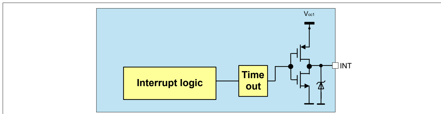
Figure 41 Interrupt Block Diagram
