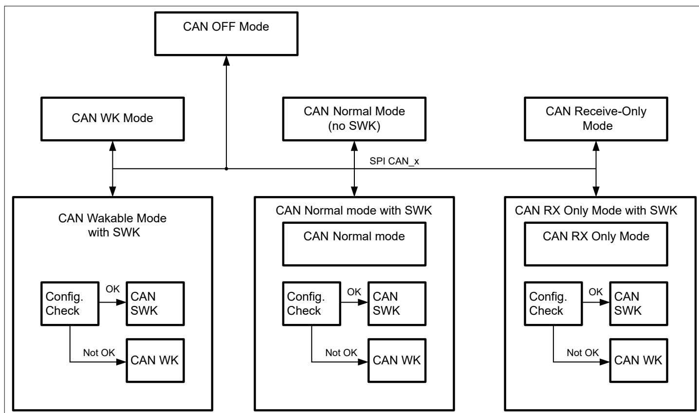
Figure 14 CAN SWK State Diagram
