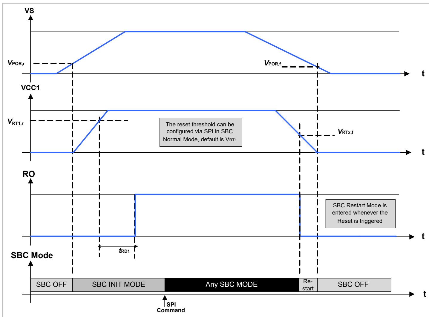
Figure 50 Ramp up / down example of Supply Voltage
