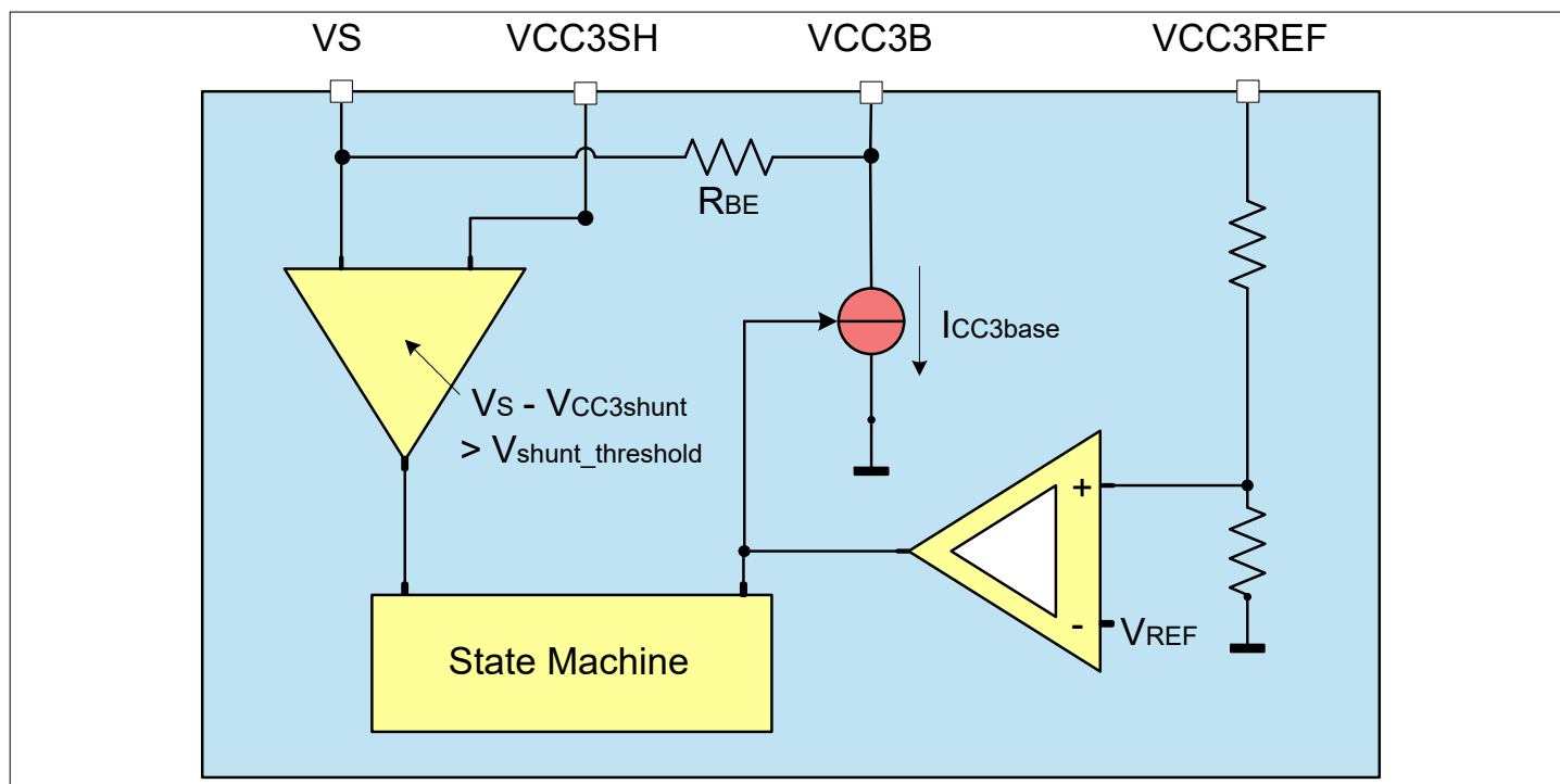
Figure 22 Functional Block Diagram
