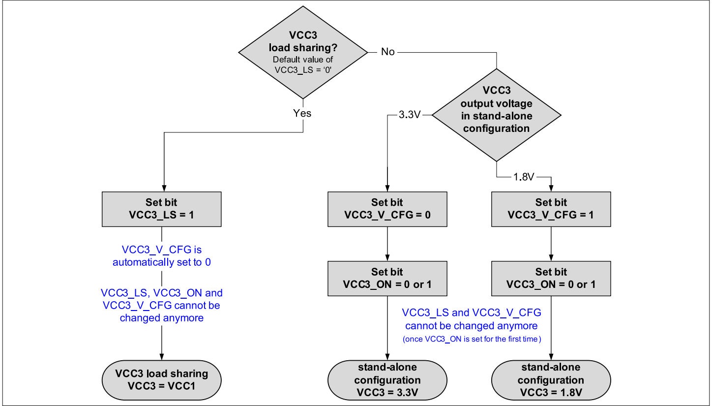
Figure 23 Selecting the Configuration of the VCC3 Regulator
