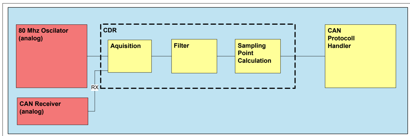
Figure 15 Clock and Data Recovery Block Diagram
