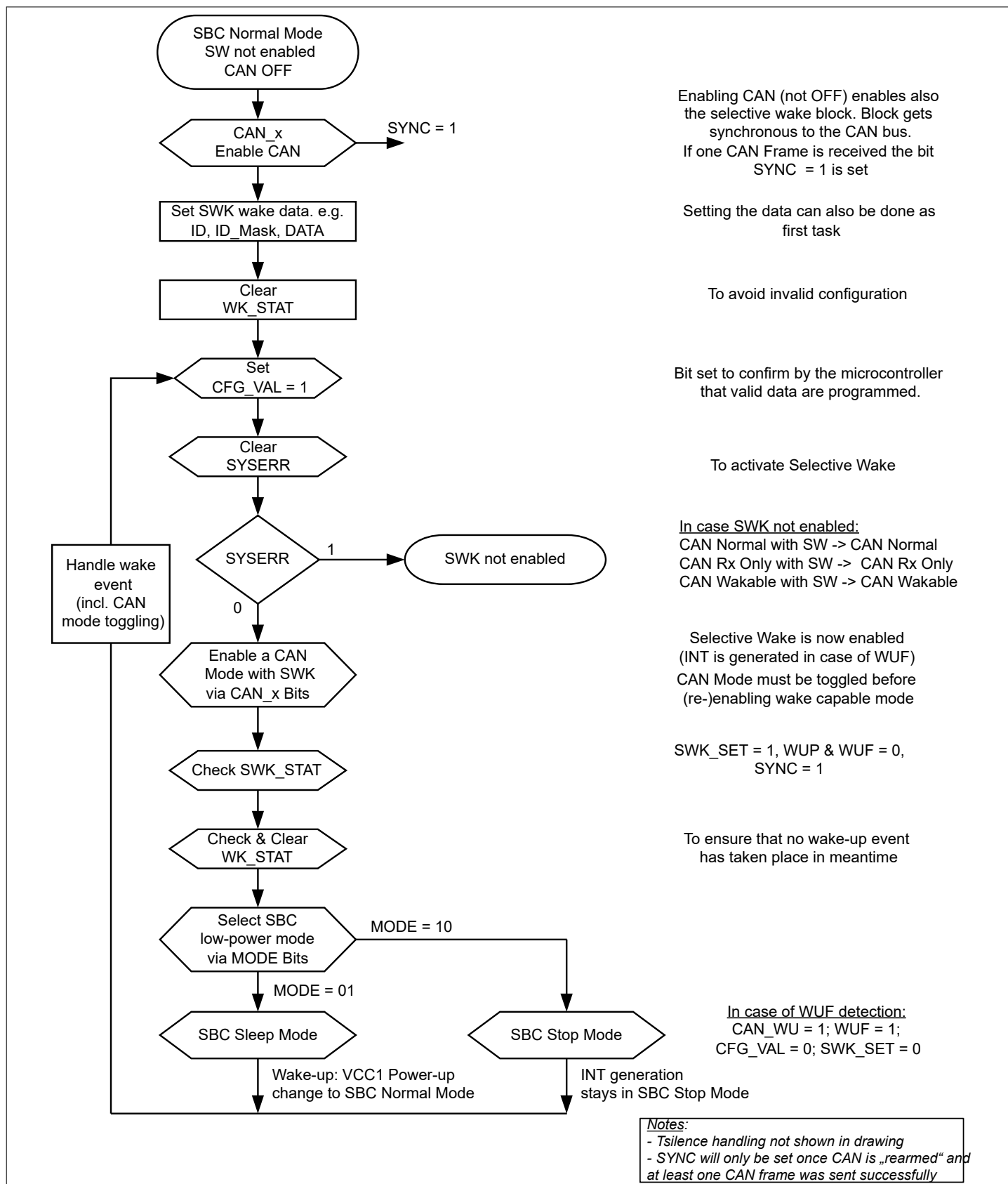
Figure 12 Flow for activation of SWK
