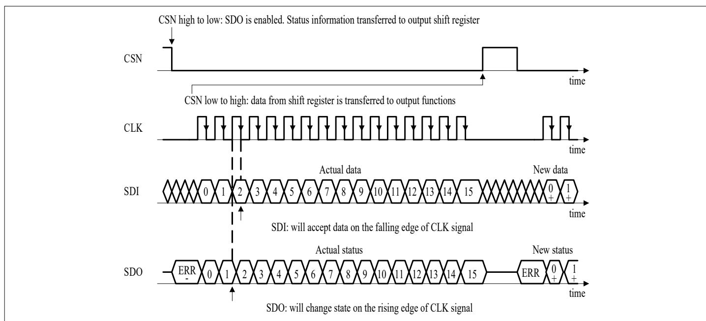
Figure 53 SPI Data Transfer Timing (note the reversed order of LSB and MSB shown in this figure compared to the register description)
