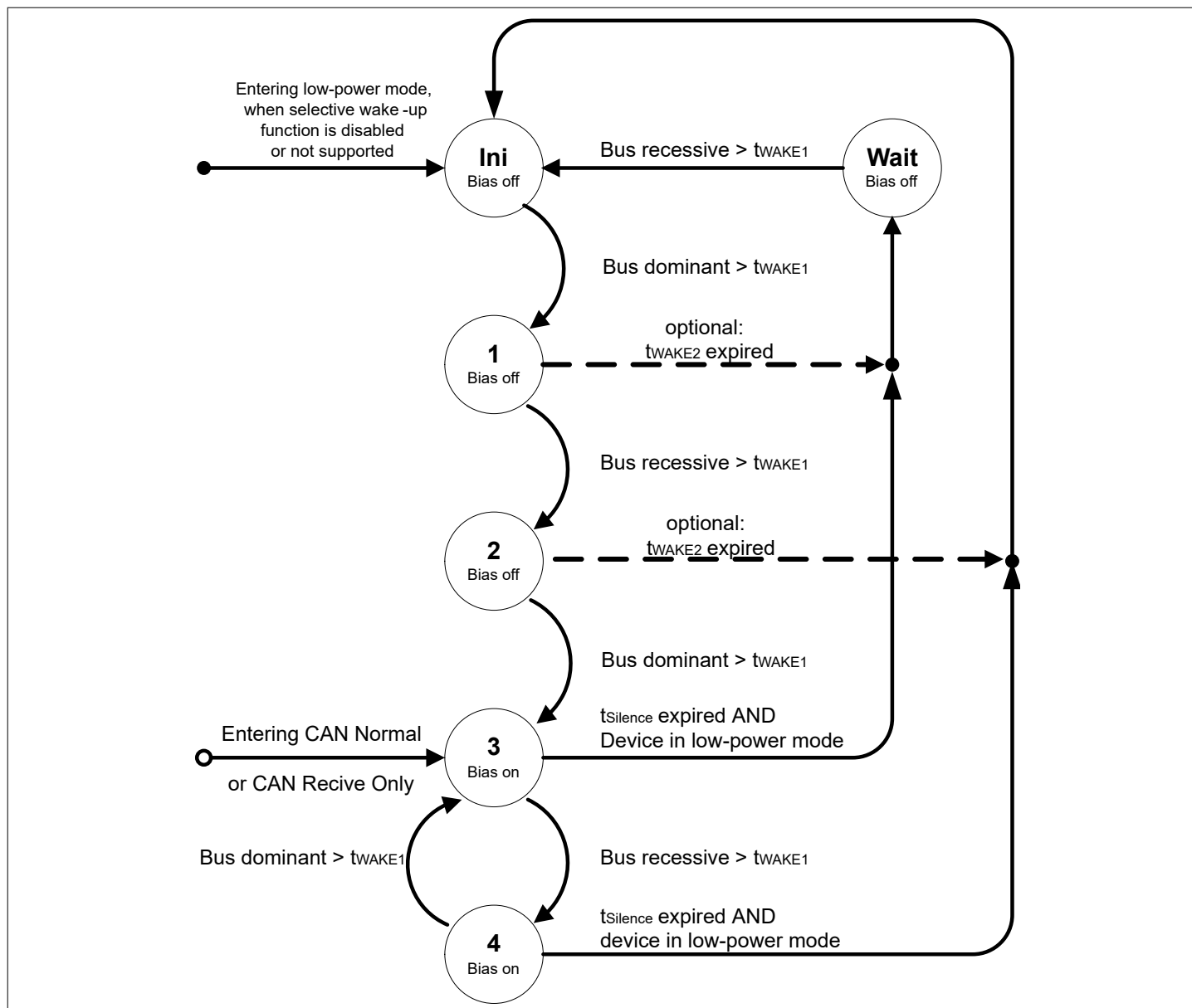
Figure 34 WUP detection following the definition in ISO 11898-2:2016
