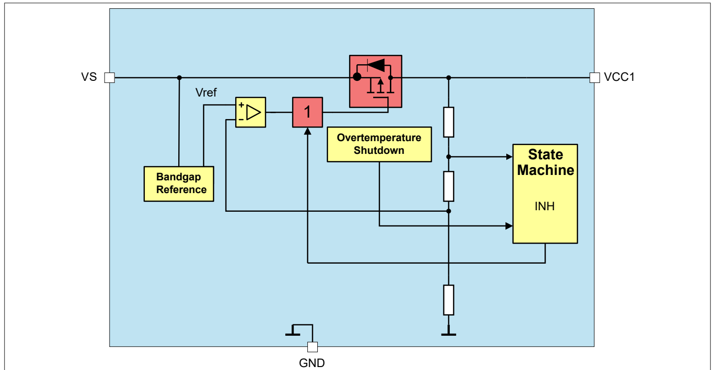
Figure 16 Module Block Diagram
