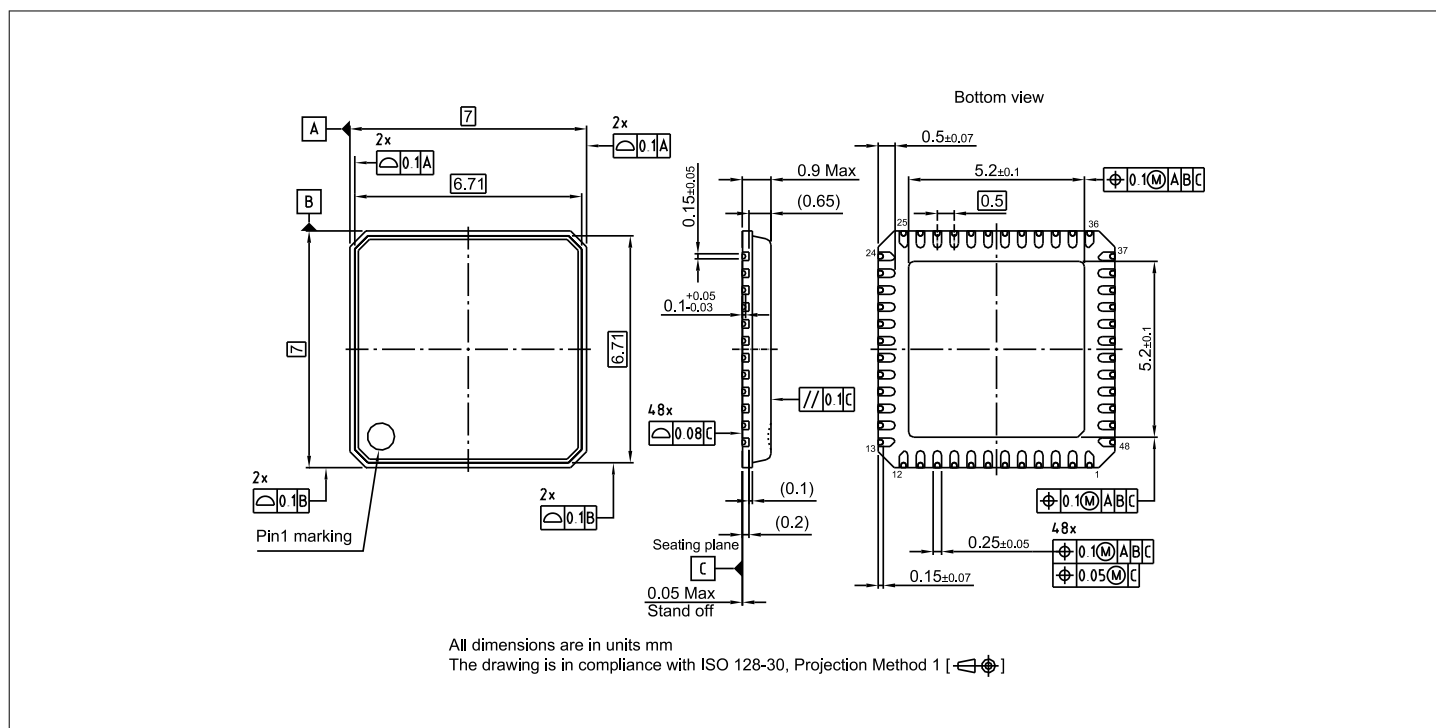
Figure 64 PG-VQFN-48
