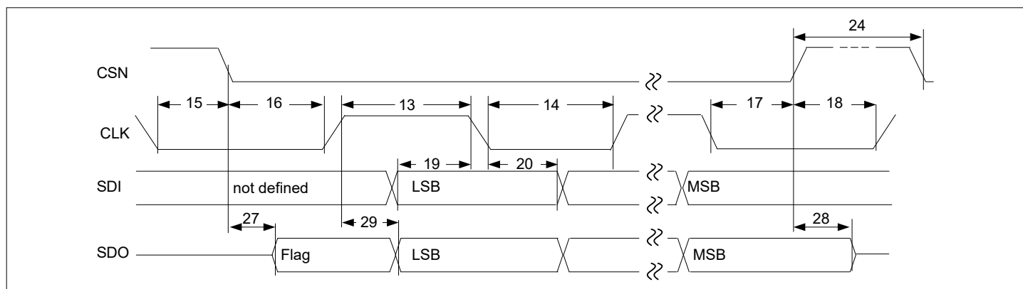
Figure 57 SPI Timing Diagram
