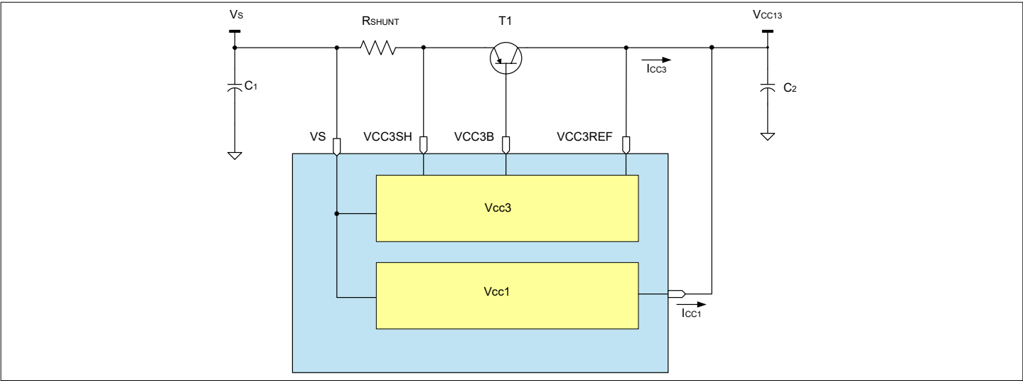
Figure 25 VCC3 in Load Sharing Configuration
