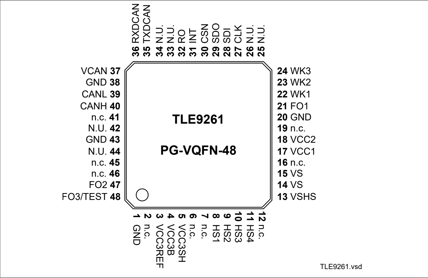
Figure 2 Pin Configuration
