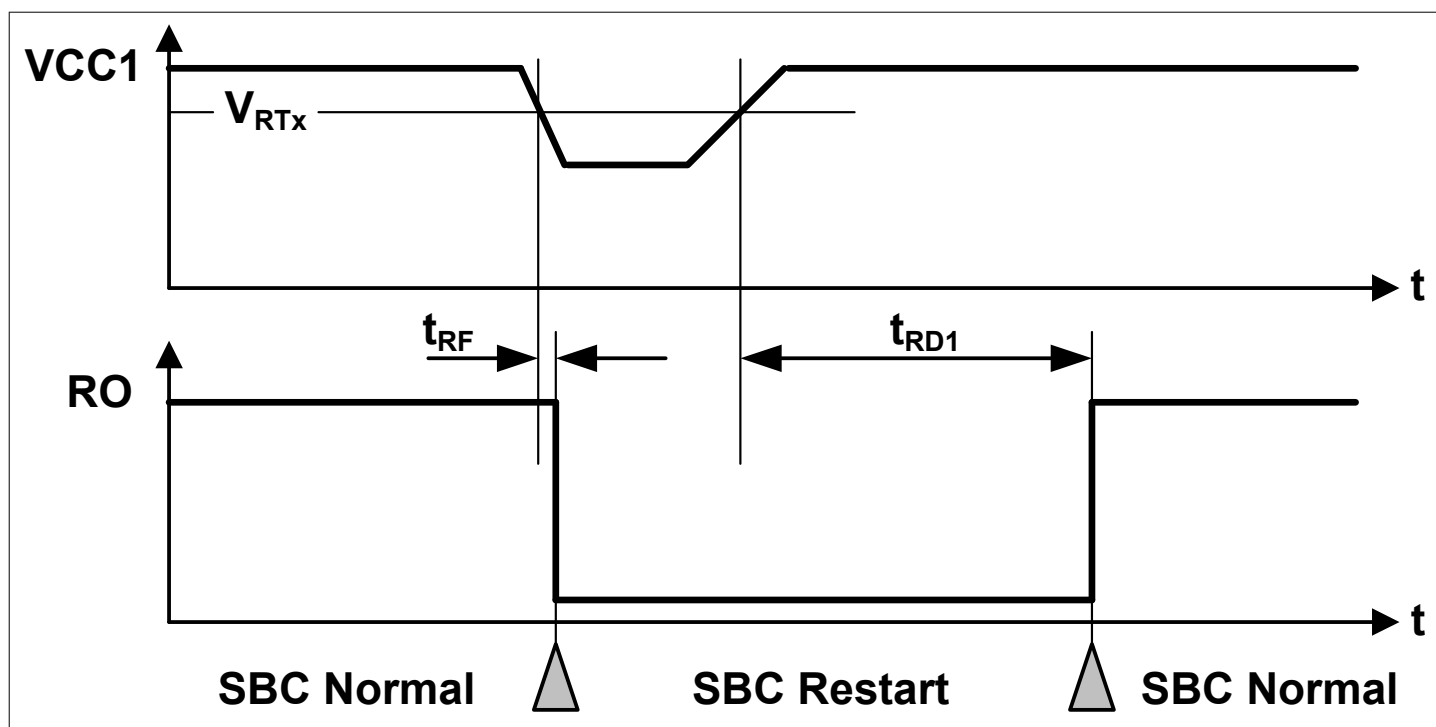
Figure 51 VCC1 Undervoltage Timing Diagram
