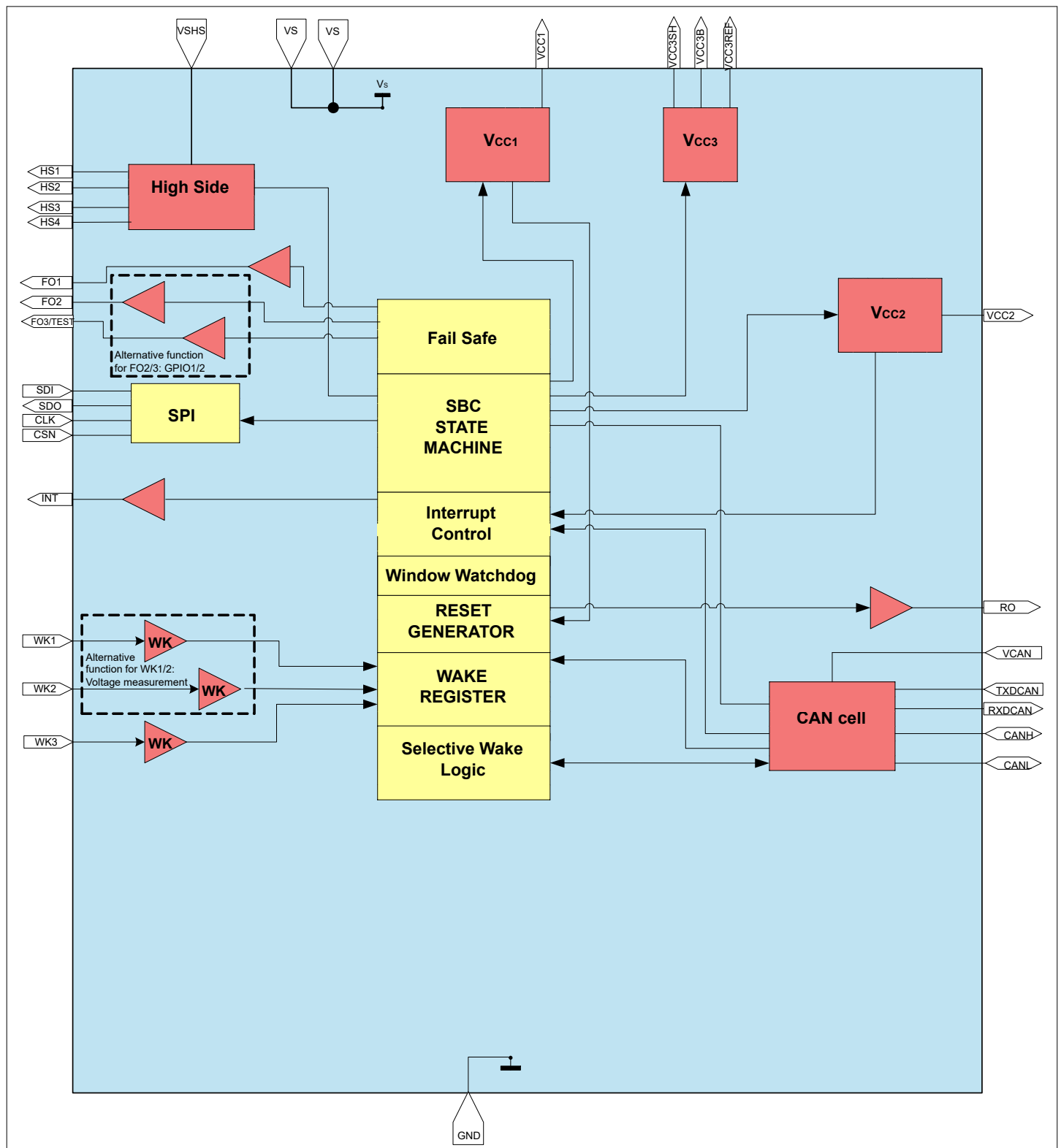
Figure 1 Block Diagram with CAN Partial Networking
