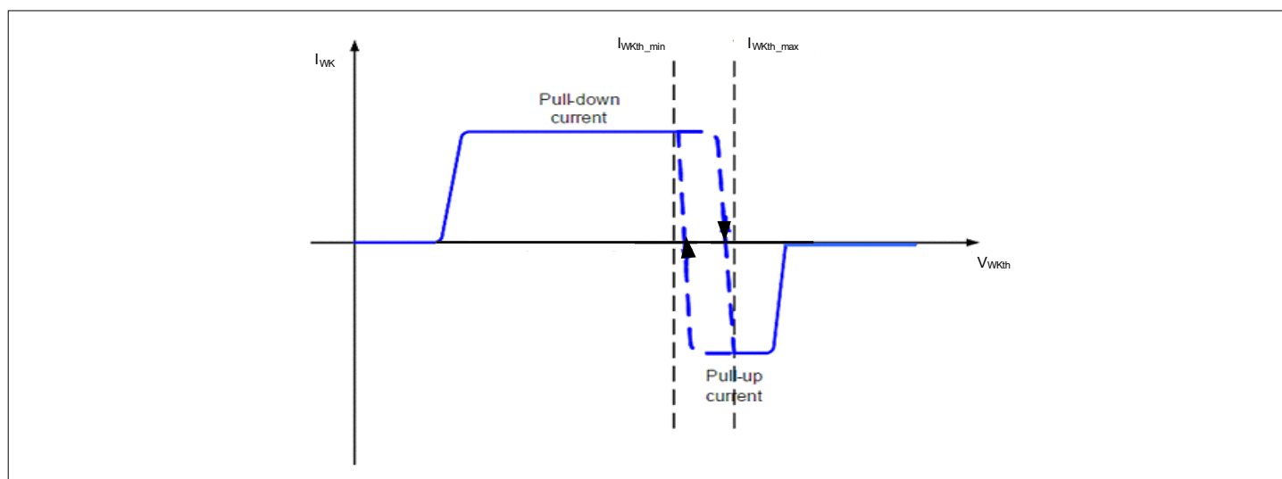
Figure 39 Illustration for Pull-Up / Down Current Sources with Automatic Switching Configuration
