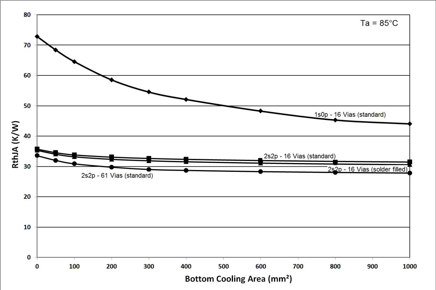
Figure 61 Thermal Resistance ( R_{th\_JA} ) vs. Cooling Area
