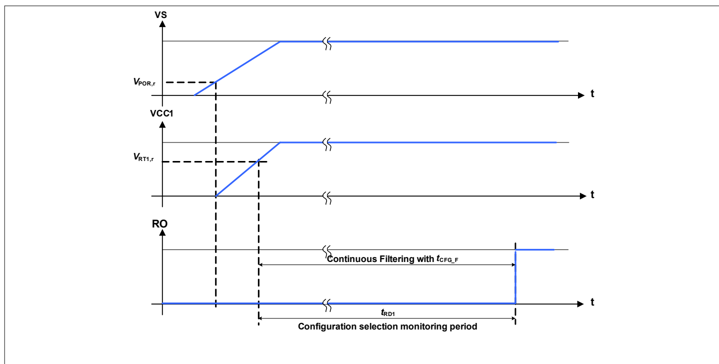
Figure 4 Hardware Configuration Selection Timing Diagram
