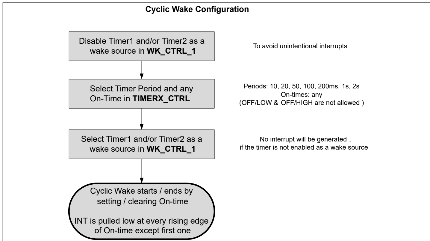
Figure 10 Cyclic Wake: Configuration and Sequence
