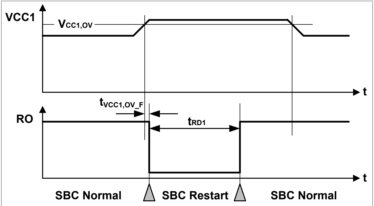
Figure 52 VCC1 Overvoltage Timing Diagram
