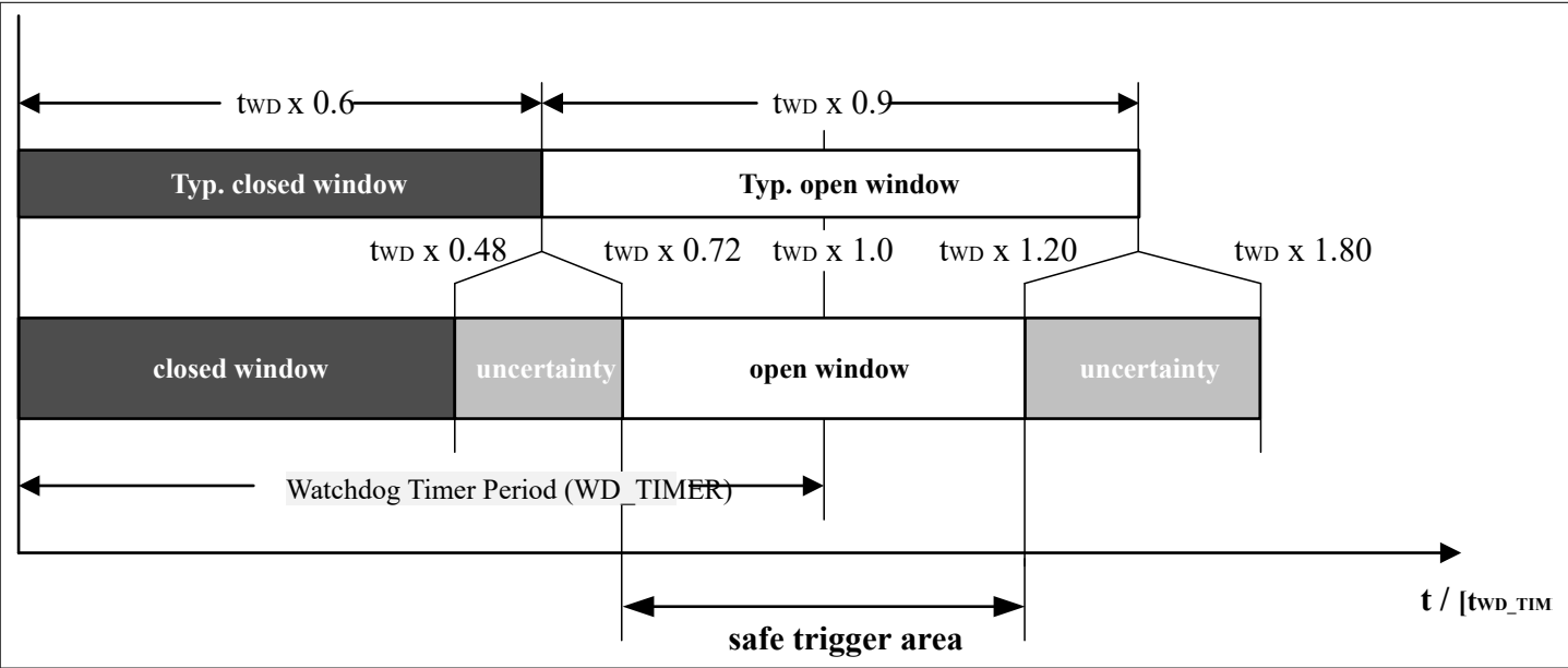
Figure 48 Window Watchdog Definition
