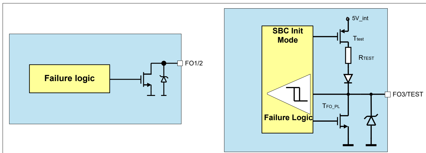
Figure 43 Simplified Fail Output Block Diagram for FO1/2 and for FO3/TEST
