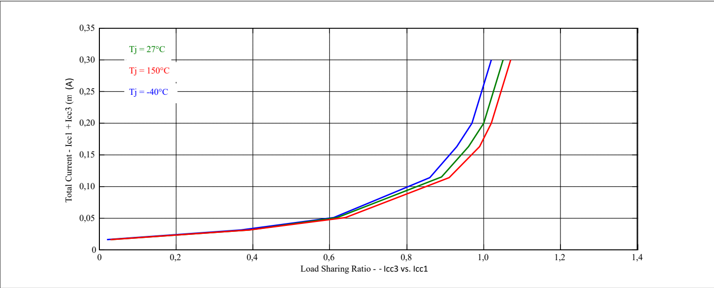
Figure 27 Load Sharing Ratio ICC1 : ICC3 vs. the total load current
