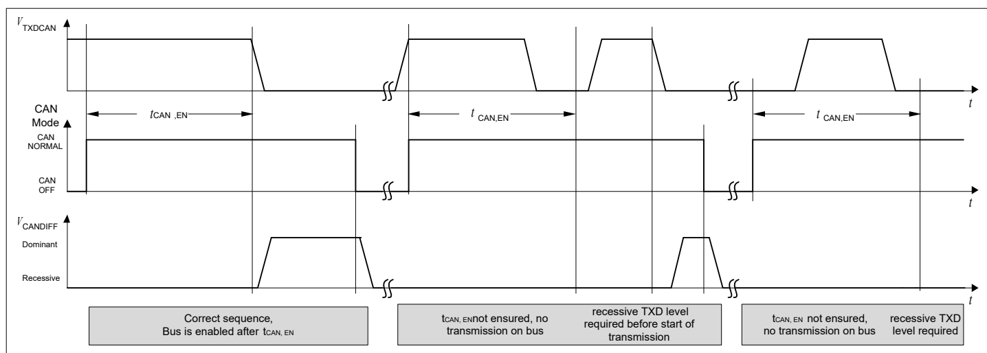
Figure 33 CAN Transceiver Enabling Sequence
