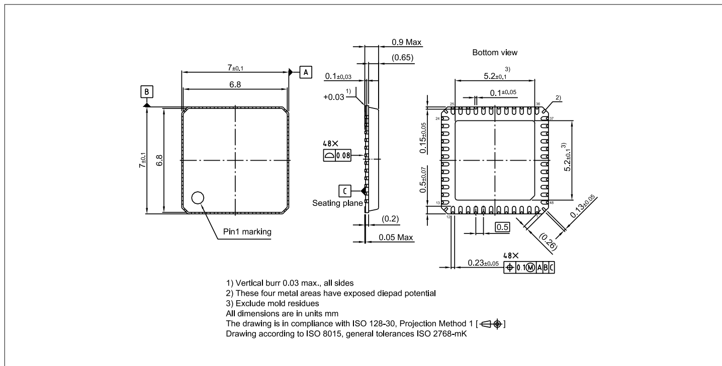
Figure 63 PG-VQFN-48
