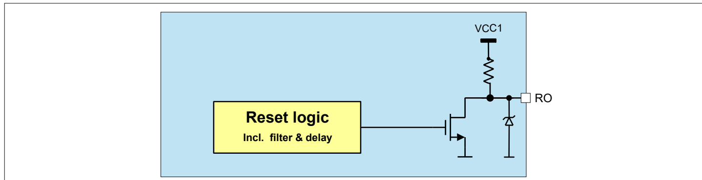
Figure 45 Reset Block Diagram
