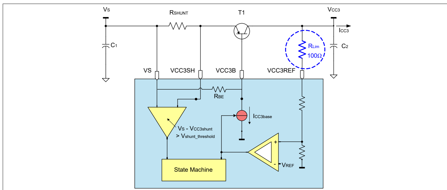
Figure 24 Protecting the VCC3 against inductive short circuits when configured as an independent voltage regulator for off-board supply
