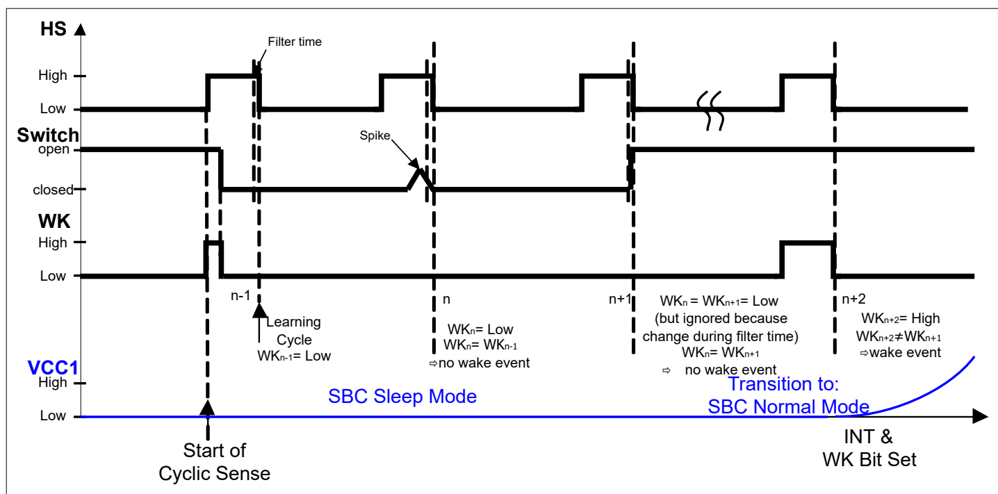
Figure 9 Cyclic Sense Example in SBC Sleep Mode, HSx starts “OFF”/HIGH, GND based WKx input
