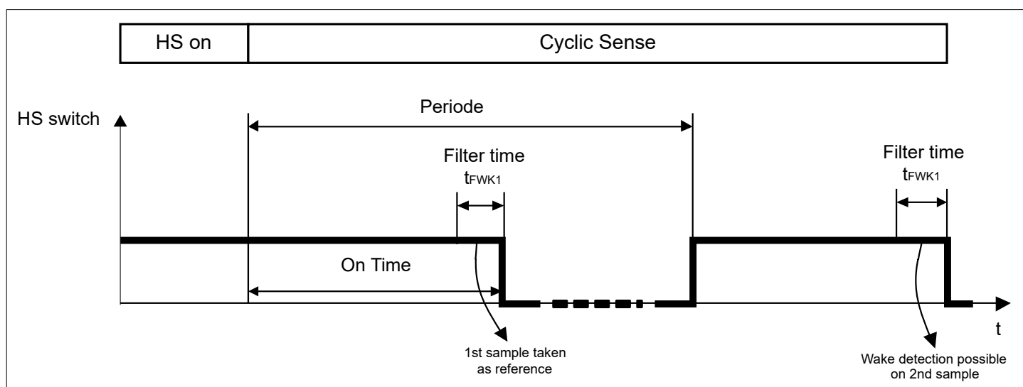
Figure 7 Wake Input Timing
