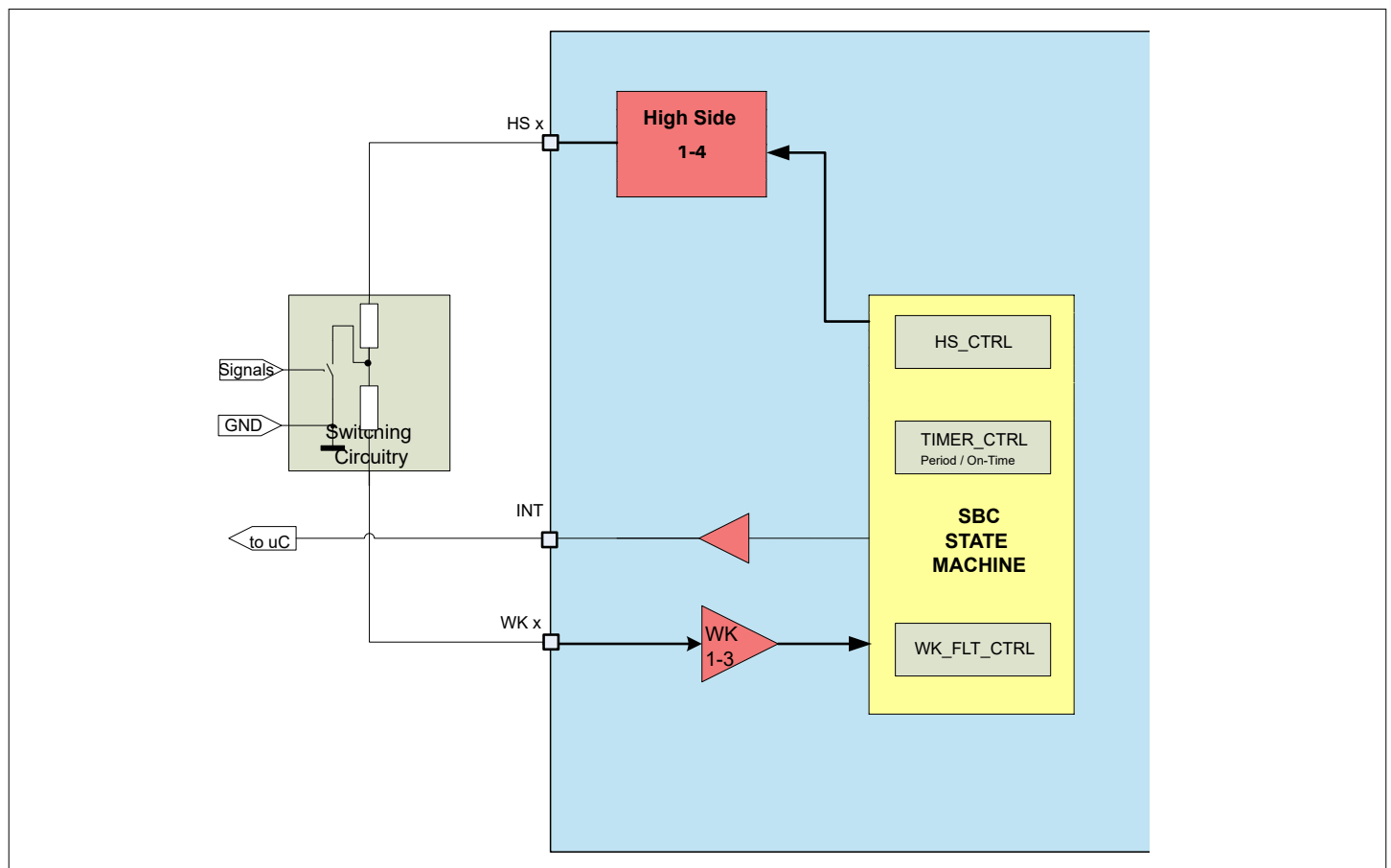
Figure 5 Cyclic Sense Working Principle
