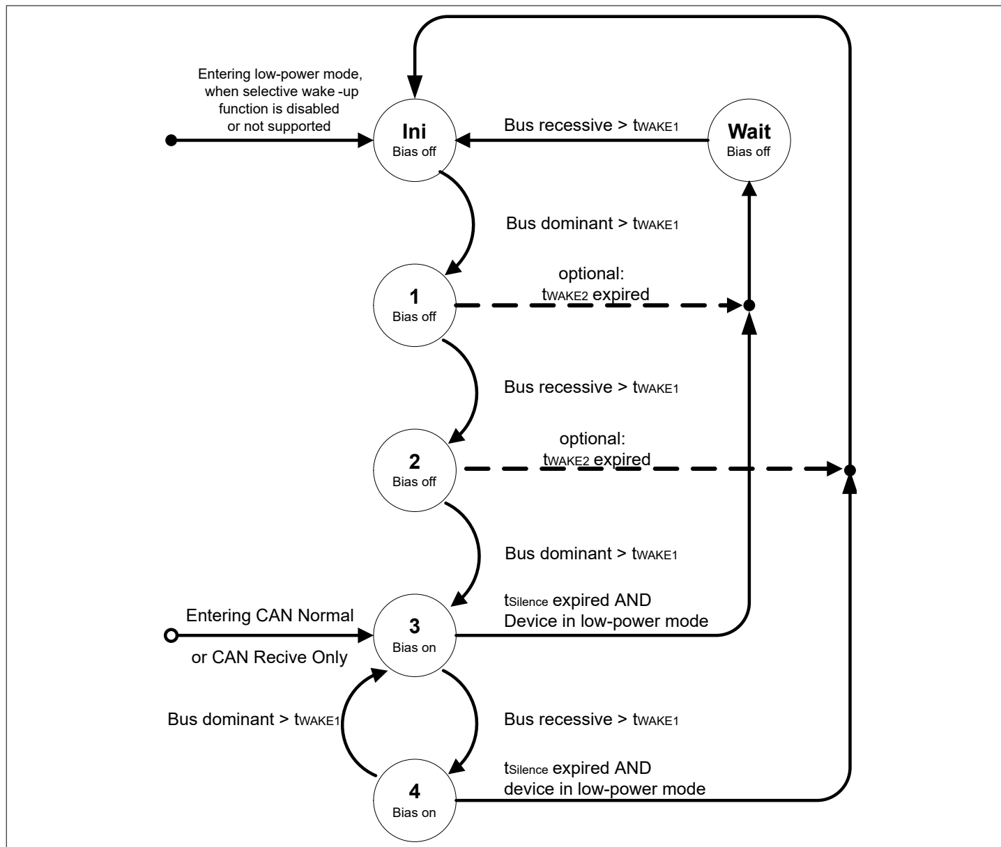
Figure 13 WUP detection following the definition in ISO 11898-2:2016
