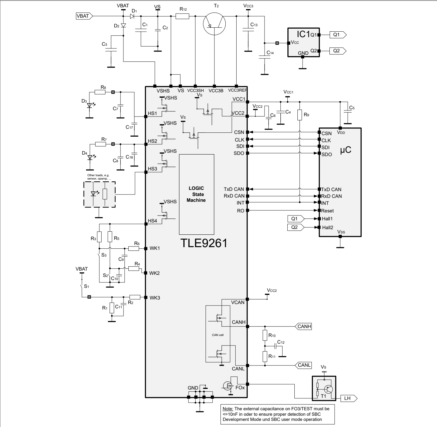
Figure 58 Simplified Application Diagram
