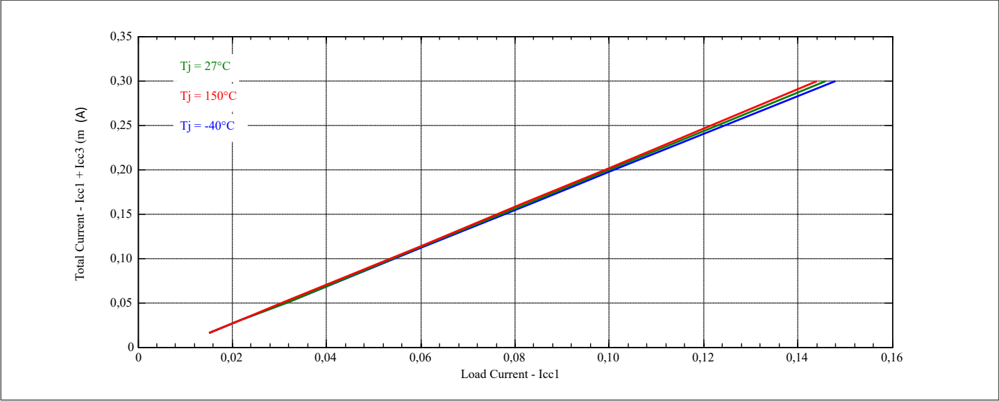
Figure 28 Load Sharing Behavior of ICC1 vs. the total load current
