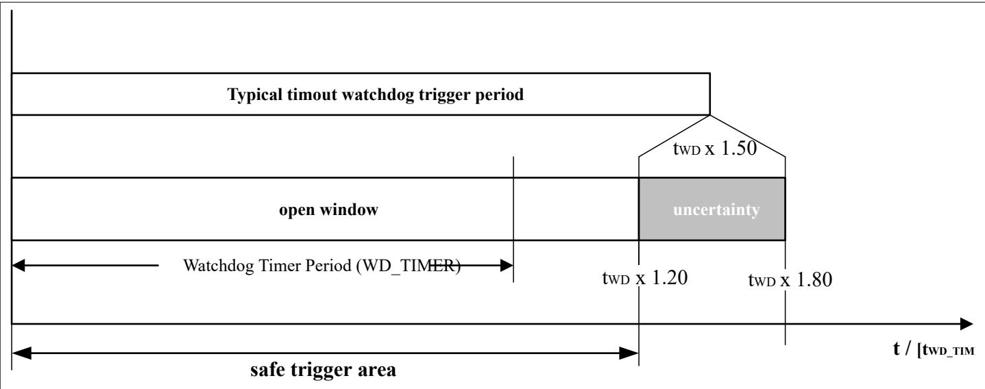
Figure 47 Time-out Watchdog Definition
