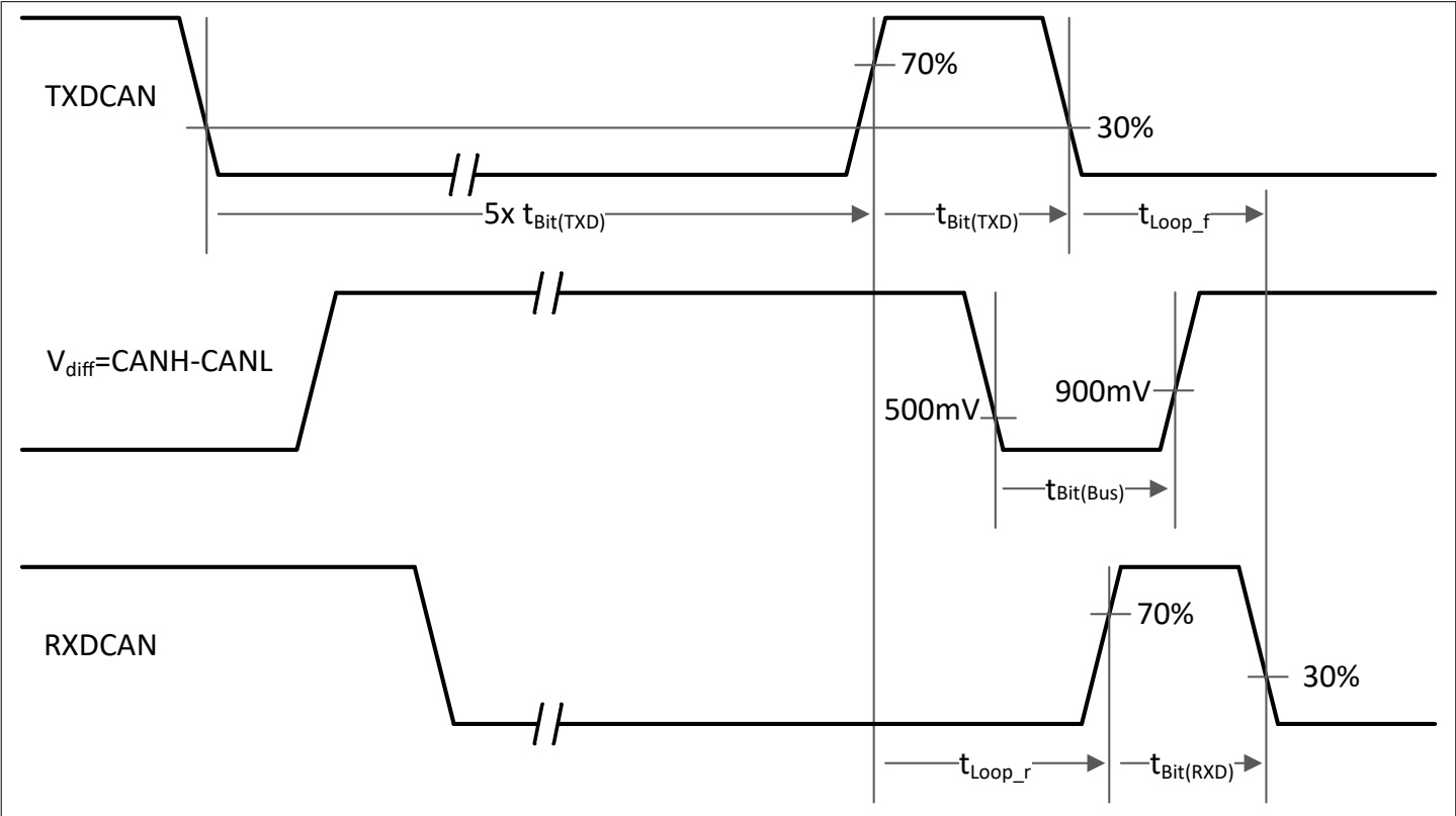
Figure 36 From ISO 11898-2: t_{loop} , t_{bit(TXD)} , t_{bit(Bus)} , t_{bit(RXD)} definitions
