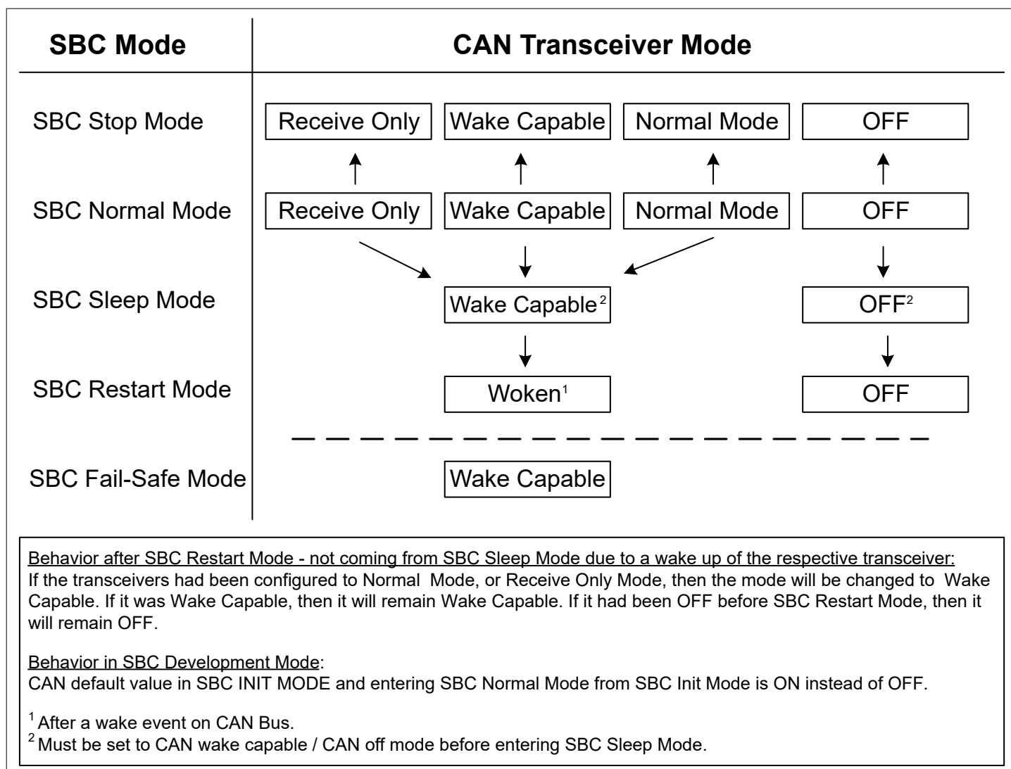
Figure 31 CAN Mode Control Diagram
