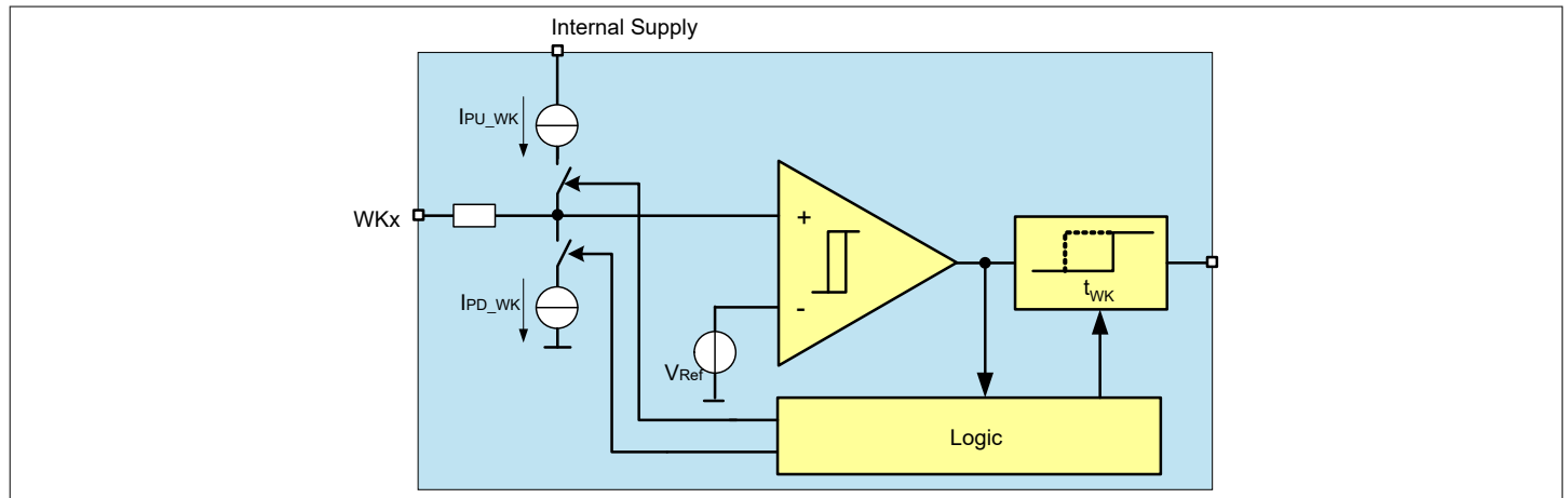
Figure 37 Wake Input Block Diagram
