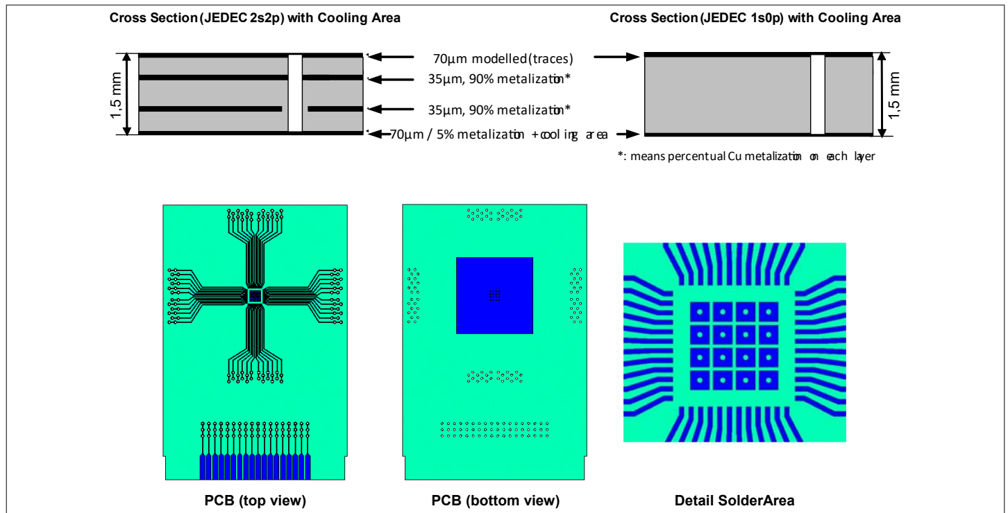
Figure 62 Board Setup
