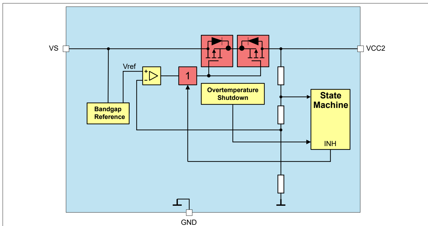
Figure 19 Module Block Diagram
