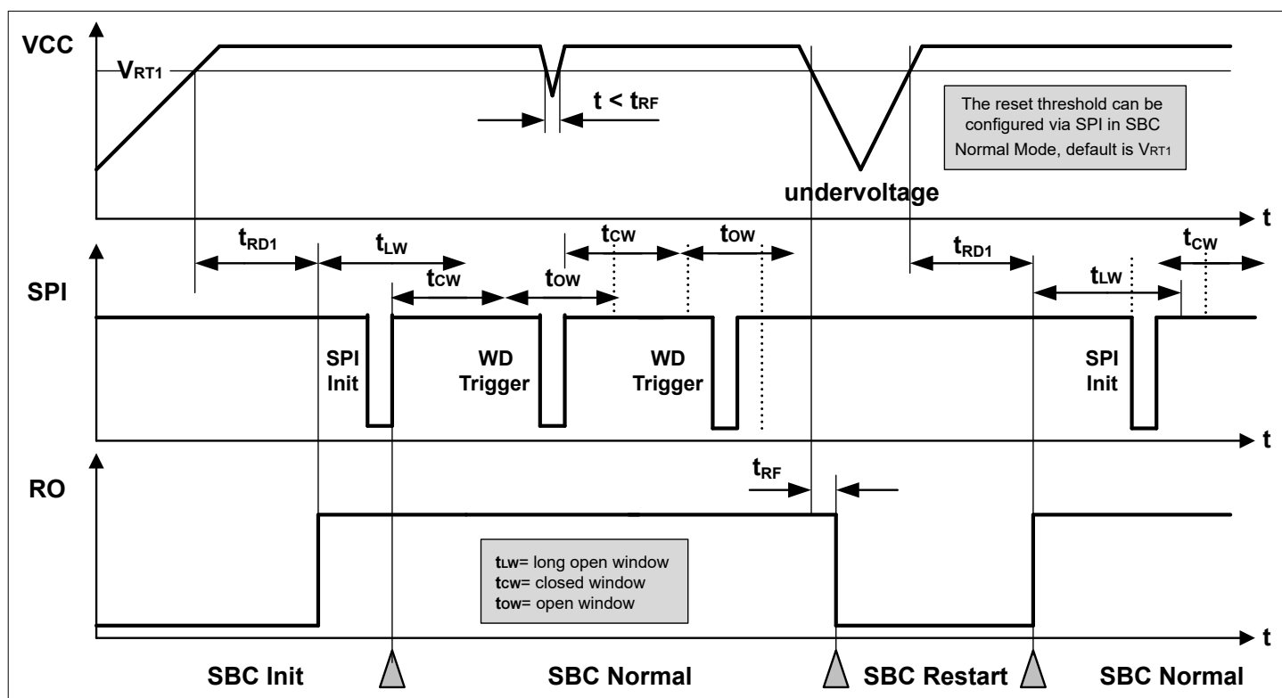
Figure 46 Reset Timing Diagram
