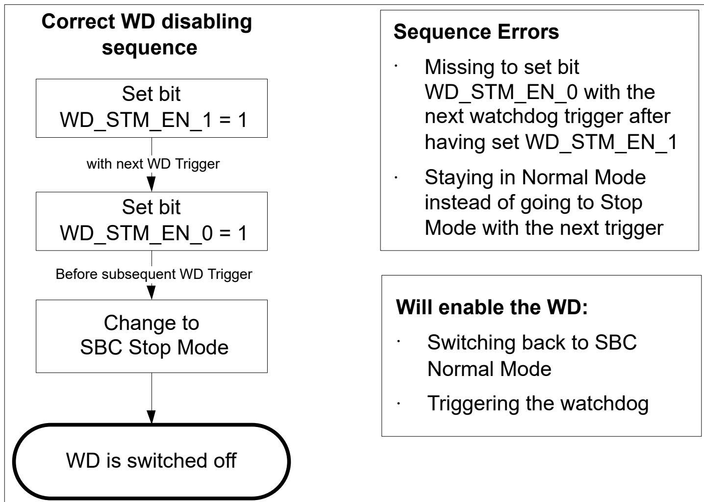
Figure 49 Watchdog disabling sequence in SBC Stop Mode
