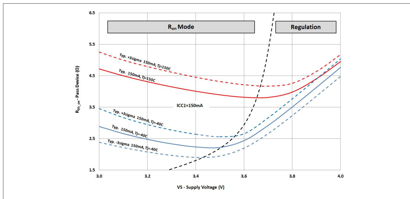
Figure 18 Characterization results of on-resistance range of VCC1 pass device during low drop operation for I_{CC1} = 150\text{mA}
