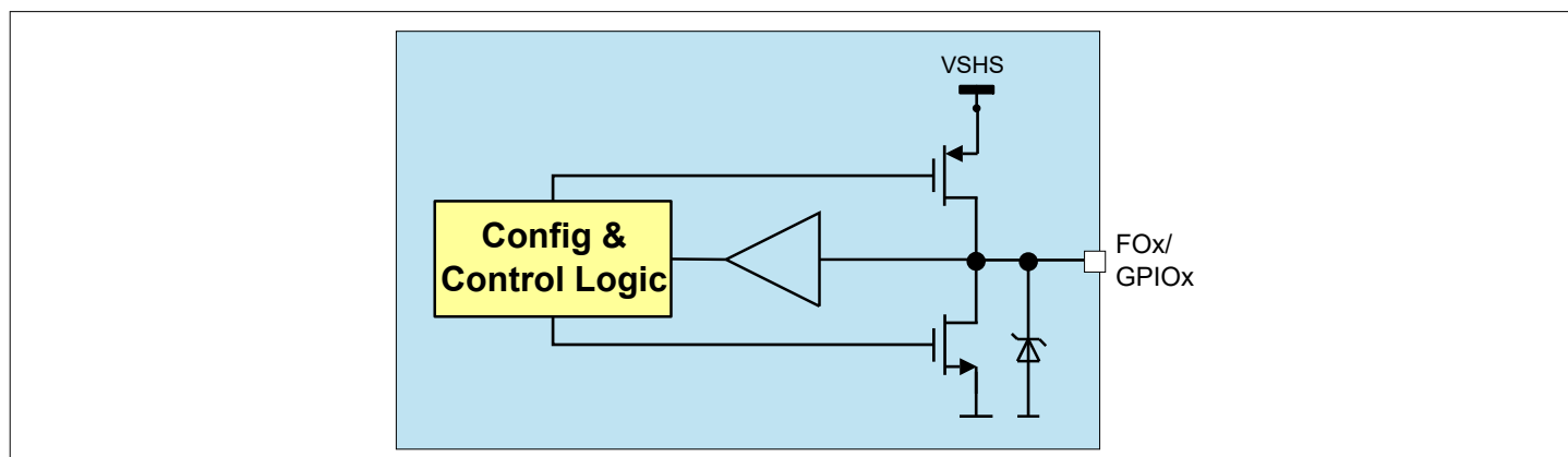
Figure 44 Simplified General Purpose I/O block diagram for FO2 and FO3/TEST
