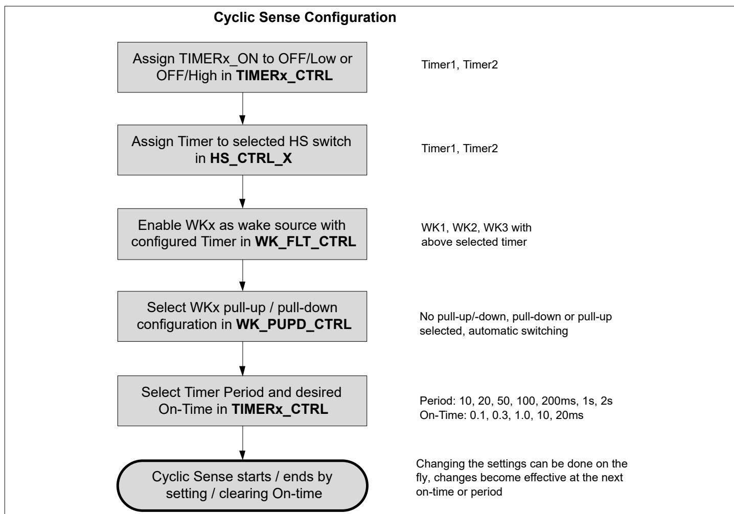
Figure 6 Cyclic Sense: Configuration and Sequence
