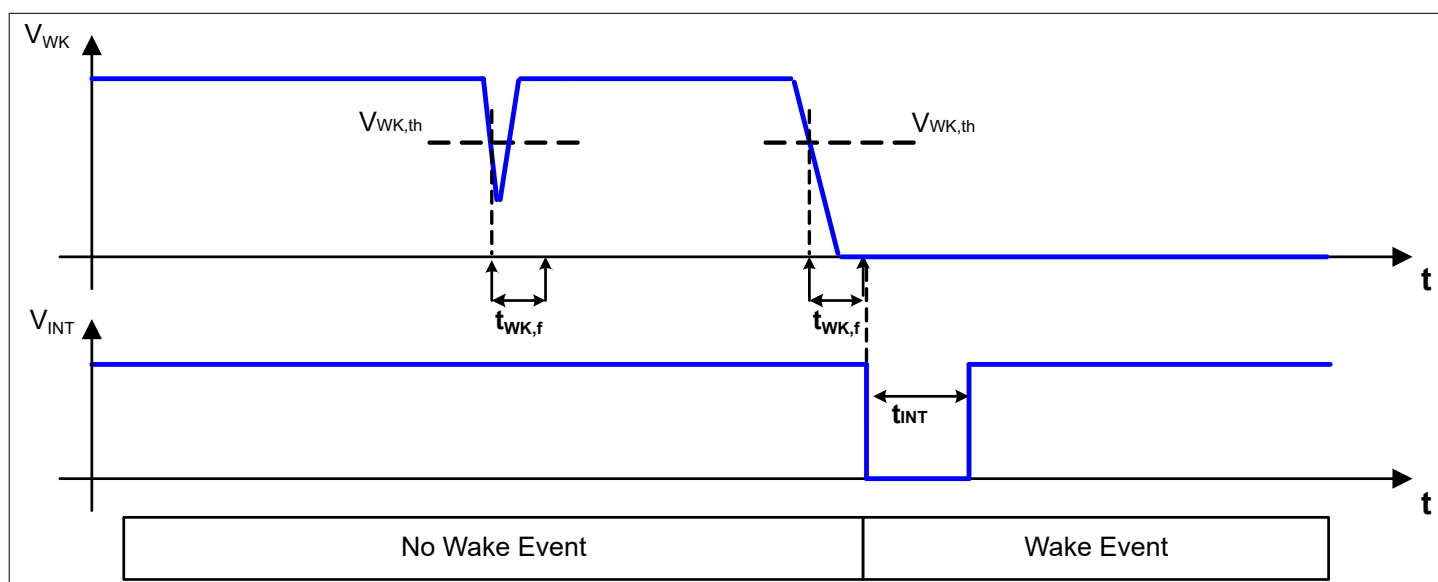
Figure 38 Wake-up Filter Timing for Static Sense
