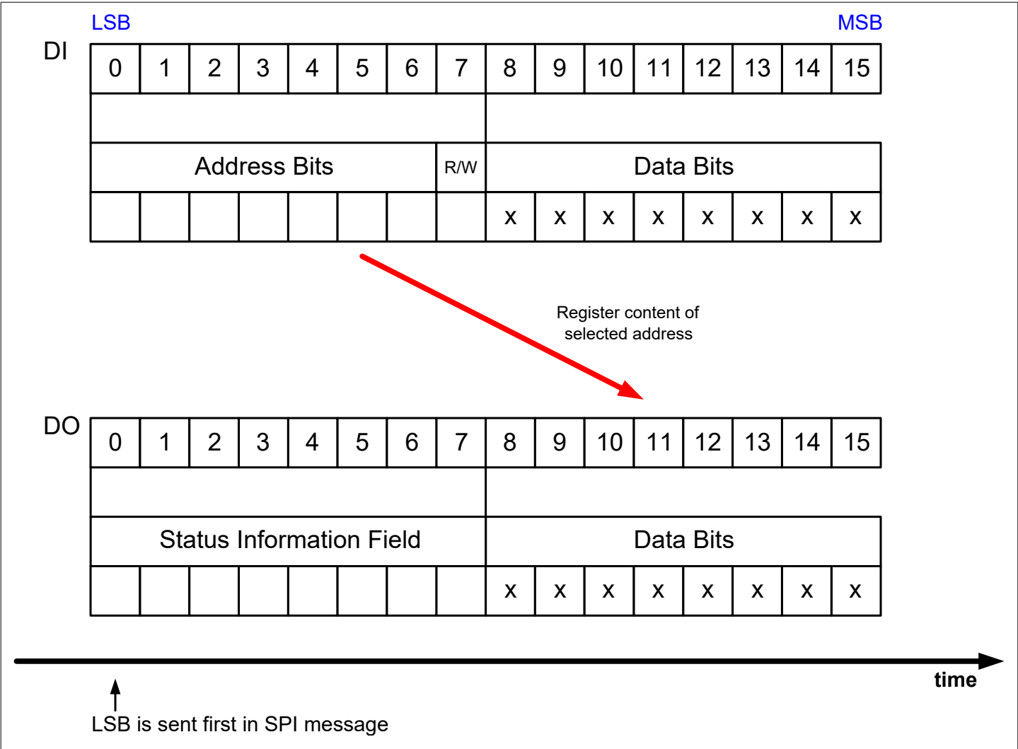
Figure 54 SPI Operation Mode
