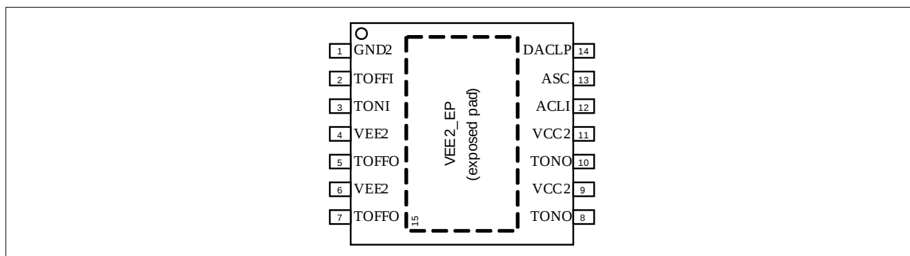
Figure 2-1 Pin Configuration
