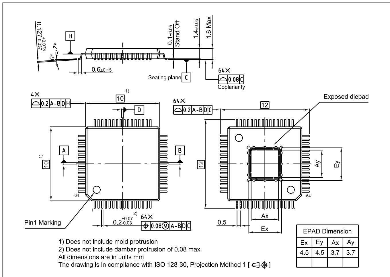
Figure 39 PG-LQFP-64
