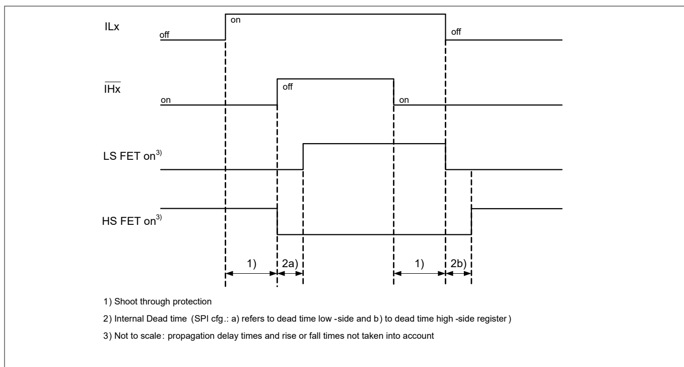
Figure 12 Shoot Through Protection and Dead Time Generation in Normal Operation Mode
