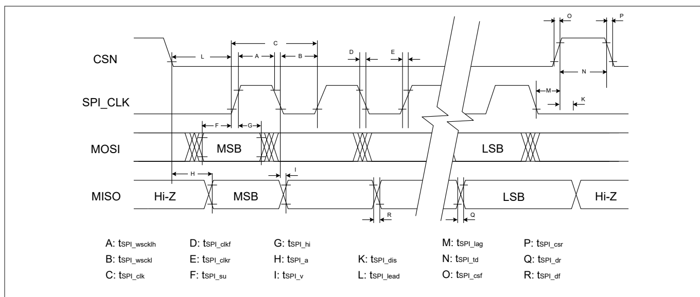
Figure 6 SPI Timing Parameters
