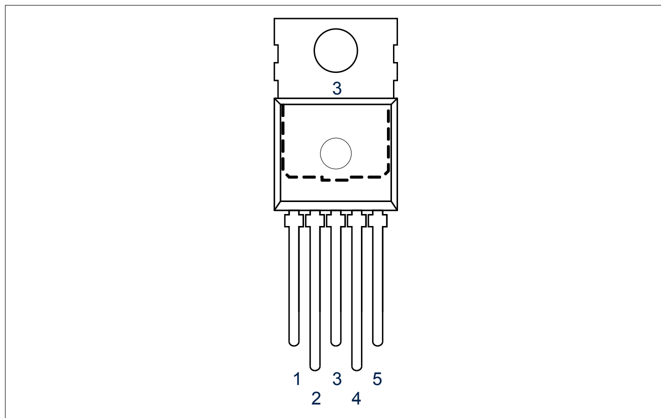
Figure 2 Pin configuration for PG-TO-220-5-12 Straight Leads
