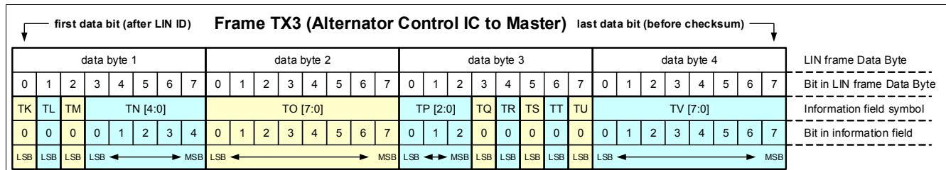
Figure 19 Frame TX3
