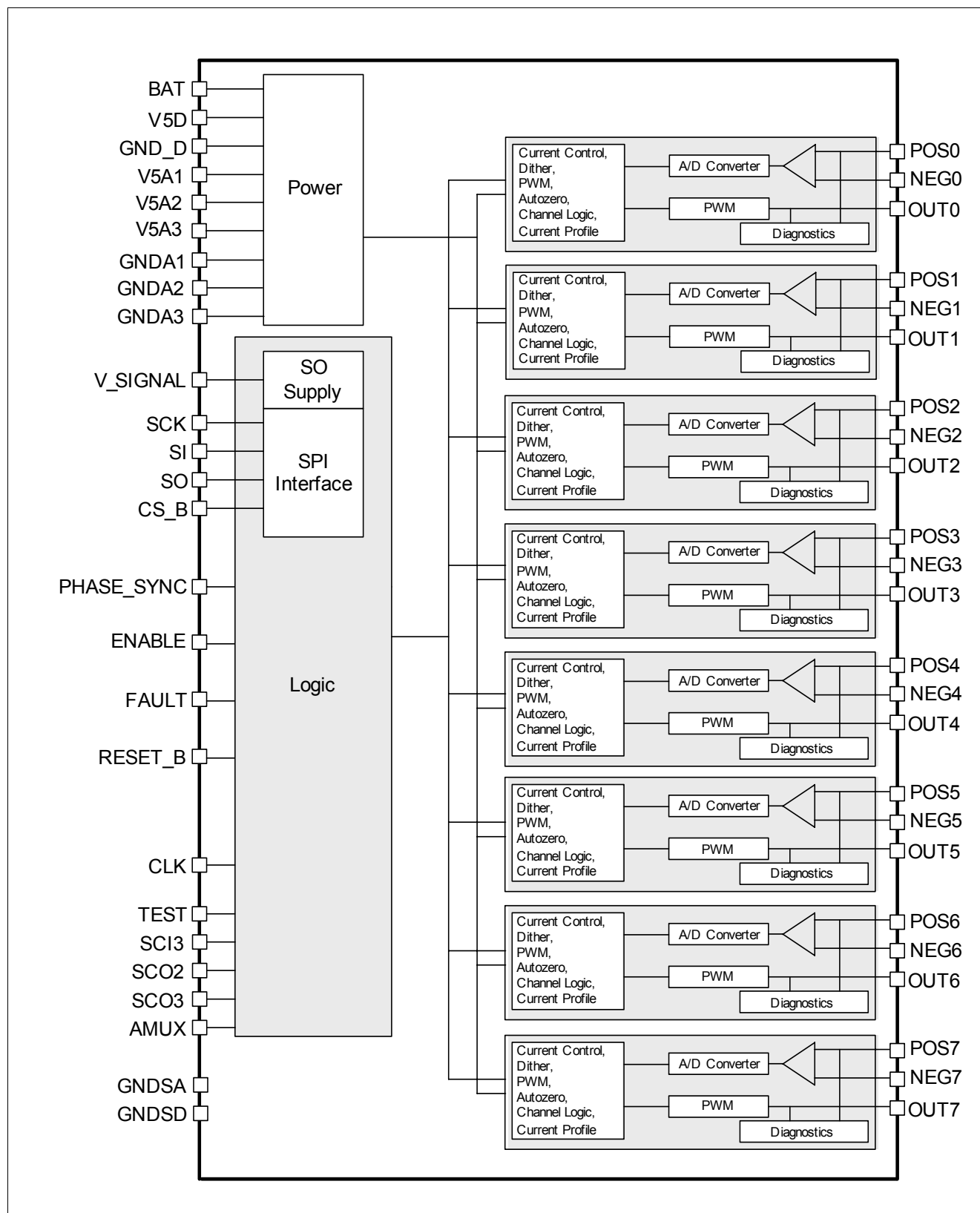
Figure 5 Block Diagram
