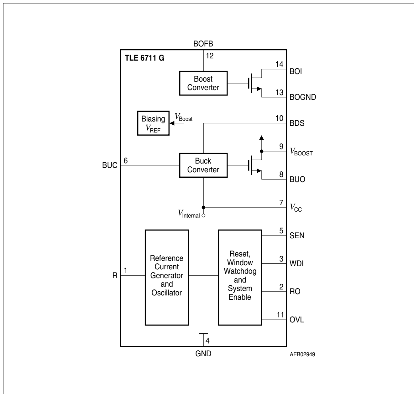
Figure 1 Block Diagram (pinning valid for PG-DSO-14-1)
