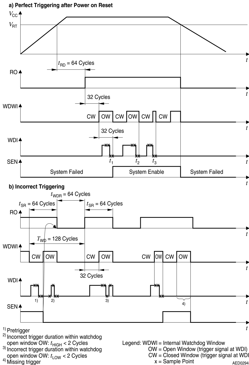
Figure 7 Window Watchdog Function
