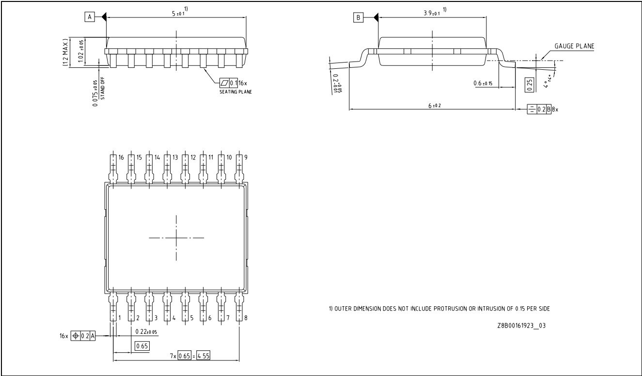
Figure 4-2 PG-TDSO-16 package dimension
