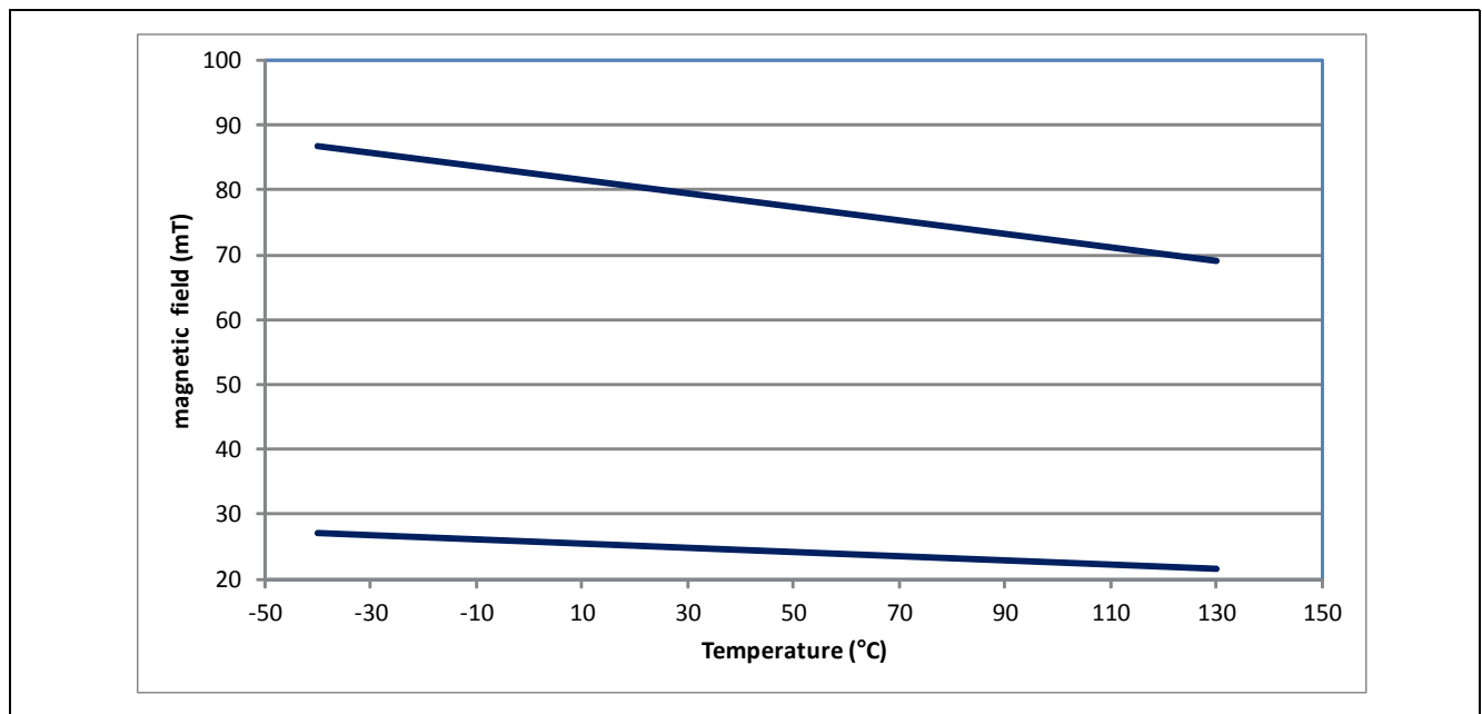
Figure 3-1 Allowed magnetic field range within ambient temperature range.
