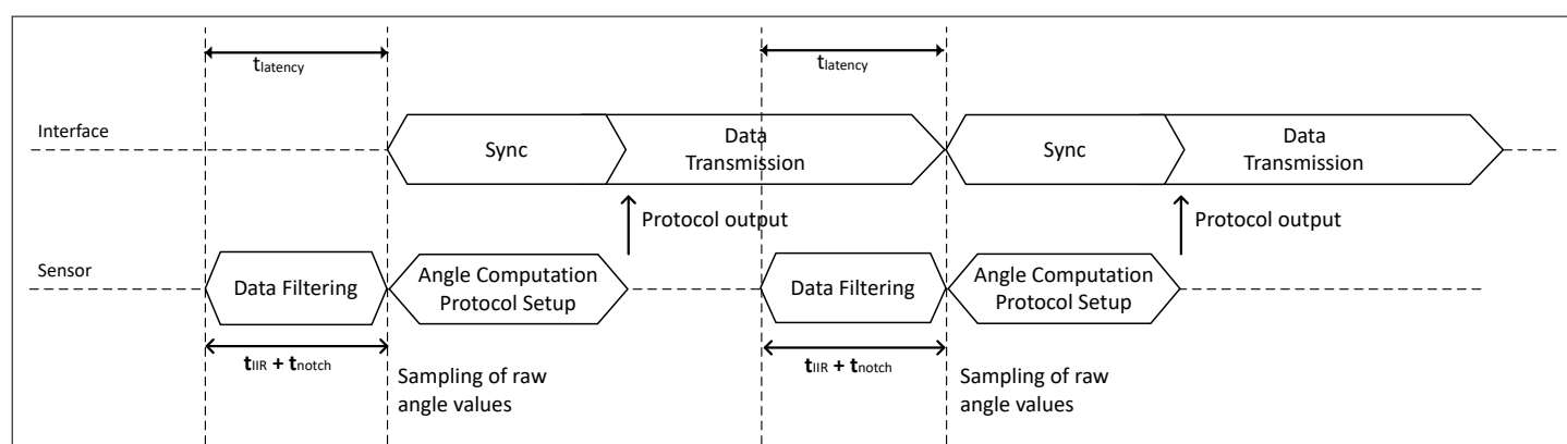
Figure 5 SENT interface timing overview
