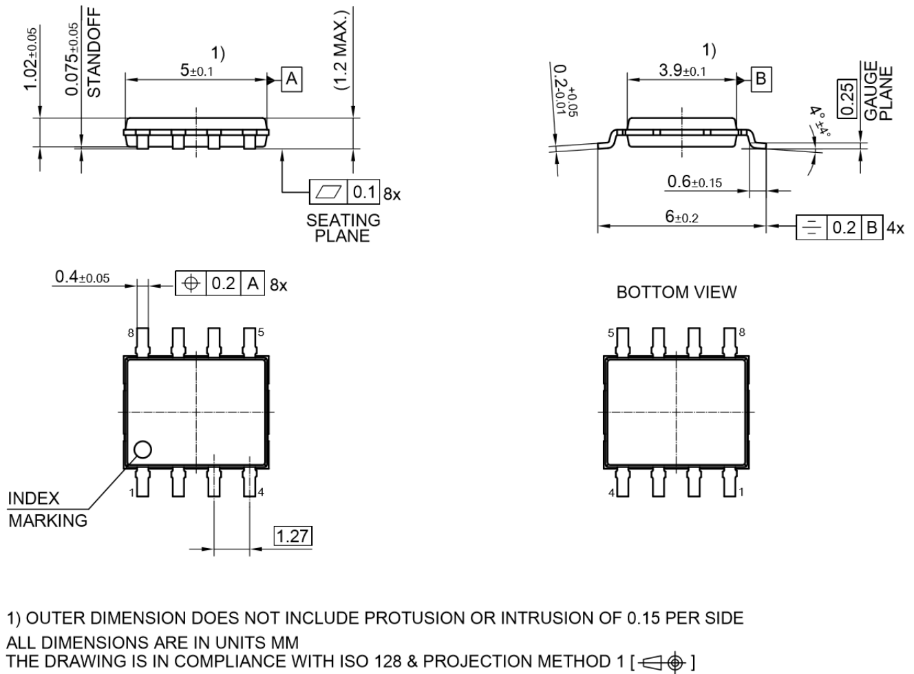
Figure 25 PG-TDSO-8-1 package drawing
