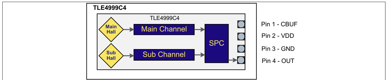
Figure 2 TLE4999C4-S0001 Package configuration
