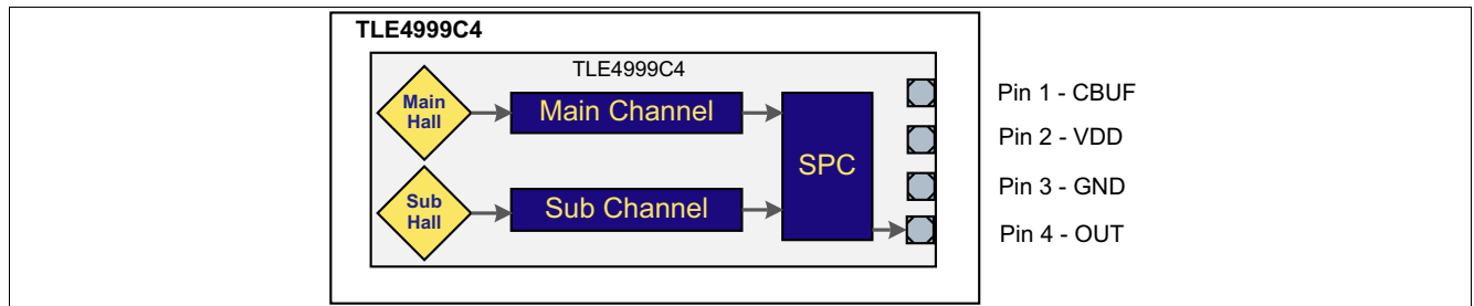
Figure 2 TLE4999C4 Package configuration
