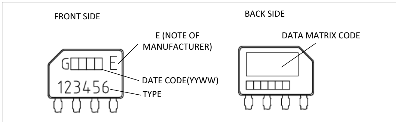
Figure 11 PG-SSO (Plastic Green Single Small Outline), package marking
