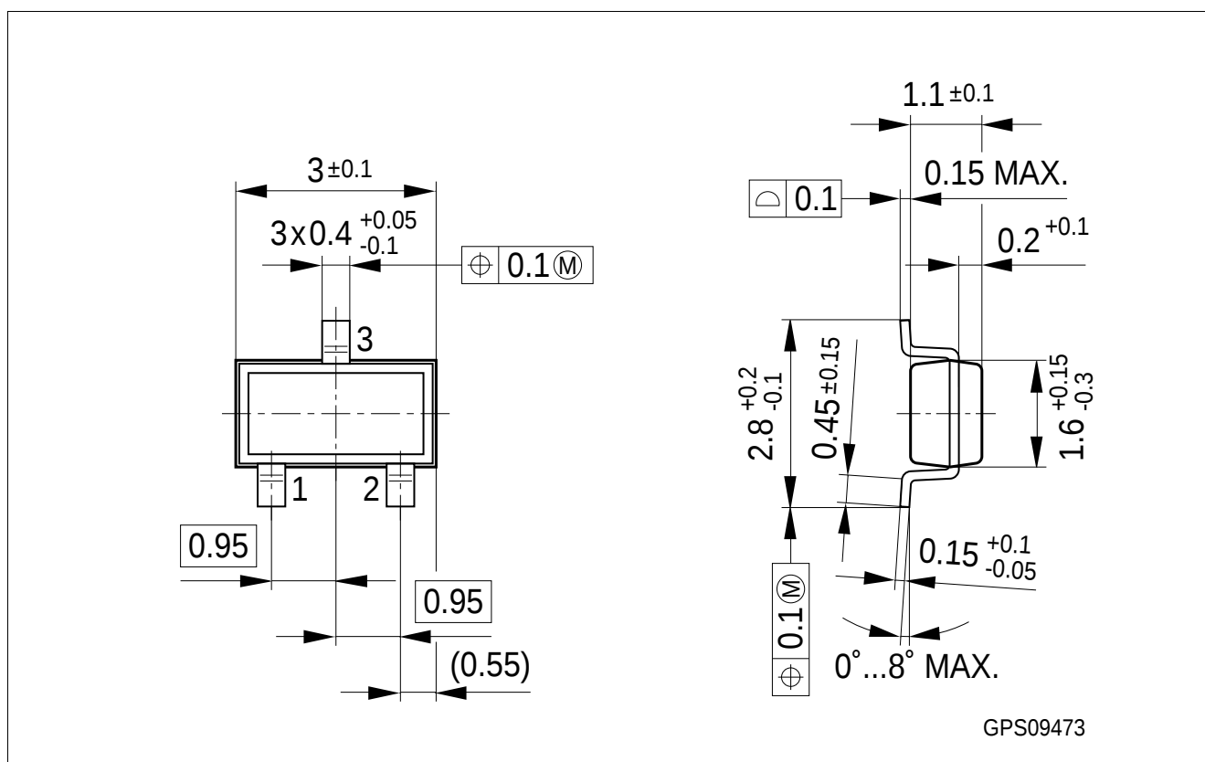
Figure 7 SC59 Package Outline (All dimensions in mm)
