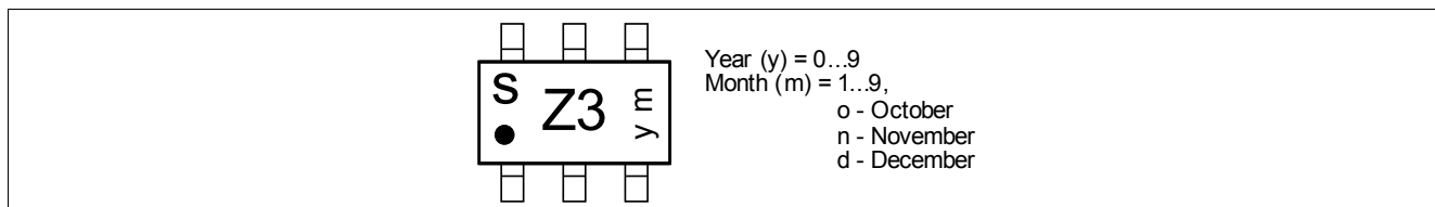
Figure 7 Marking PG-TSOP-6-6-5
