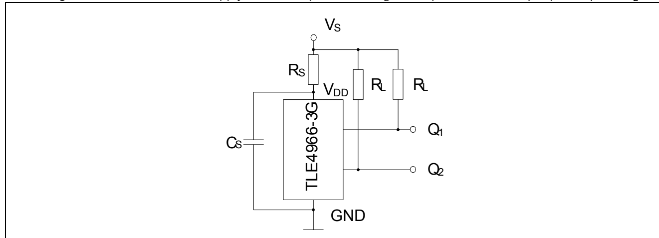
Figure 3 Application Circuit
