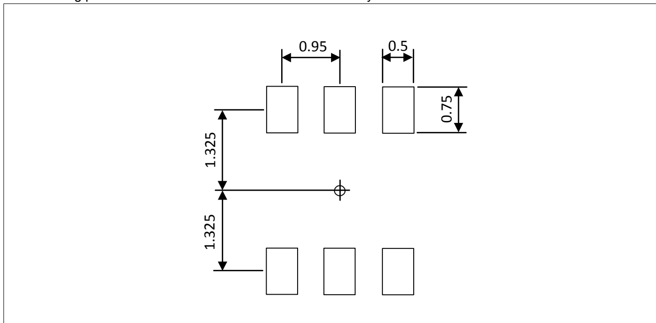
Figure 8 Footprint PG-TSOP6-6-9
