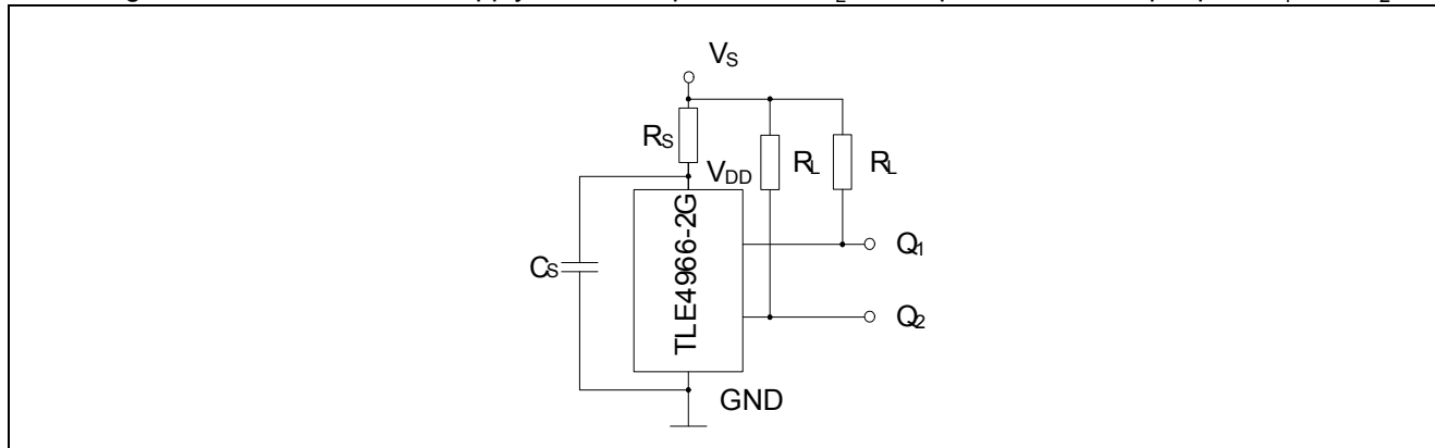
Figure 3 Application Circuit
