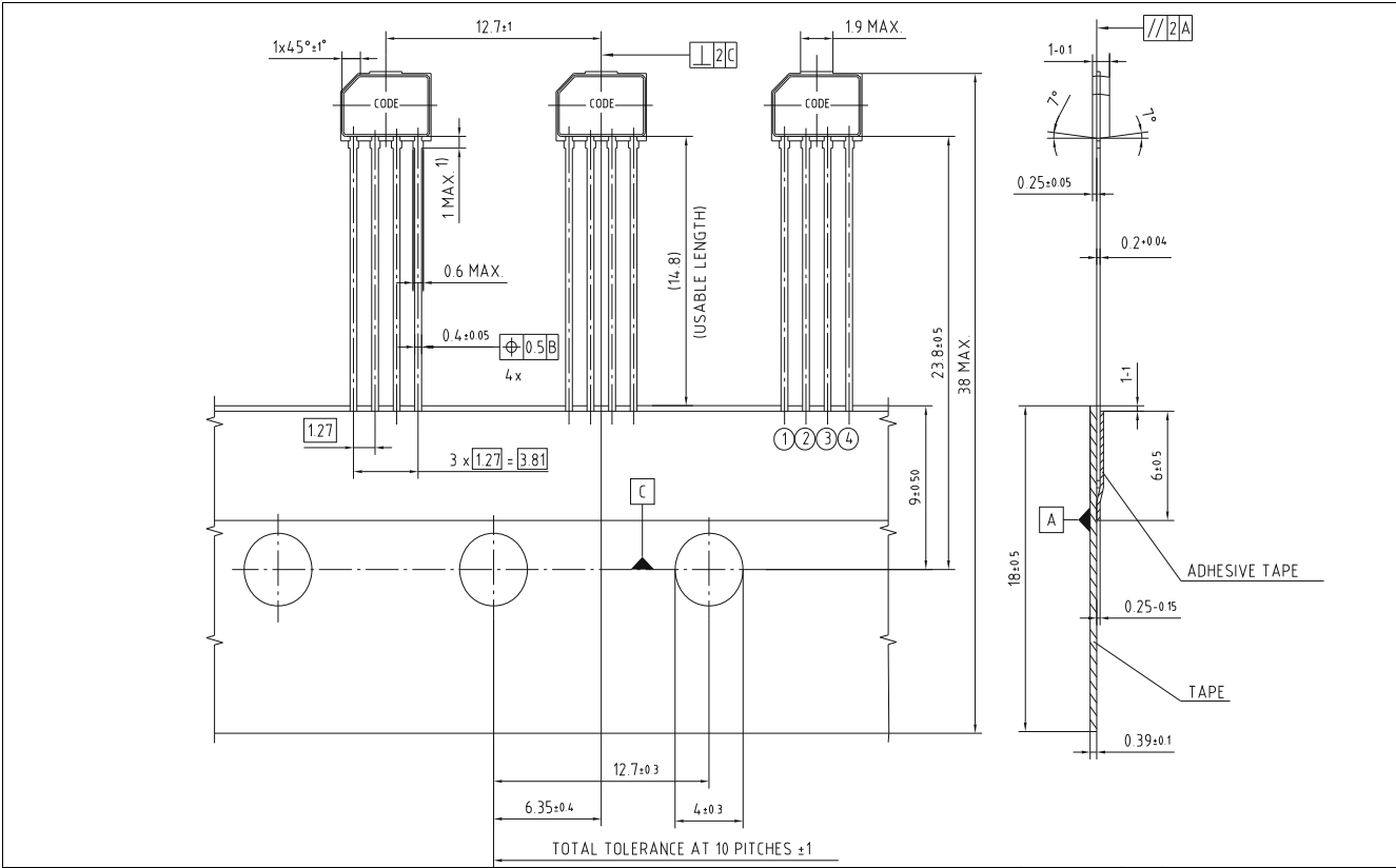
Figure 8 PG-SSO-4-1 Ammopack
