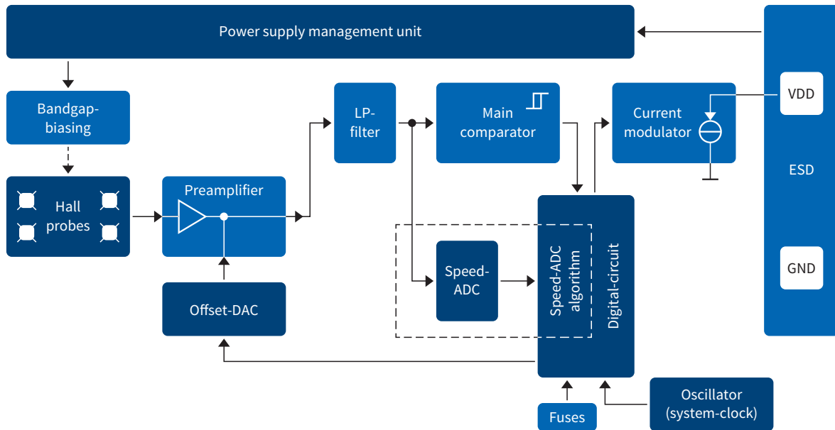
TLE4941plusC block diagram
