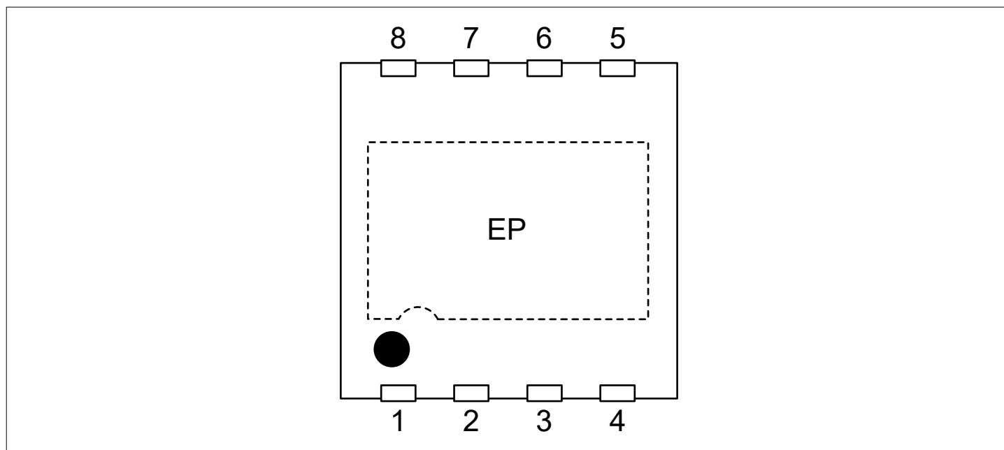
Figure 2 Sensor pinout
