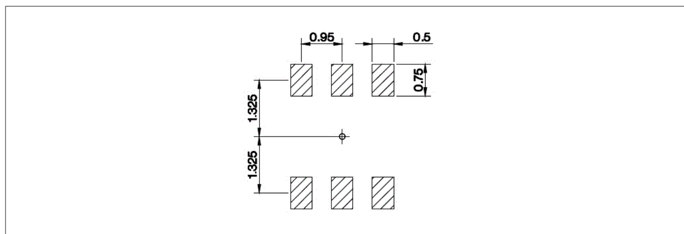
Figure 10 Footprint PG-TSOP6-6-8 (compatible to PG-TSOP6-6-5, all dimensions in mm)
