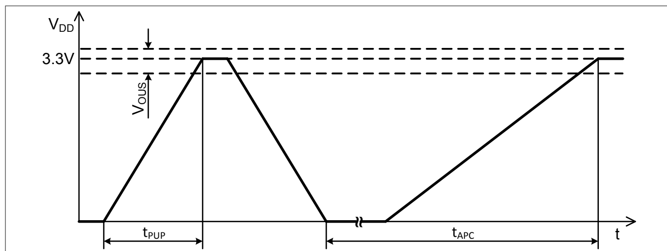
Figure 6 V_{DD} power up and power cycle for high availability
