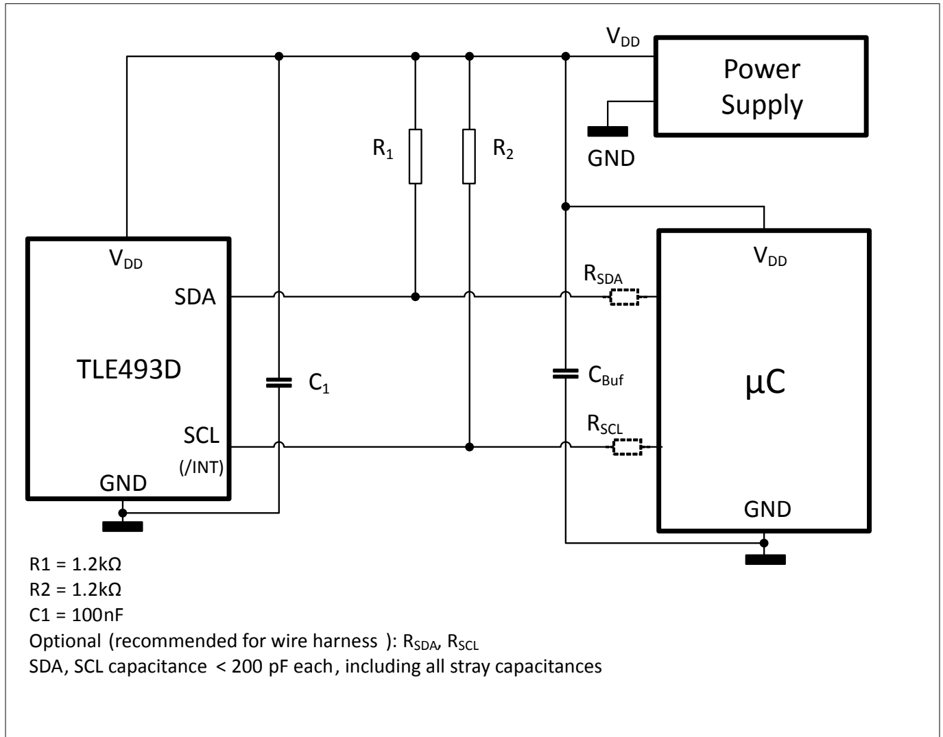
Figure 5 Application circuit with external power supply and μC
