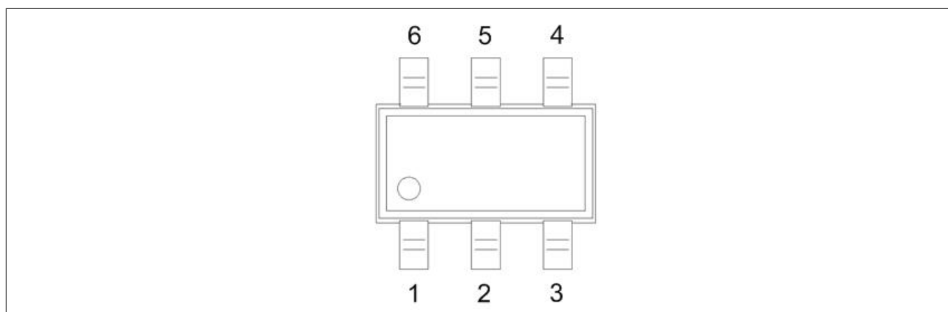
Figure 2 TLE493D-P2B6 pinout
