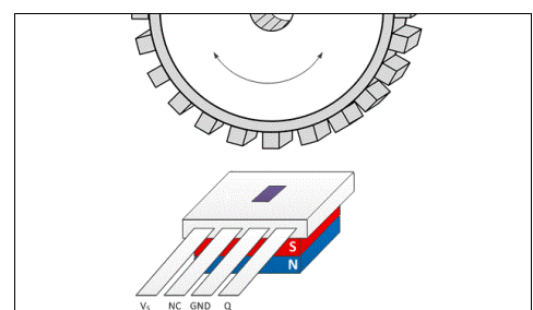
Figure 1-5 Wheel with sensor
