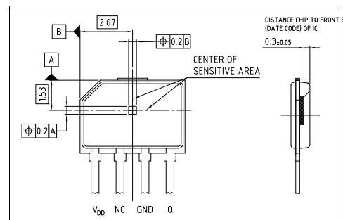
Figure 1-2 Pinning, Sensitive Area
