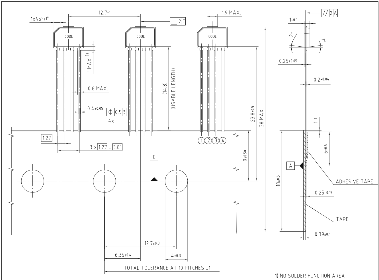
Figure 3-3 PG-SSO-4-1 packaging
