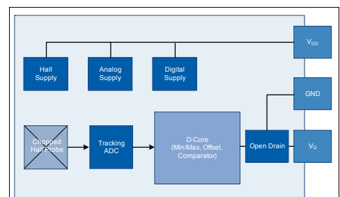
Figure 1-3 Blockdiagram TLE4922
