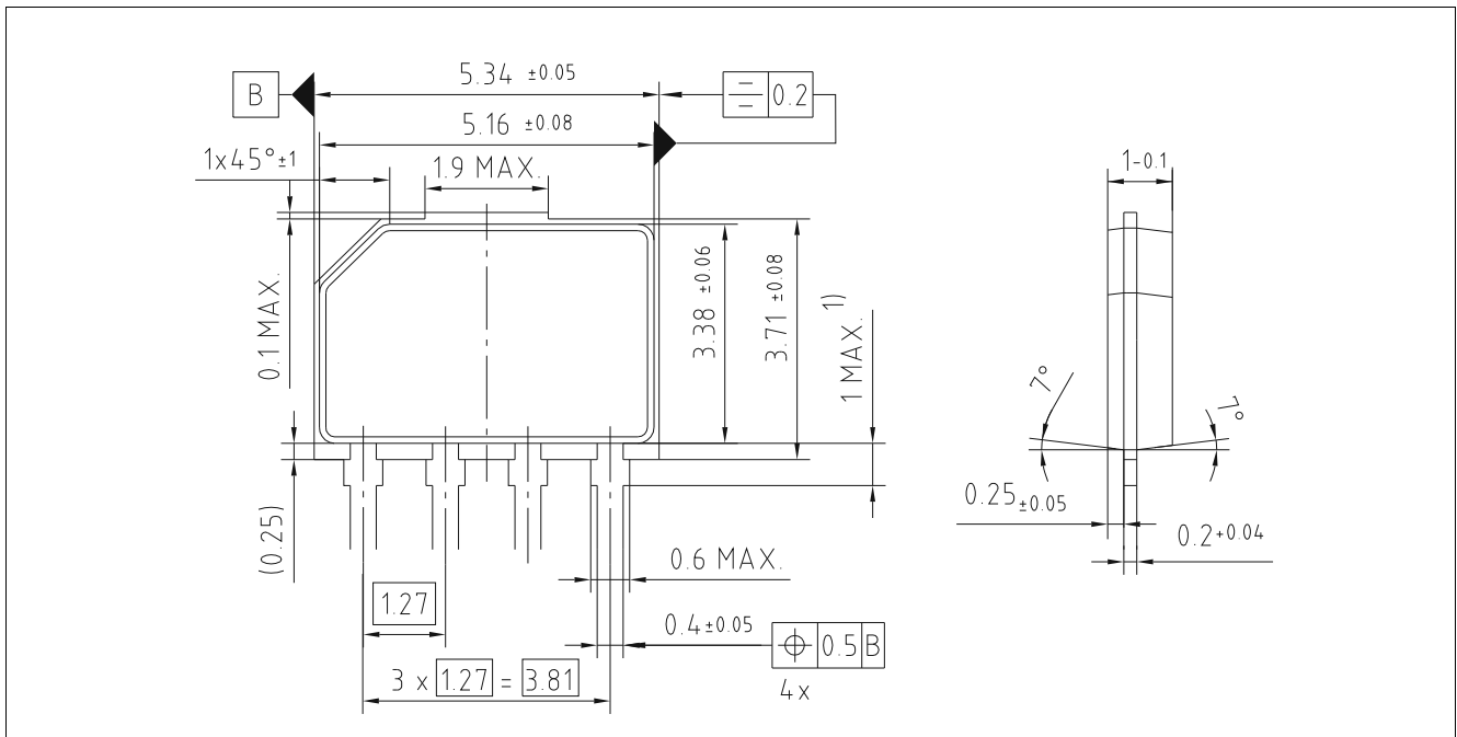
Figure 3-2 PG-SSO-4-1 package dimensions
