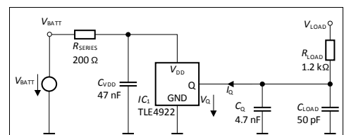
Figure 1-4 Application circuit TLE4922
