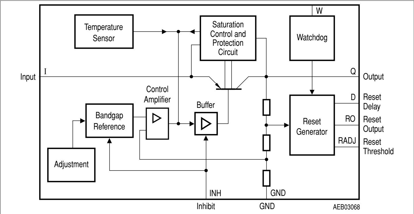
Figure 1 Block diagram
