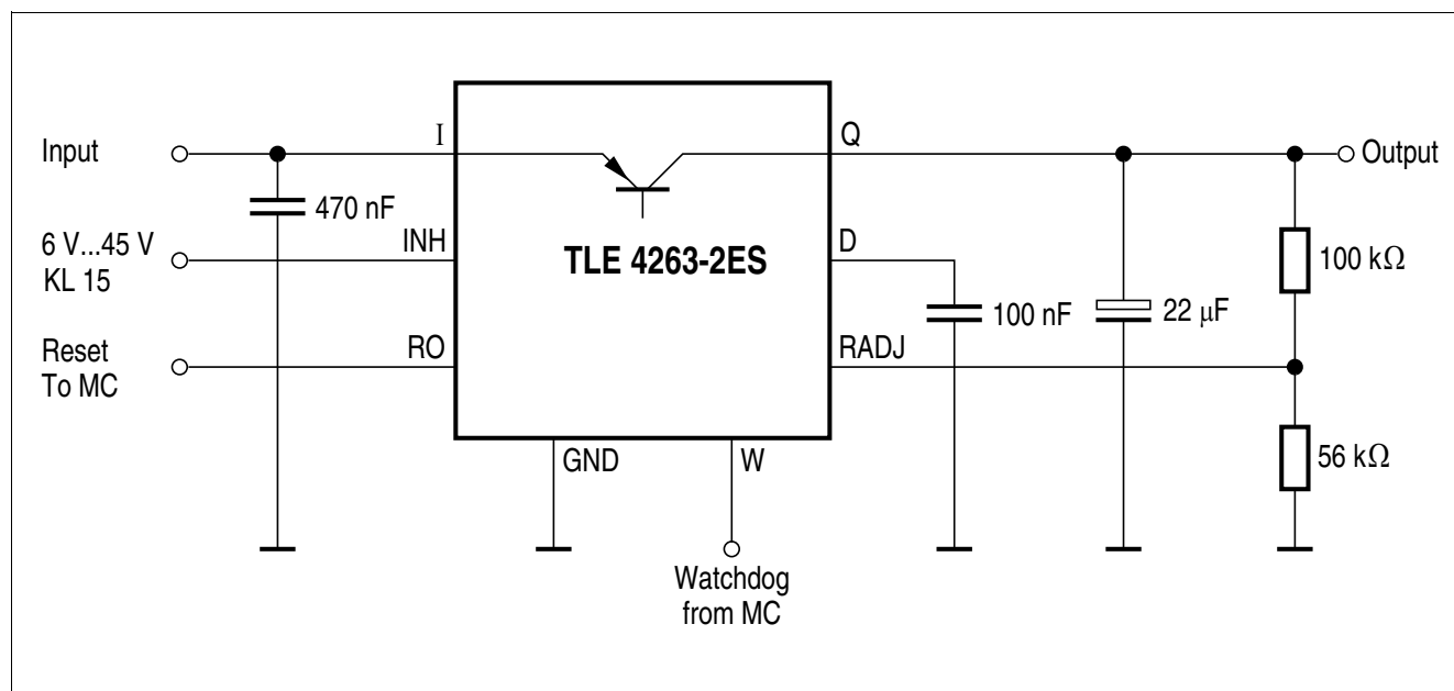
Figure 3 Application circuit
