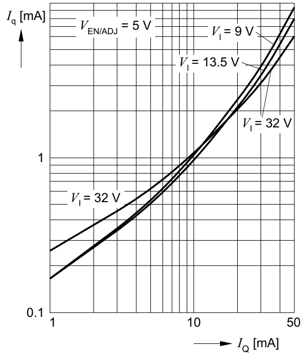
Current consumption I_{q2} vs. output current I_Q
