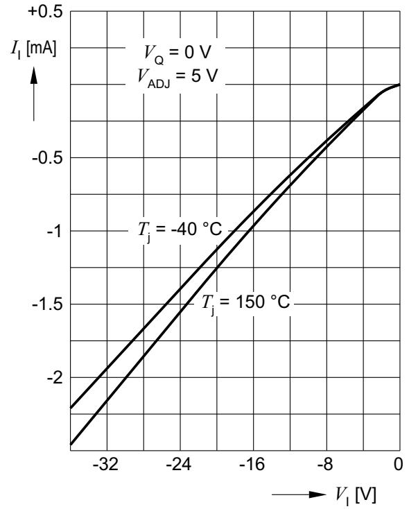
Reverse current I_I vs. input voltage V_I
