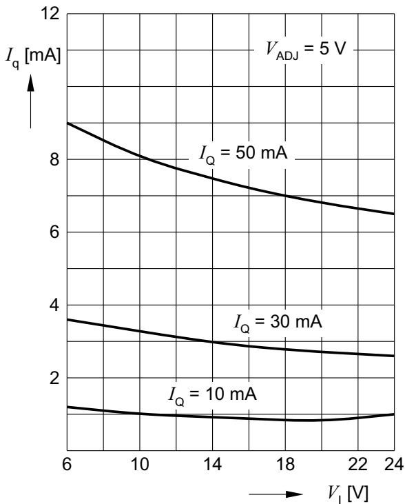
Current Consumption I_{q2} vs. input voltage V_i
