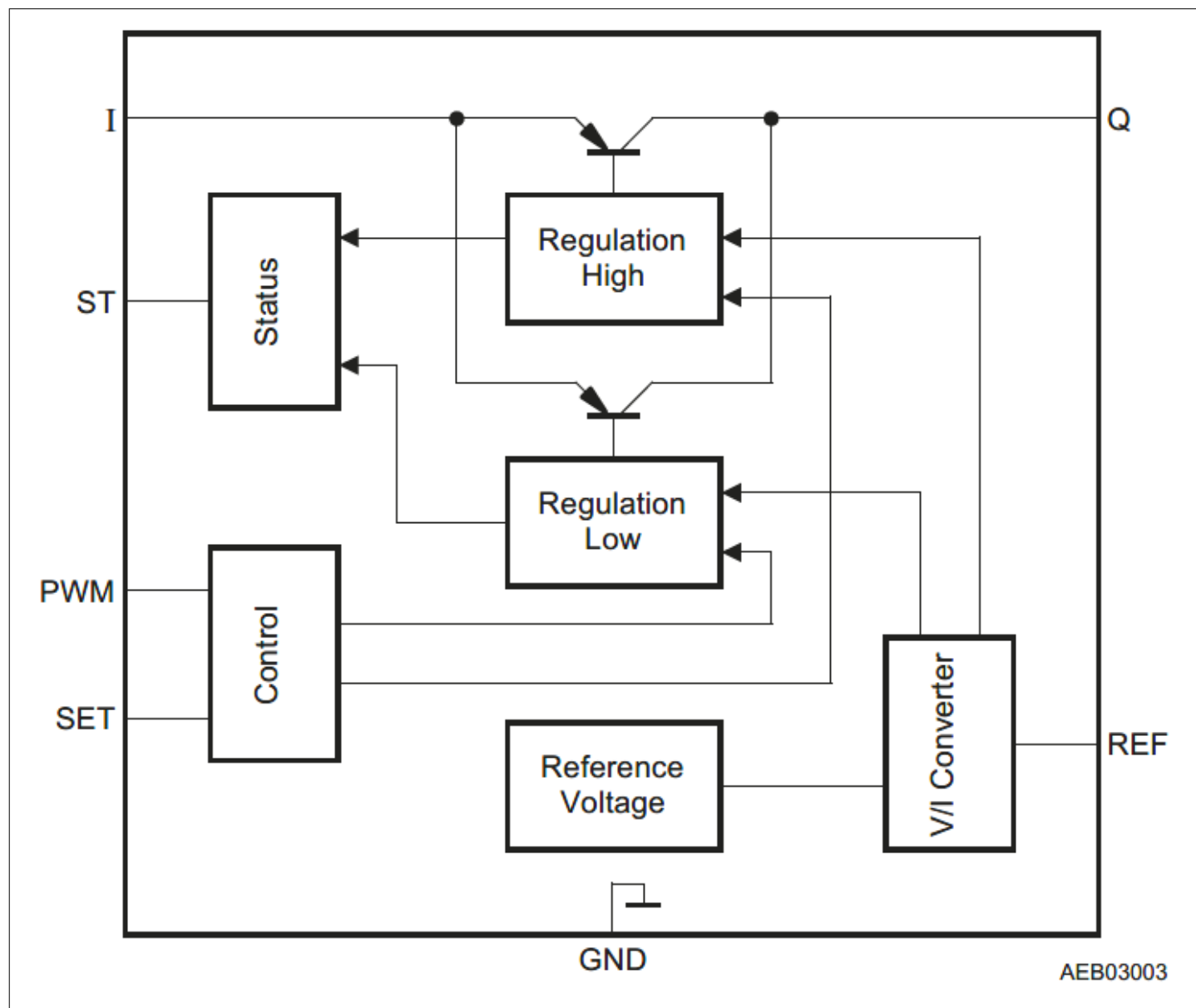
Figure 3 Block Diagram
