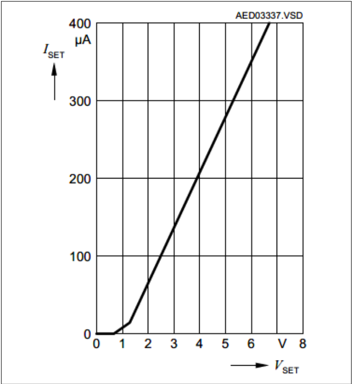
Figure 15 SET Pin Input Current versus SET Voltage
