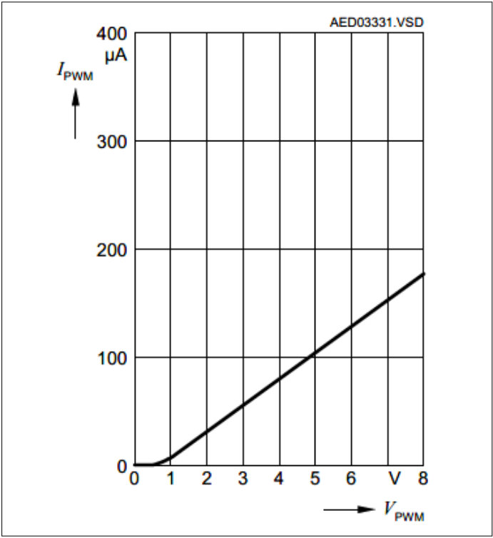
Figure 13 PWM Pin Input Current versus PWM Voltage
