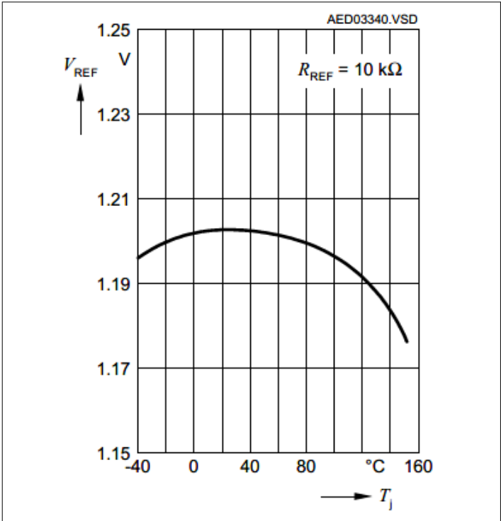
Figure 11 Reference Voltage versus Junction Temperature
