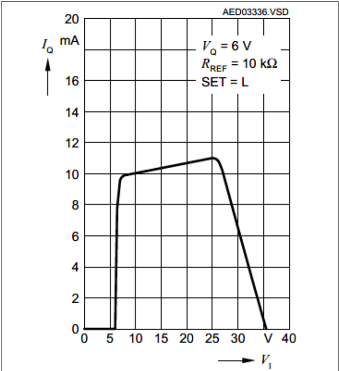
Figure 10 Output Current versus Supply Voltage, SET = L
