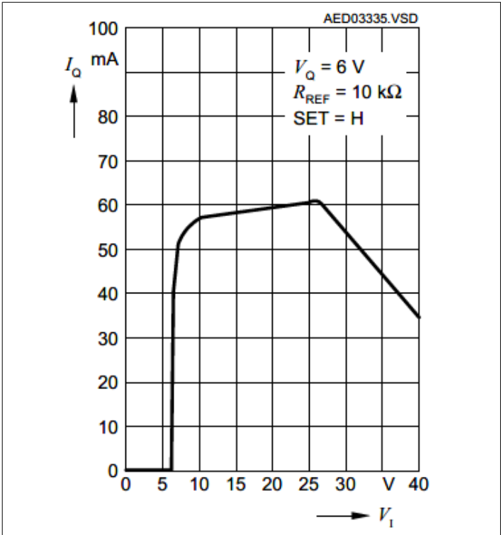
Figure 9 Output Current versus Supply Voltage, SET = H
