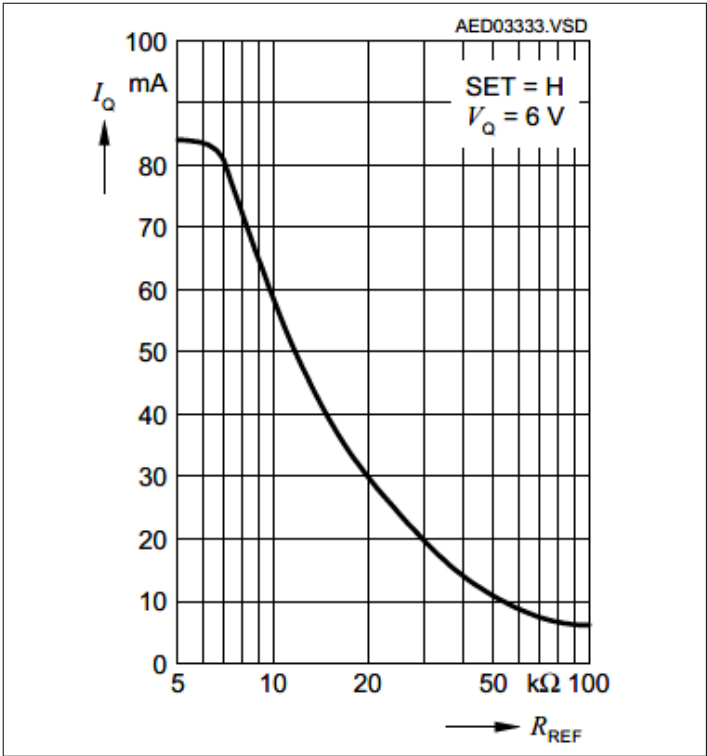
Figure 7 Output Current versus External Resistor, SET = H
