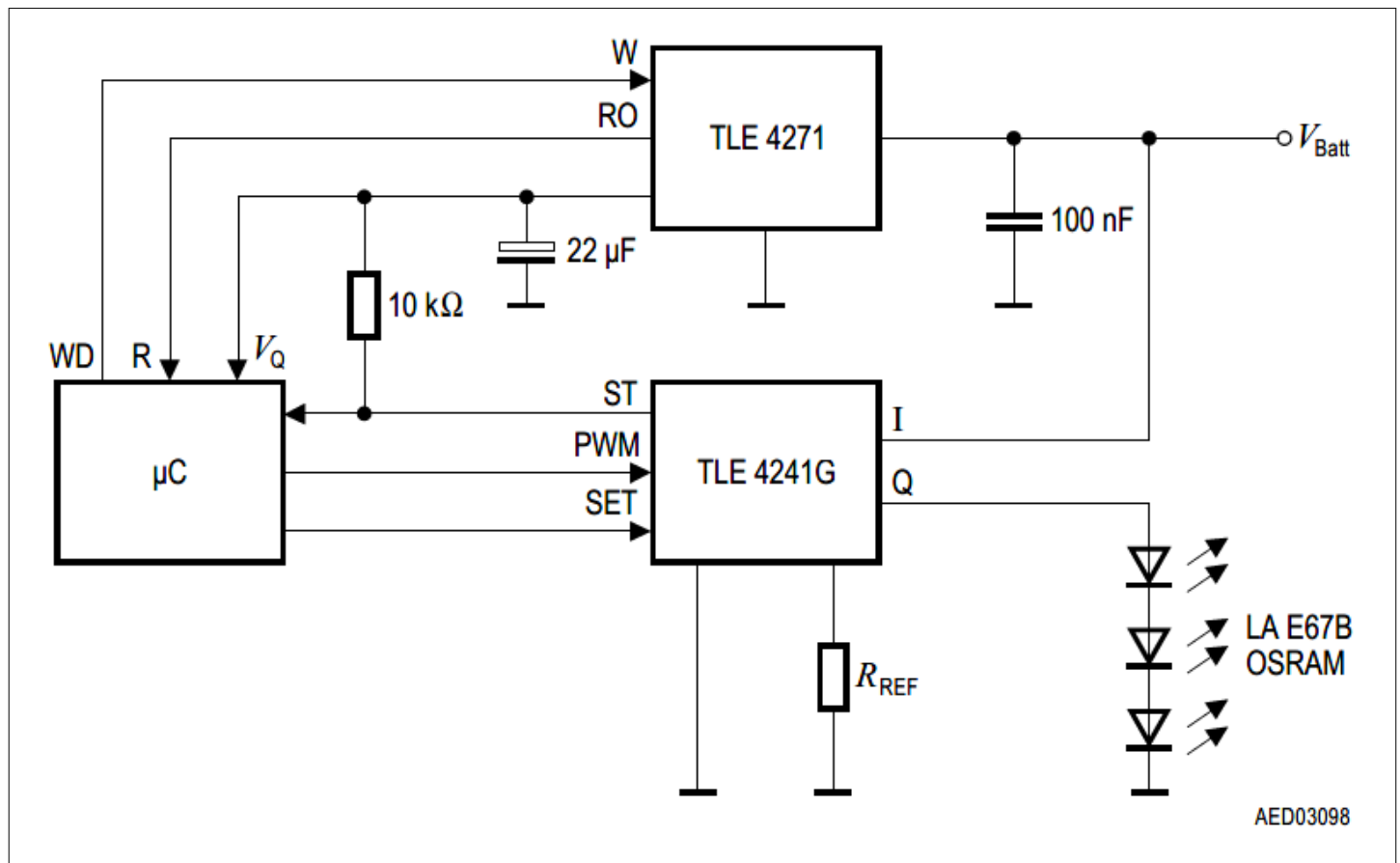
Figure 5 Application Circuit
