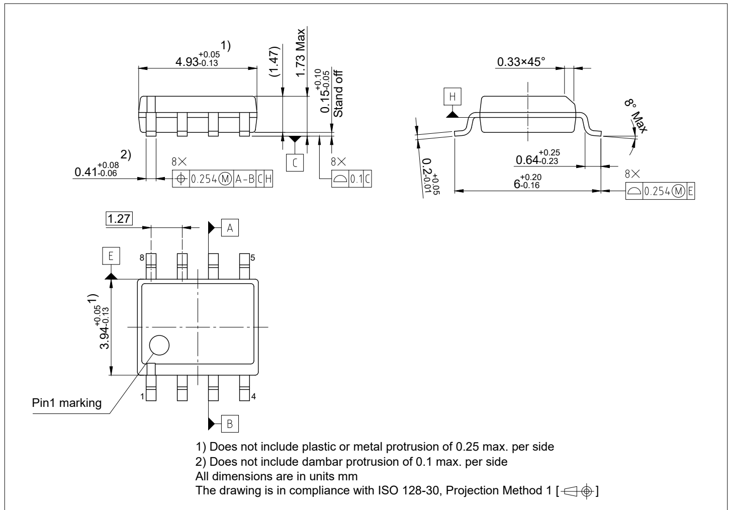
Figure 17 PG-DSO-8-62
