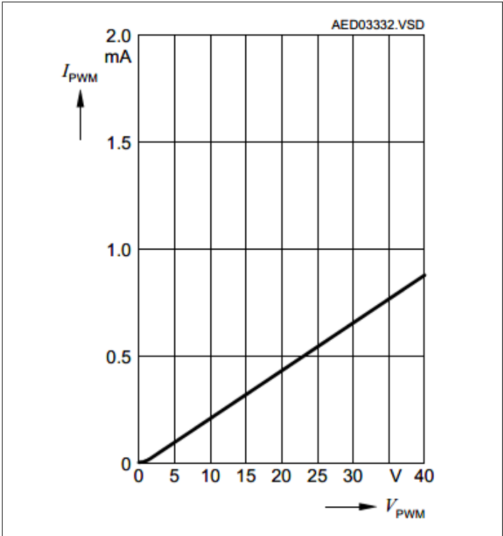
Figure 12 PWM Pin Input Current versus PWM Voltage
