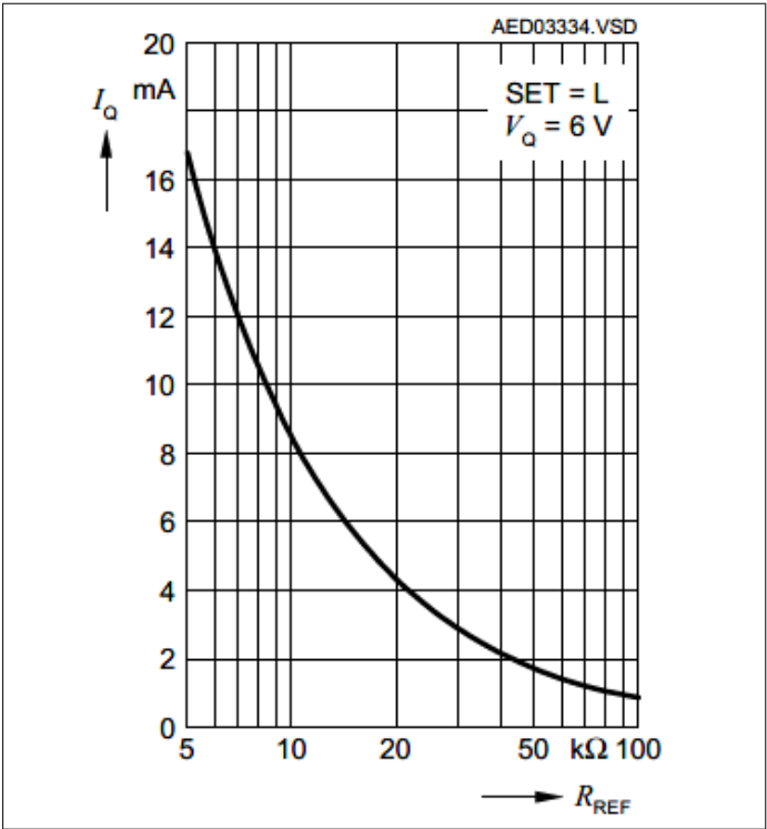
Figure 8 Output Current versus External Resistor, SET = L
