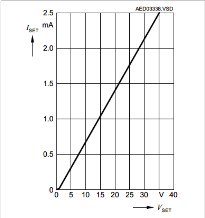
Figure 14 SET Pin Input Current versus SET Voltage
