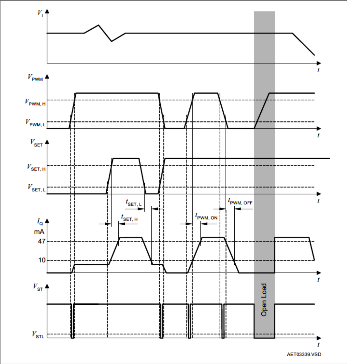
Figure 6 Function and Timing Diagram
