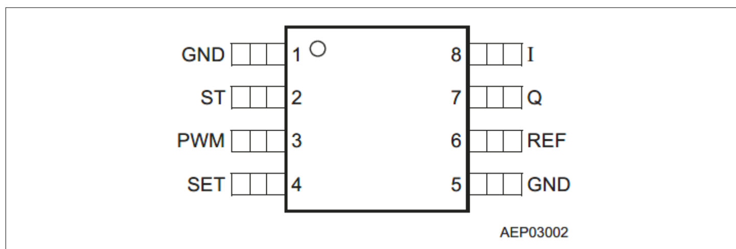
Figure 4 Pin Configuration (top view)
